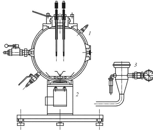
Figure 1: Standard 20-liter explosion sphere: 1 — explosion sphere, 2 — fast acting valve, and 3 — storage canister
