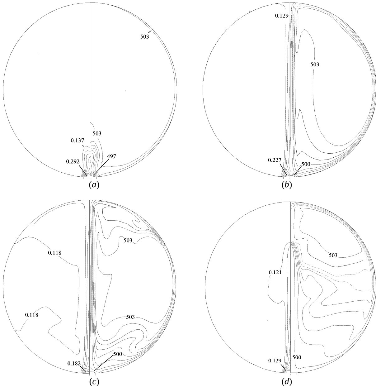
Figure 6: Calculated isolines of oxygen mass fraction (left hemisphere) and temperature (right hemisphere) at time (a) 3 s; (b) 10; (c) 20; and (d) 100 s after injection. Initial oxygen pressure is 29.67 bar. Initial n -butane pressure is 3.2 bar. Injection duration is 0.01 s. The interval between the isolines is uniform
