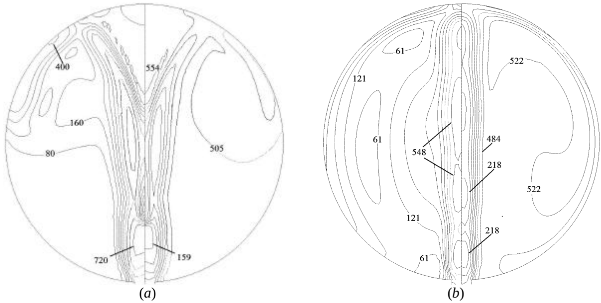
Figure 3: Calculated isolines of the velocity vector length (in m/s, left hemisphere) and temperature isotherms (in K, right hemisphere) at injection of pressurized oxygen into a vessel filled with n -butane at time (a) 2.3 ms and (b) 5.5 ms after valve opening. Initial oxygen pressure is 21 bar. Initial n -butane pressure is 0.4 bar. Injection duration is 0.0117 s. The interval between the isolines is uniform
