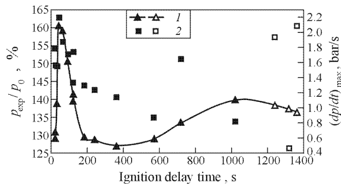
Figure 2: Measured explosion pressure p_{\text{exp}} (1) and maximum rate of pressure rise (dp/dt)_{\text{max}} (2) as a function of forced ignition delay time in the fuel-rich 78% \text{C}_4\text{H}_{10} + 22% \text{O}_2 mixture at p_0 = 4.1 bar and T_0 = 500 K [1]. Closed symbols are related to forced ignition, open symbols to self-ignition
