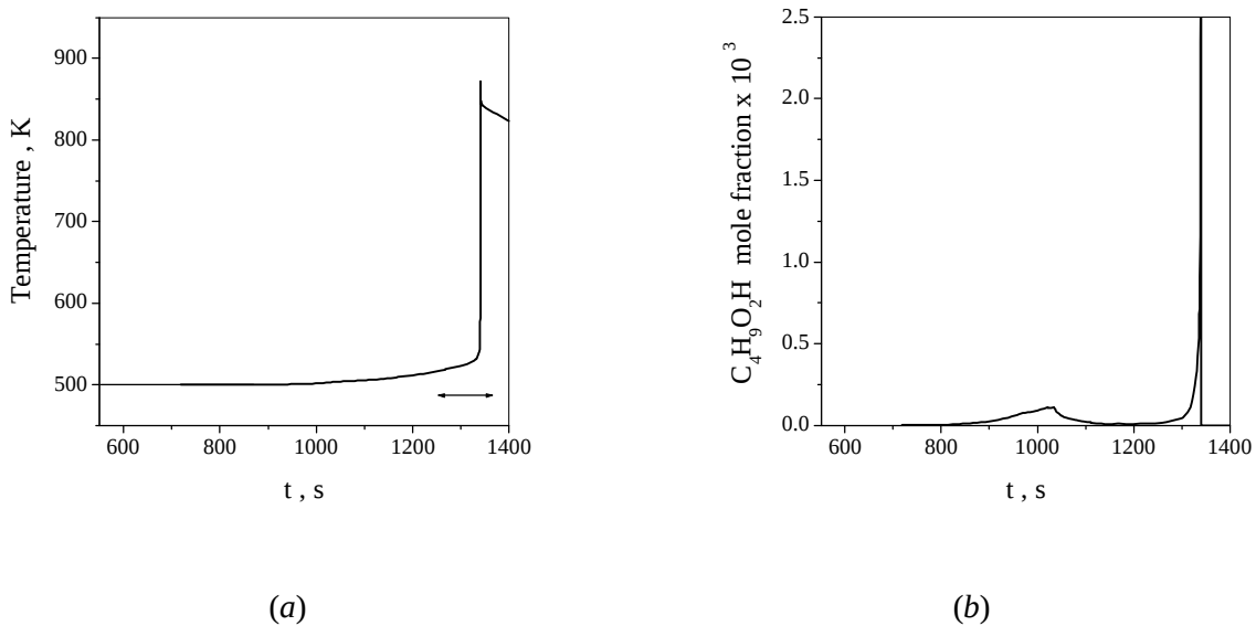
Figure 8: (a) Predicted temperature history in the 78% C 4 H 10 + 22% O 2 test mixture in the course of self-ignition at T_0 = 500 K and p_0 = 4.1 bar (arrow shows the experimental self-ignition delay); (b) Predicted time history of butyl hydroperoxide mole fraction in the test mixture
