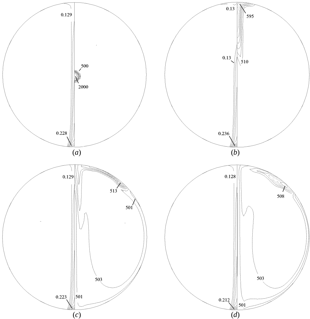
Figure 9: Calculated isolines of oxygen mass fraction (left hemisphere) and temperature (right hemisphere) after ignition of test mixture in the vessel center 10 s after termination of oxygen injection: (a) ignition completion; (b) 0.3 s; (c) 1; and (d) 2 s. Initial oxygen pressure in the canister is 29.67 bar. Initial n -butane pressure in the vessel is 3.2 bar. Injection duration is 0.01 s. The interval between the isolines is uniform
