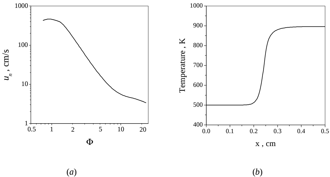
Figure 7: (a) Predicted laminar burning velocities of n -C 4 H 10 –O 2 mixtures as a function of equivalence ratio \Phi at T_0 = 500 K and p_0 = 4.1 bar; (b) Calculated temperature profile in the n -C 4 H 10 –O 2 laminar flame at \Phi = 23 at T_0 = 500 K and p_0 = 4.1 bar
