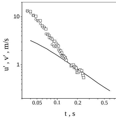
Figure 4: Comparison of predicted and measured [1] root-mean-squared velocity fluctuations u' and v' in the vessel center. Initial oxygen pressure is 21 bar. Initial n -butane pressure is 0.4 bar. Injection duration is 0.0117 s
