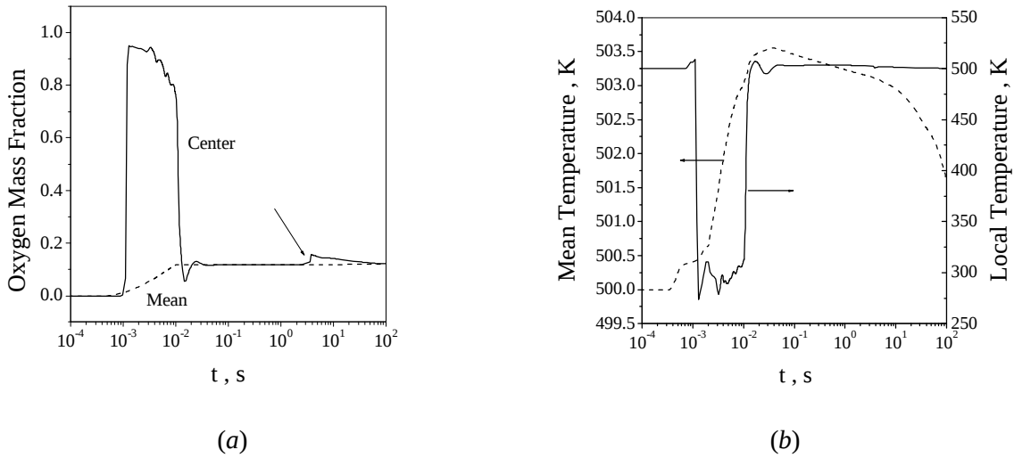
Figure 5: Calculated time histories of (a) oxygen mass fraction and (b) temperature in the 20-liter vessel. Solid curves correspond to local instantaneous values at the ignition site (vessel center). Dashed curves correspond to mean values. Initial oxygen pressure in the canister is 29.67 bar. Initial n -butane pressure in the vessel is 3.2 bar. Injection duration is 0.01 s
