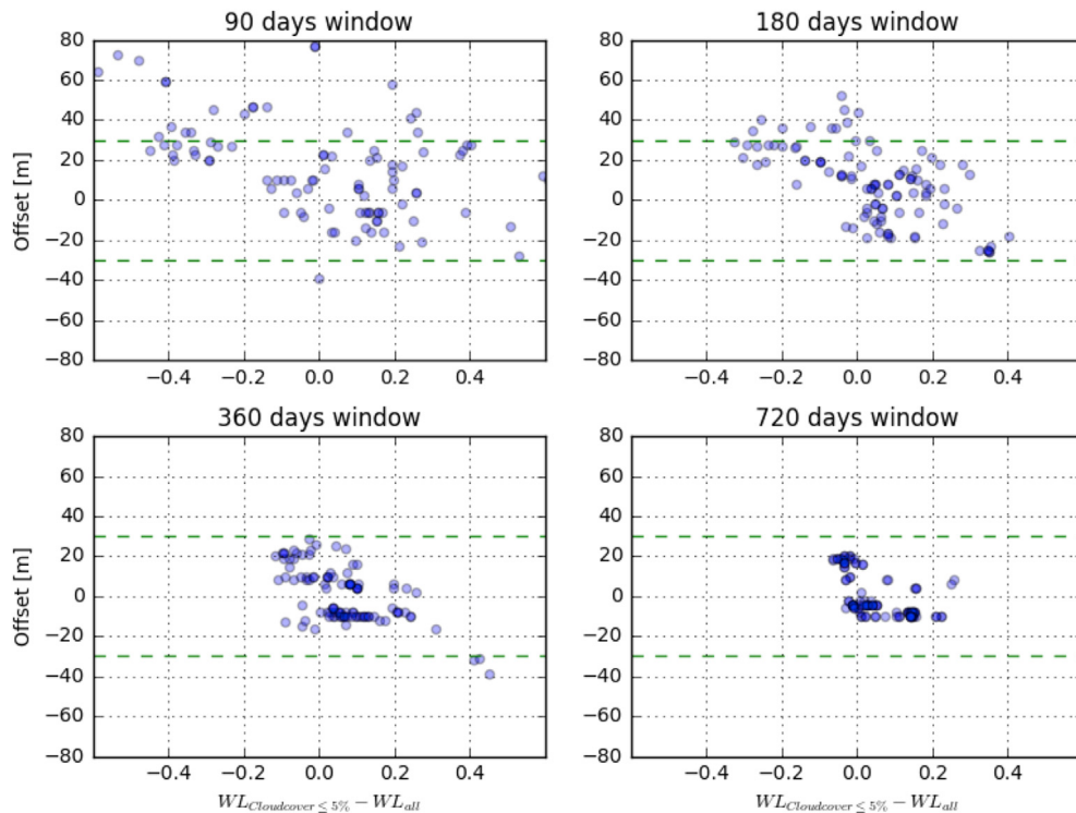
Fig. 16. Effect of the image composite moving average time windows on the difference between the water level observed on the underlying cloud free images ( WL_{Cloudcover \leq 5\%} ) and on all underlying images ( WL_{all} ) within a time window in relation to the offset value. All values are based on the values found at the first transect. The Landsat pixel resolution is indicated in green. (For interpretation of the references to colour in this figure legend, the reader is referred to the Web version of this article.)
