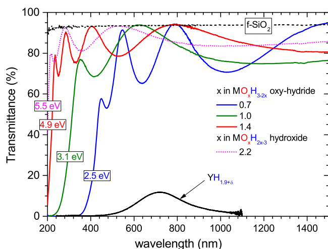
Figure 4. Transmittance spectra of Y-based ternary M–O–H films corresponding to Figure 2 with different compositions illustrating the metal–insulator transition from the dihydride \text{YH}_{1.9+\delta} to the oxyhydride \text{MO}_x\text{H}_{3-2x} phase followed by band gap widening with increasing \text{O}^{2-}/\text{H}^- ratio. The transmittance of a hydroxide-like film with a large \text{H}^+ concentration of \sim 30 atom % is shown for comparison. The optical band gap values as obtained from Tauc plots are given. The black dashed line is the transmittance of the bare fused silica substrate.
