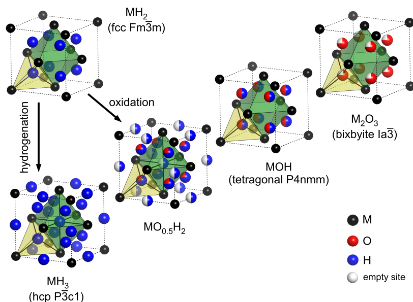
Figure 3. Generalized crystal structure evolution of rare-earth oxyhydrides with different \text{H}^-/\text{M} and \text{O}^{2-}/\text{M} ratios based on the fcc-fluorite ( \text{Fm}\bar{3}m ) structure motif. Anion sublattice disorder is visualized by multicolored spheres in terms of partial occupancy of tetrahedral (yellow polygon) and octahedral (green polygon) sites. The corresponding anion-ordered crystal structures of fcc- \text{MH}_2 , hcp- \text{MH}_3 , tetragonal \text{MOH} , 5,6 and bixbyite- \text{M}_2\text{O}_3 24 are given in parentheses. The arrows indicate metal–insulator transitions.
