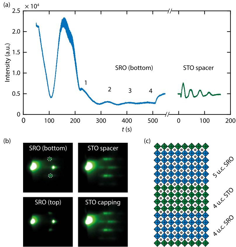
Figure 1. PLD synthesis. (a) RHEED intensity of the first-order diffraction spot during PLD growth of the first SRO and STO layers. (b) Post-growth RHEED patterns after each layer. (c) Illustration of the grown heterostructure, which consists of 4 u.c. SRO, 4 u.c. STO, 5 u.c. SRO and a 10 u.c. STO capping layer, grown on an STO substrate.
