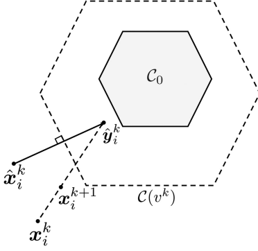
Fig. 1. Illustration of the payoff allocation proposed by an agent i , as in (8) where \hat{y}_i^k := \text{overproj}_{C(v^k)} \hat{x}_i^k .
