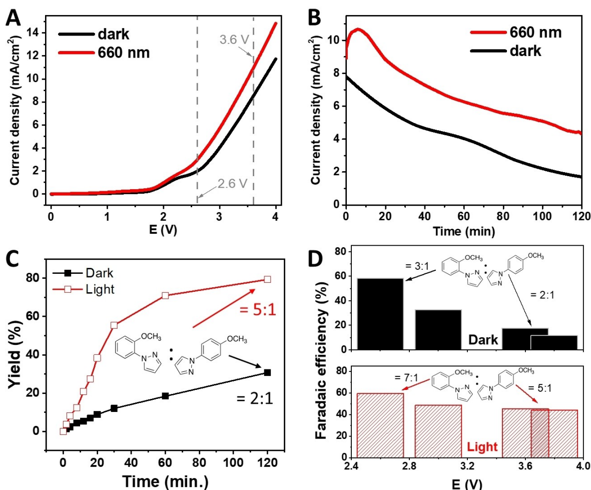
Figure 2. (A) – LSV curves, measured during C–H amination (pyrazole and anisole model case) proceeding on Au@Pt grating electrode surface in dark or under illumination (i.e. with plasmon assistance); (B) – chronoamperometric curves measured during amination proceeding in dark and light under 3.6 V vs RHE potential; (C) – time-resolved yields and regioisomers ratio of methoxyphenyl-1H-pyrazole obtained in the dark or under plasmon-assisted C–H amination; (D) – Faradaic efficiency of C–H amination and produced regioisomers ratio as a function of used potential with or without plasmon triggering.
