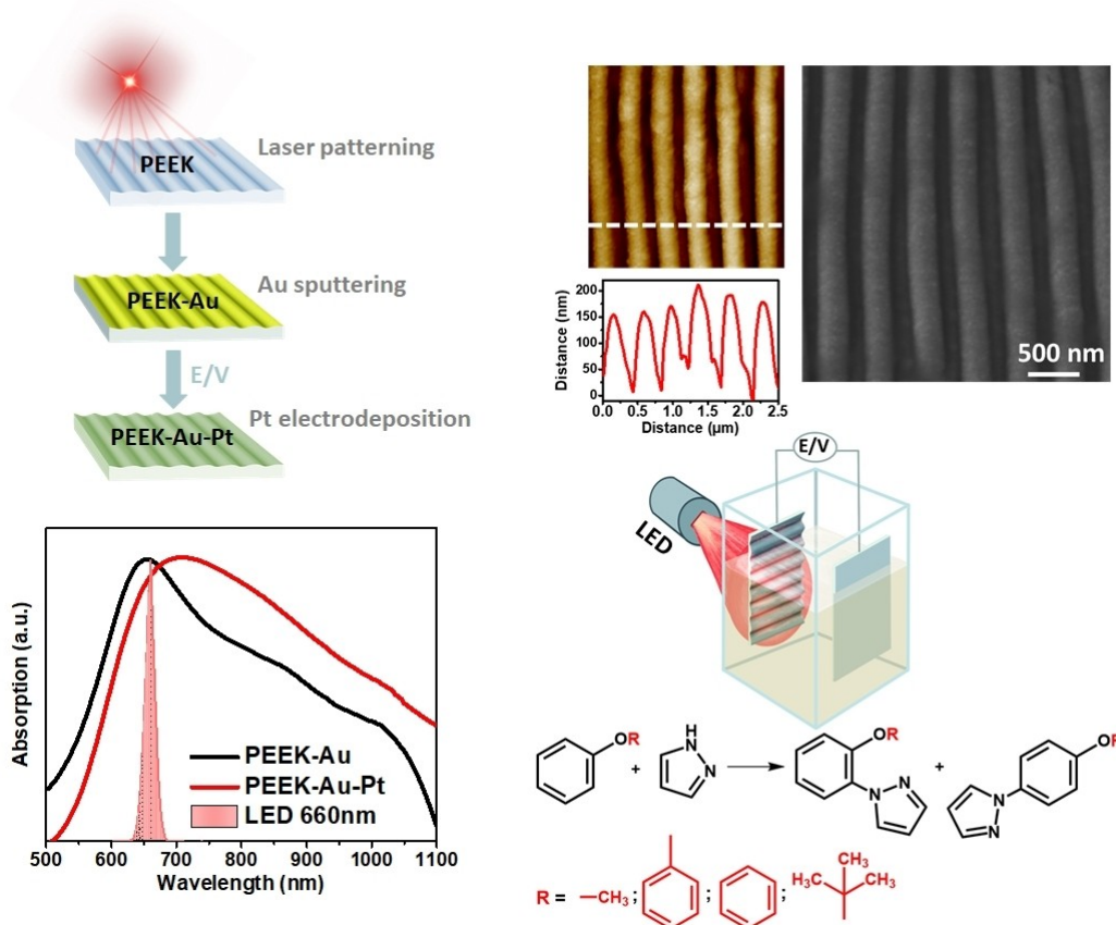
Figure 1. (A) – Schematic representation of Au@Pt photo-electrode preparation: creation of grating-like polymer template, Au sputtering, and Pt electrochemical deposition; (B) – Au@Pt grating surface morphology measured by AFM (including surface profile and SEM); (C) – UV-Vis absorption spectra of pristine Au grating and Au@Pt grating (emission spectrum of used LED is also presented); (D) – schematic representation of experimental set-up and C–H amination with the formation of ortho- and para- regioisomers.
