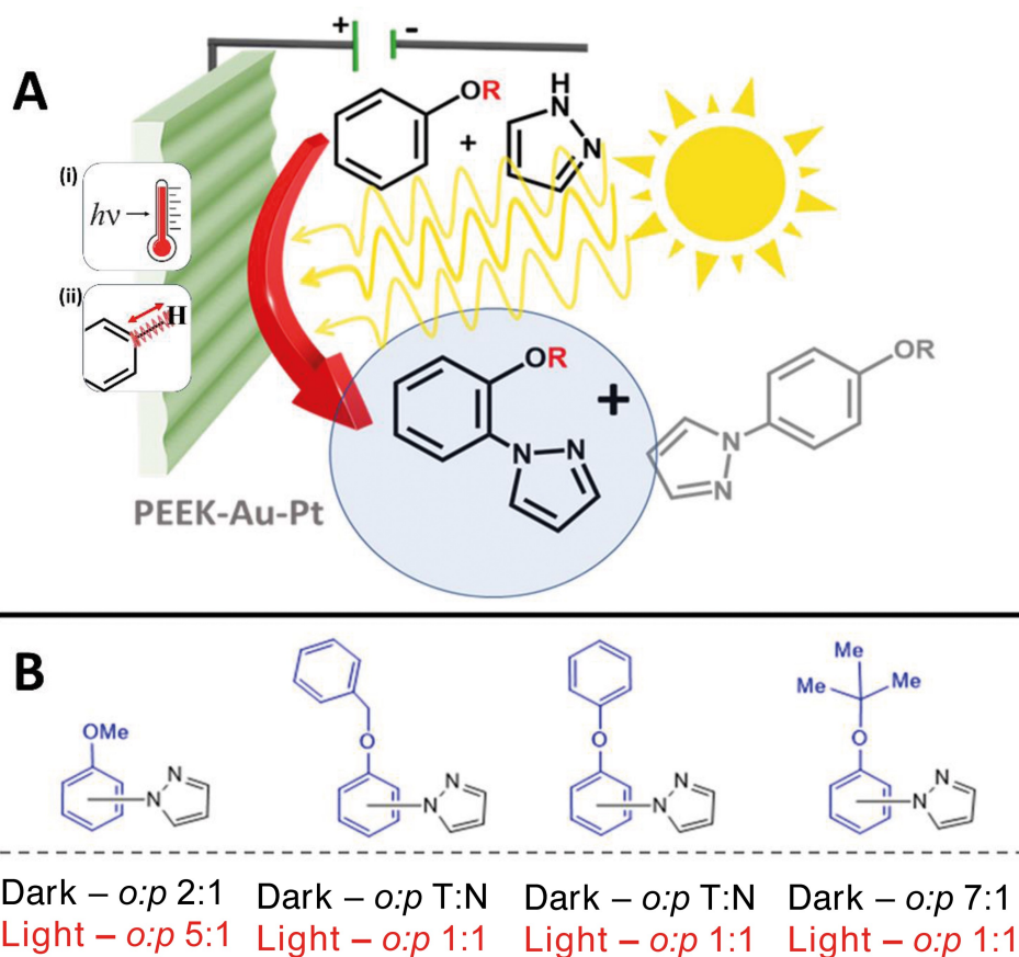
Figure 3. (A) – Schematic representation of C–H amination (pyrazole and benzene derivatives) performed in plasmon-assisted photoelectrochemical mode and (B) – ratio of ortho:para regioisomers, obtained with (Light) or without (Dark) plasmon triggering.
