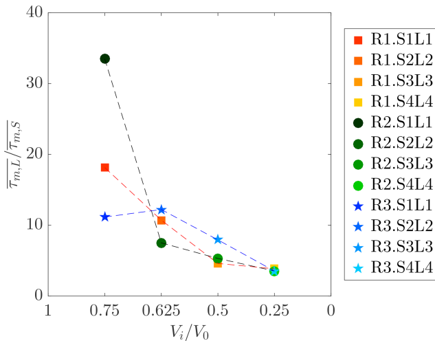
Figure 7. Ratio between time-averaged interface shear stress of tests with varying lock lengths ( \bar{\tau}_{m,L} ) and test with varying lock slopes ( \bar{\tau}_{m,S} ) versus percentage of volume of the upstream lock reach V_i/V_0 . Dashed lines link tests performed with the same initial excess density.
