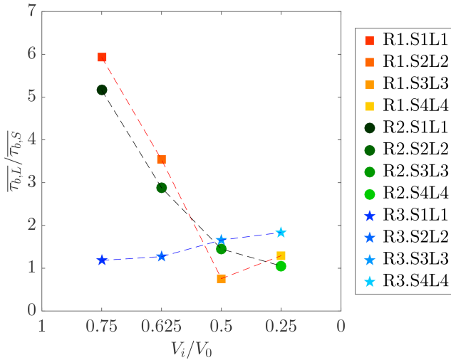
Figure 6. Ratio between time-averaged bed shear stress of tests with varying lock lengths ( \bar{\tau}_{b,L} ) and test with varying lock slopes ( \bar{\tau}_{b,S} ) versus percentage of volume of the upstream lock reach V_i/V_0 . Dashed lines link tests performed with the same initial excess density.
