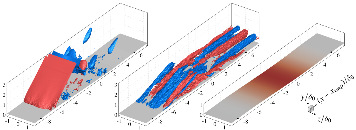
Fig. 10 Real part of a representative low-frequency mode in the SPDMD solution of the coupled interaction ( St_{Lsep} = 0.015 ): (left) modal pressure, (center) modal streamwise velocity, (right) modal displacements. Front and rear edges of the flexible panel are indicated with black circles. Iso-contours in the left and center panels indicate strong positive (red) and negative (blue) fluctuations, and the corresponding surface geometry is indicated in gray. In the right panel, the surface geometry is colored by the modal displacements.
