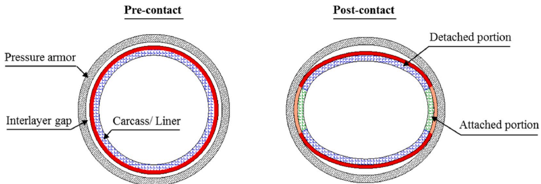
Fig. 5. Progressive buckling process of an encased carcass in wet collapse.
