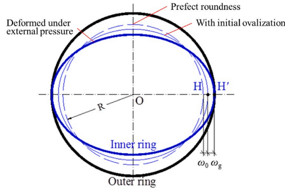
Fig. 6. Contact moment of a concentric ring structure.
