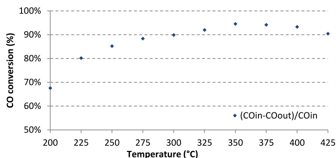
Fig. 9. Carbon monoxide conversion with ZnO–CuO as a function of temperature.
