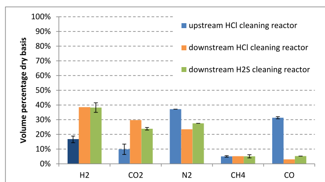
Fig. 10. Main gas composition measured in the pilot plant using wood chips as fuel.
