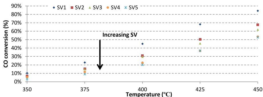
Fig. 8. Carbon monoxide conversion in the presence of K_2CO_3 as a function of temperature and space velocity.
