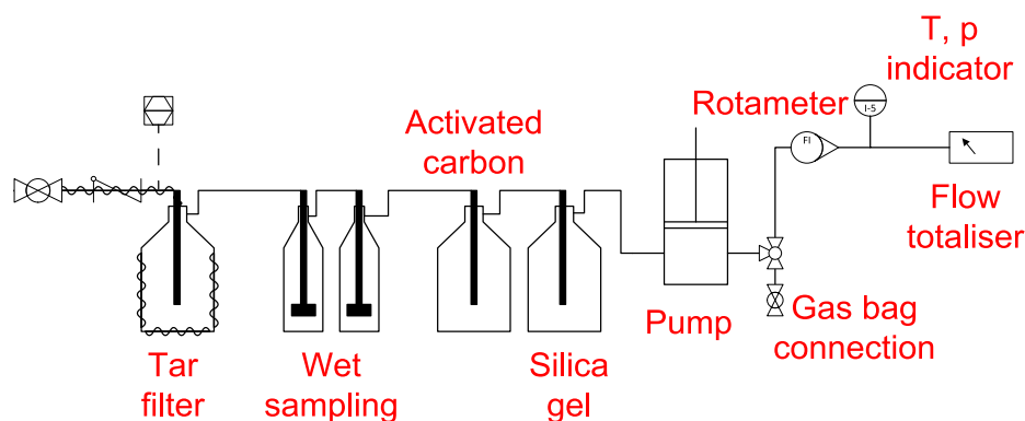
Fig. 4. Sampling train used in pilot-plant tests.
