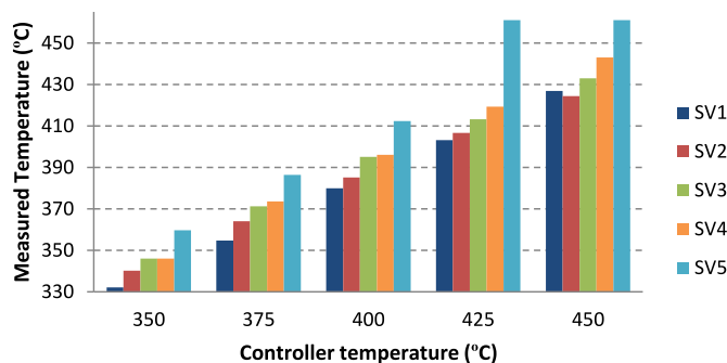
Fig. 6. Temperature measured at the top of the sorbent bed as a function of the space velocity and the temperature set point ( \text{SV1} = 150 \text{ h}^{-1} , \text{SV5} = 750 \text{ h}^{-1} ).
