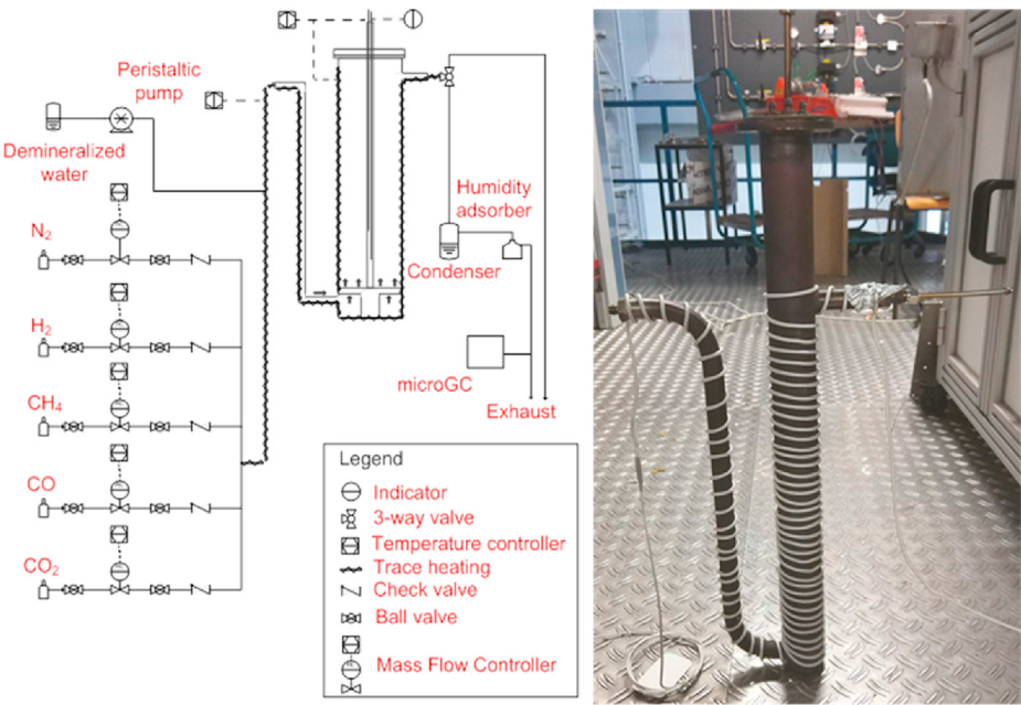
Fig. 2. Schematic representation of the second version of the FlexiFuel-SOFC system [39].
