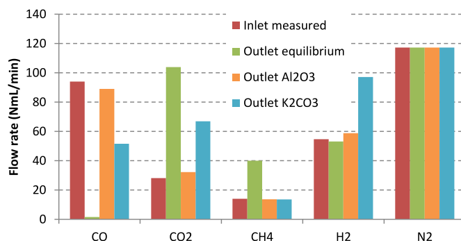
Fig. 7. Gas flow rates experimental results measured at \text{SV} of 150 \text{ h}^{-1} and 400^\circ\text{C} , and equilibrium composition.
