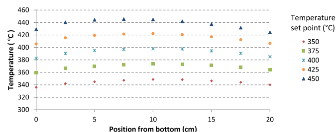
Fig. 5. Temperature profiles measured along the height of the reactor at different temperature set points.
