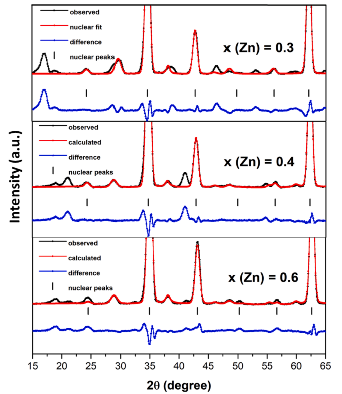
Fig. 10. Neutron diffraction patterns at 100 K with a fit of only the nuclear contribution.
