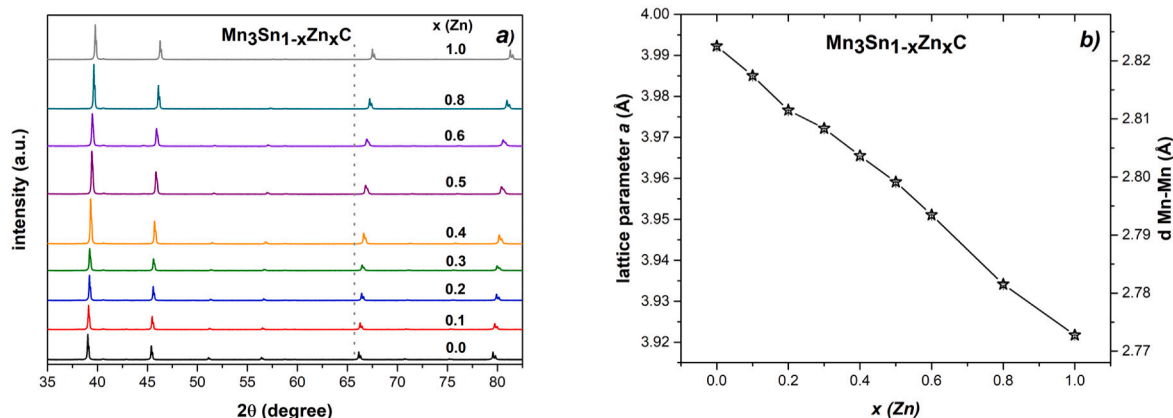
Fig. 1. a) stacked xrd patterns measured at 298 K, b) composition dependence of the lattice parameter a and the nearest Mn-Mn distance in \text{Mn}_3\text{Sn}_{1-x}\text{Zn}_x\text{C} compounds measured at 298 K. The error bars are smaller than the size of the marker.
