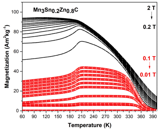
Fig. 6. Temperature dependence of the magnetization measured for x(\text{Zn}) = 0.8 in magnetic fields up to 2 T.
