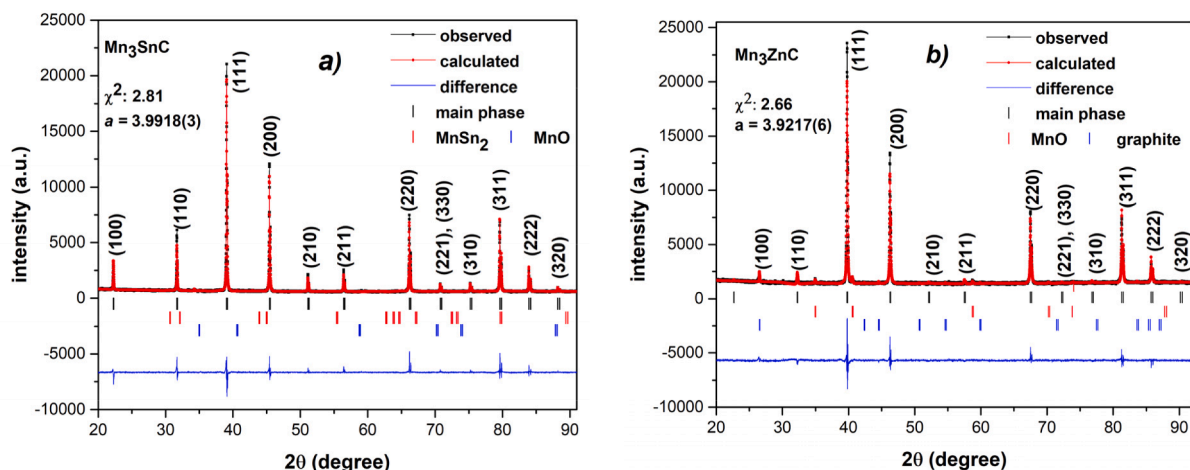
Fig. 2. Observed and calculated XRD patterns of a) \text{Mn}_3\text{SnC} and b) \text{Mn}_3\text{ZnC} at 298 K.
