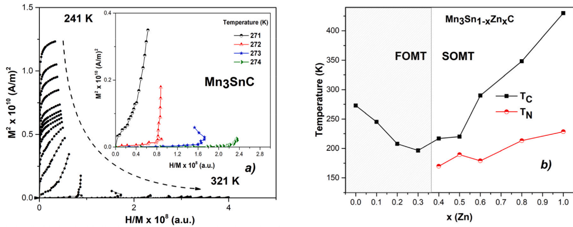
Fig. 5. a) Arrott plots derived for \text{Mn}_3\text{SnC} from isofield curves measured upon heating in the vicinity of T_C , b) changes in T_C and T_N as a function of Zn content in \text{Mn}_3\text{Sn}_{1-x}\text{Zn}_x\text{C} compounds. The error bars for T_C and T_N are within the marker size ( \pm 1 K).
