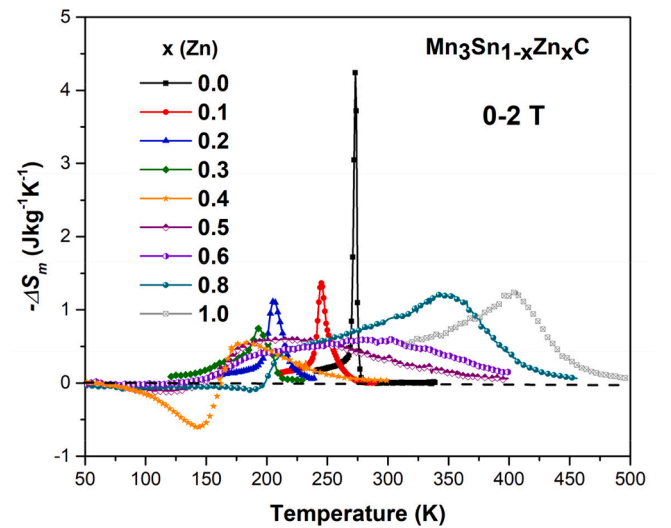
Fig. 9. Magnetic entropy change ( -\Delta S_m ) of \text{Mn}_3\text{Sn}_{1-x}\text{Zn}_x\text{C} , derived from M-T curves measured in a magnetic field change of 2 T.
