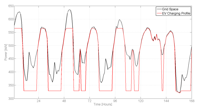
Fig. 9. Comparison of the Available Grid Space and Combined EV Charging Profile for 240kW DC and 3.7kW
