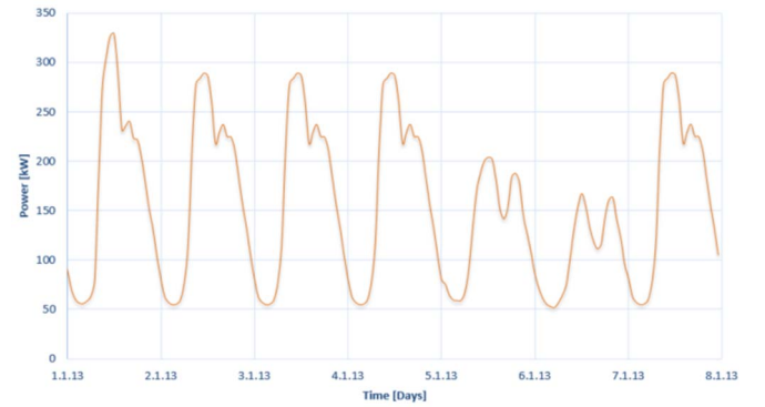
Fig. 1. Aggregated Base Load Profile
