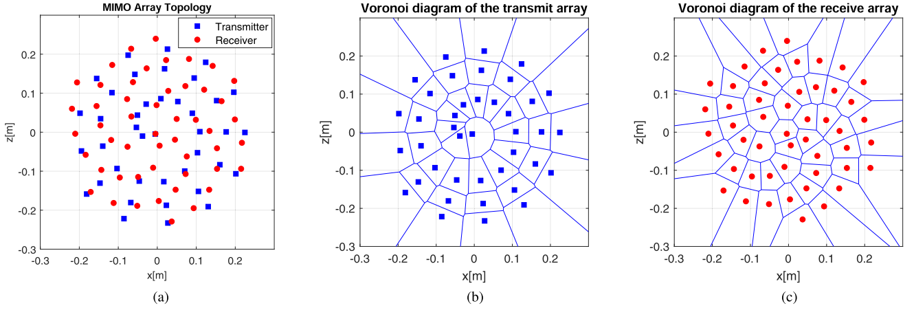
Fig. 6. MIMO array used for numerical simulation. (a) Shows the MIMO array topology formed by 40 transmit and 50 receive antennas. (b) and (c) Display the Voronoi diagrams related to the transmitting and receiving antenna arrays, respectively.
