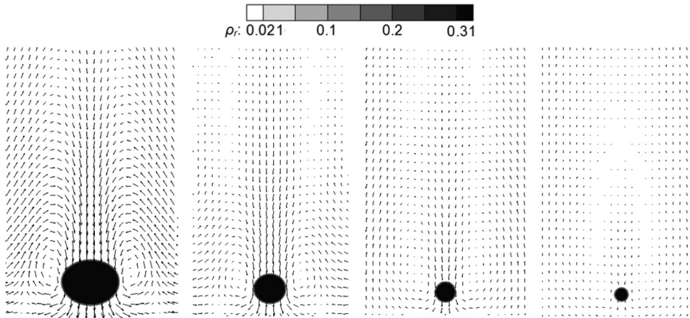
FIG. 12. The time evolution of density and instantaneous velocity field for moving an evaporating droplet. From left to right: t = 0, t = 0.039, t = 0.072 , and t = 0.1 . (Note: At t = 0 the droplet is moving with its terminal velocity; i.e., U_{t,LB} = 0.06 in lattice units).
