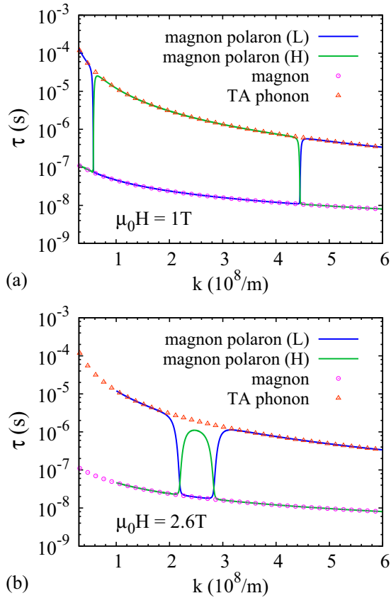
FIG. 3. (a) Scattering times of magnons, TA phonons ( \lambda = 1 ), and lower (L)/upper (H) branch magnon-polarons in YIG for \mu_0 H = 1 T ( \mathbf{H} \parallel \hat{\mathbf{z}} ) as a function of wave vector \mathbf{k} \parallel \hat{\mathbf{x}} for \eta = 100 . (b) Same as (a) but \mu_0 H_{\perp} = 2.64 T.
