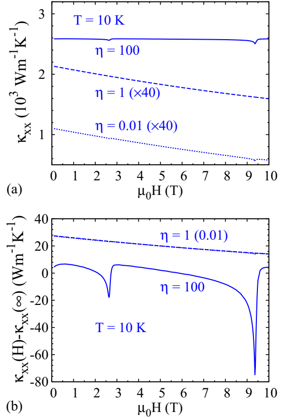
FIG. 7. (a) The magnetic field dependence of the heat conductivity \kappa_{xx} at T = 10 K for different scattering parameters \eta . (b) Magnetic field dependence of the heat conductivity difference \kappa_{xx}(H) - \kappa_{xx}(\infty) simulating the experimental procedure [24] at T = 10 K.
