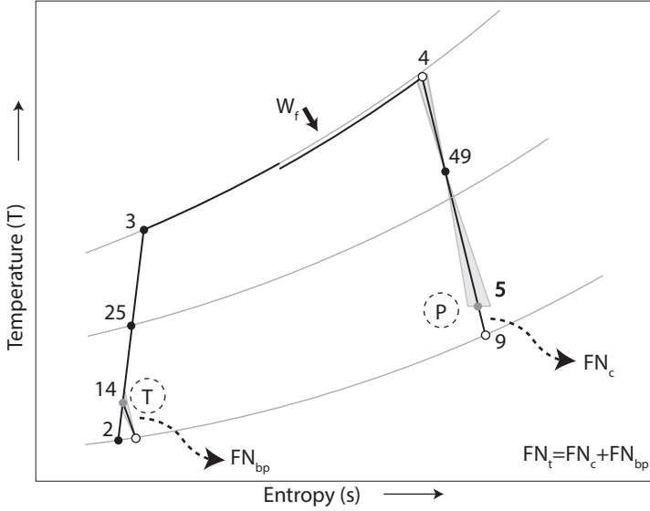
Figure 4.14: Temperature-entropy diagram for a turbofan engine. Fuel flow ( W_f ) and (total) engine thrust ( FN_t ) are used for specifying the thermodynamic cycle instead of the missing pressures and temperatures: Tt14, Tt4, Pt4, and Pt5. Total engine thrust ( FN_t ) is the sum of the fan thrust ( FN_{bp} ) and core engine thrust ( FN_c ). This results in larger uncertainty for performance parameters that are not directly measured.
