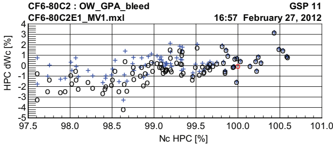
Figure 4.7: HPC mass flow capacity condition deviations graphed against the corrected HPC (N 2 ) shaft speed. o-markers show the results obtained with original maps, +-markers represent the results obtained with the tuned maps.
