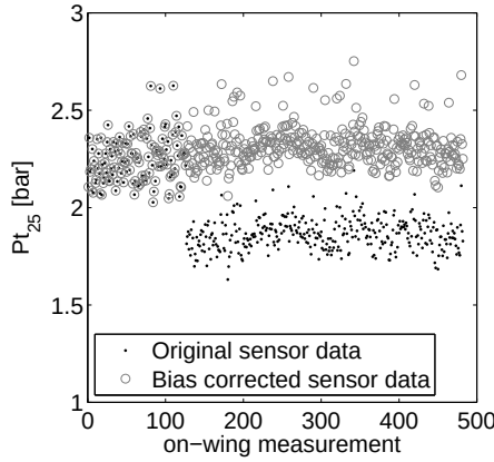
Figure 5.12: This figure shows the original Pt_{25} parameter data including the downward shift, and the data corrected with the offset value.
