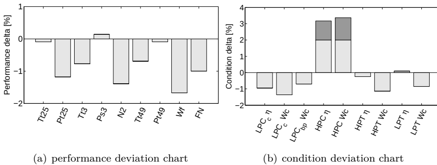
Figure 3.2: GPA results using performance data of the rejected performance test. While the HPC condition is better than the reference condition, the remaining components show slightly below average condition.
