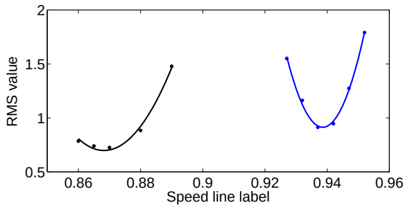
Figure 4.5: The RMS values and the corresponding best-fit curves plotted against the speed line label for the combined fan core and booster component. These graphs indicate that a minimum error would be obtained for normalized speed line labels of 0.87 and 0.94.
