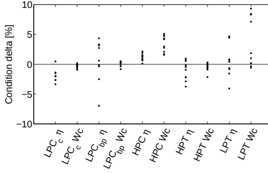
(a) CF6-80C2A5
