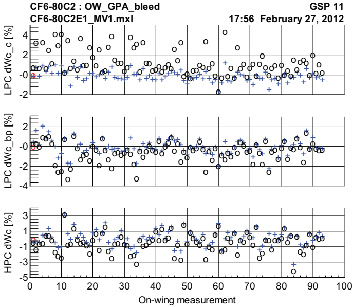
Figure 4.8: LPC core and bypass mass flow capacity condition deviations graphed in order of measurement. o-markers show the results obtained with original maps, +-markers represent the results obtained with the tuned maps.
