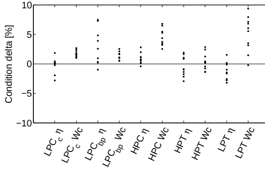
(b) CF6-80C2B1F
