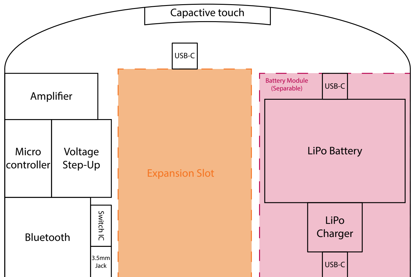
Figure 27.1: A top-view of the electronics layout.
