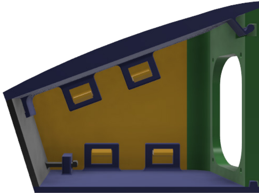
Figure 21.2: The 3D-printed model, used to discover the mistakes regarding snap-joints.
