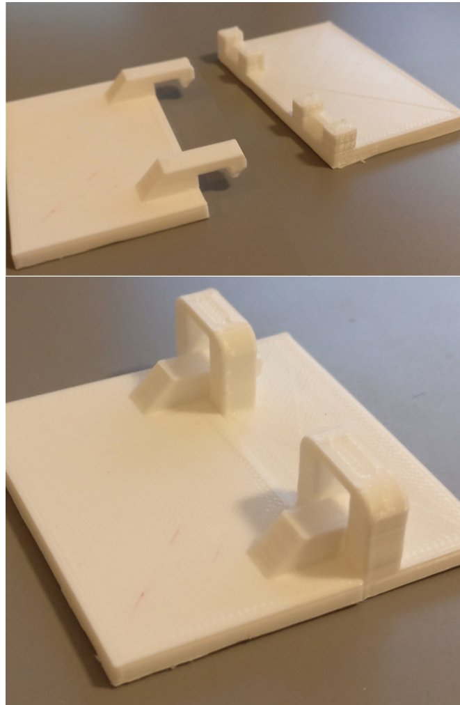
Figure 21.4: The 3D printed snap-fits
