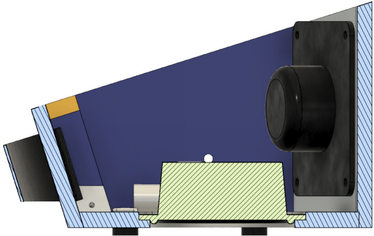
Figure 24.1: A section view of the speaker with passive radiator (yellow) installed downwards.
