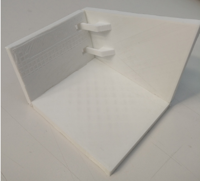
Figure 21.5: The 3D printed hinged box with snap-fits
