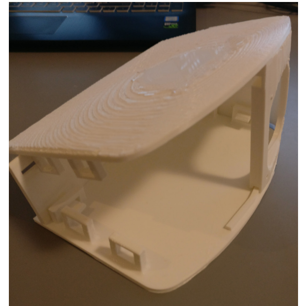
Figure 21.2: The 3D-printed model, used to discover the mistakes regarding snap-joints.
