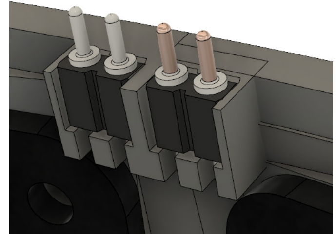
Figure 28.6: The pogo pins placed in the front pieces, these are used to connect the drivers to the rest of the electronics.
