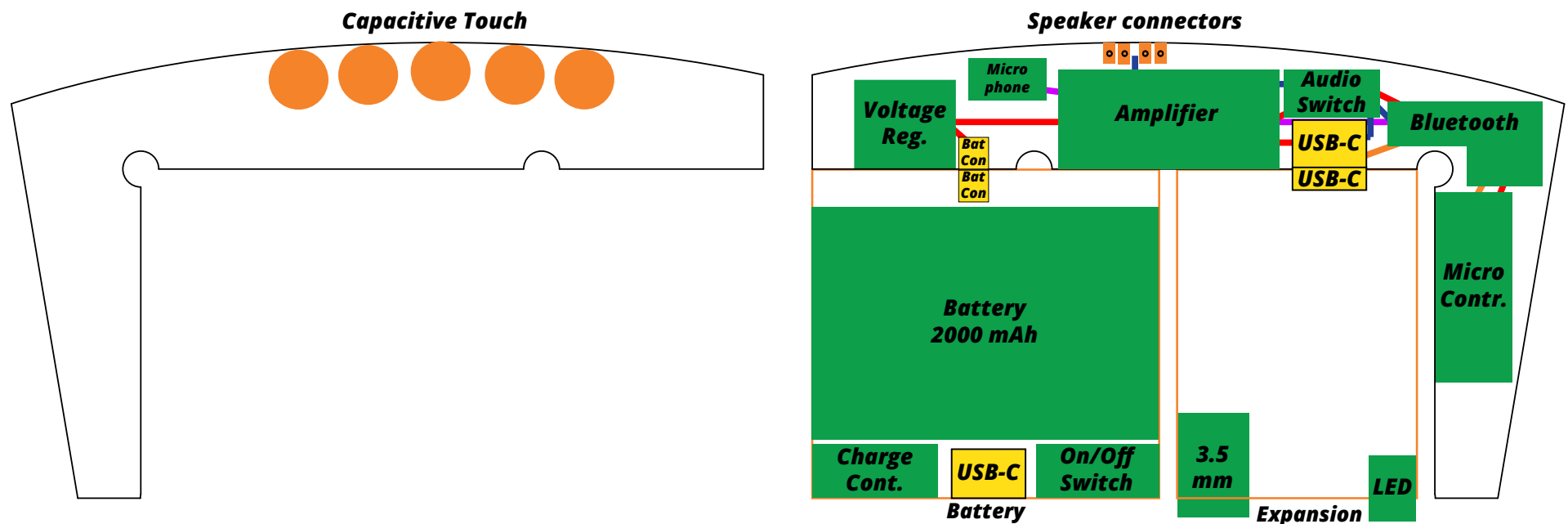
Figure 28.3: The top and bottom sides of the reorganised electronic components in the top of Mayer. Some connections between components were drawn as a indication on the low difficulty in creation of such a PCB.
