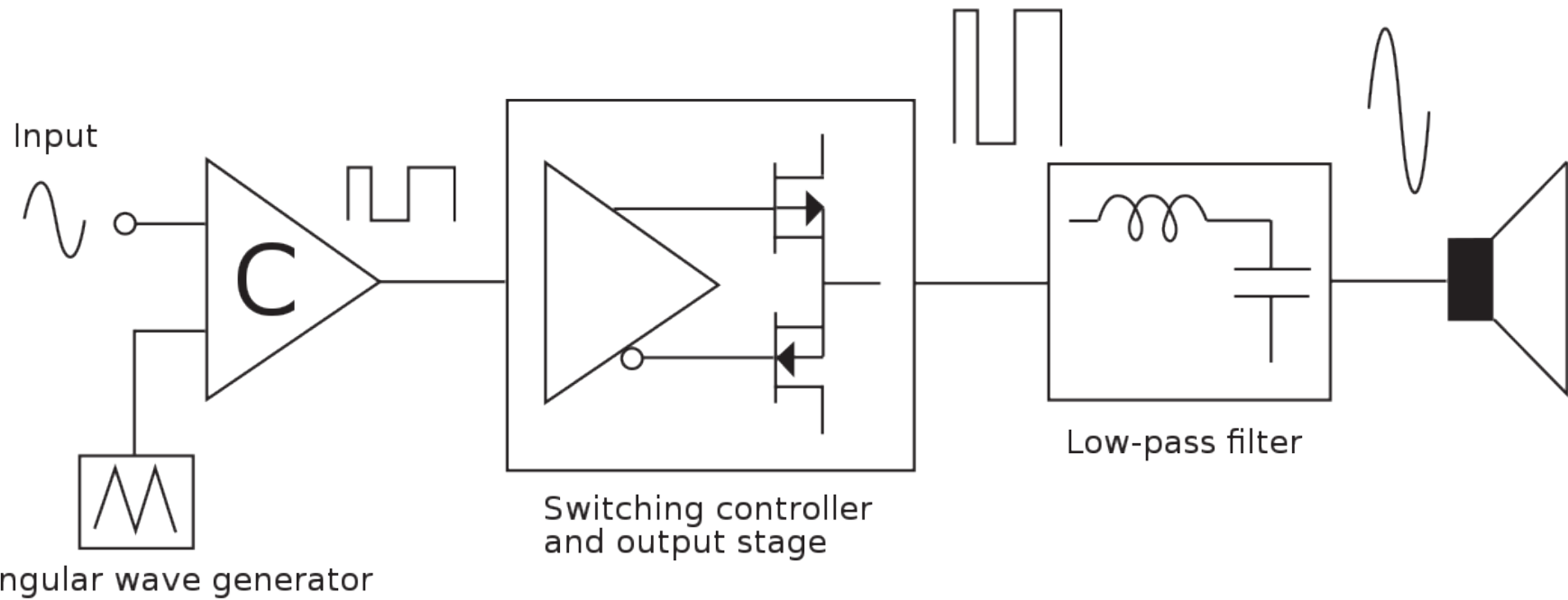
Figure A2.1: This figure shows the basic principle of Class D amplification. It might look intimidating, but the basics are as follows: the analogue signal is transform in a PWM signal. The PWM signal is amplified using MOSFETs and the amplified PWM signal is transformed back in a wave through a Low-pass filter.
