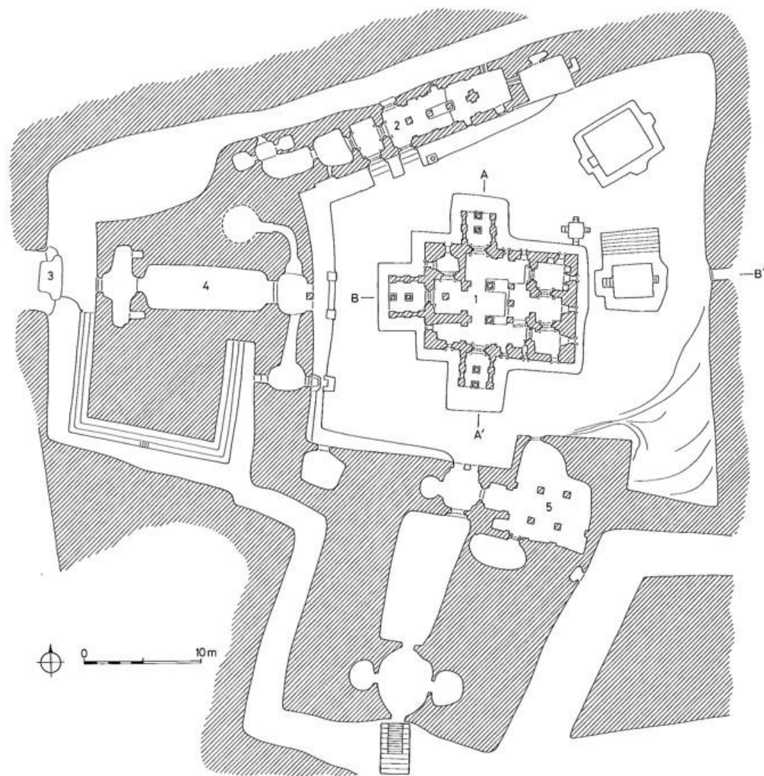
246 Lalibela, plan of part of the Northern Complex (based on Bianchi Barriviera 1957): 1 = Beta Maryam; 2 = Beta Masqal; 3 = Tomb of Adam; 4 = old approach to Beta Maryam, passing over the roof of Beta Golgotha; 5 = Beta Danagel. The sections are shown in fig. 247.
