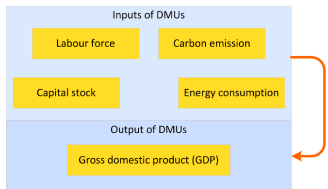
Fig. 9. Framework of the DEA model.
