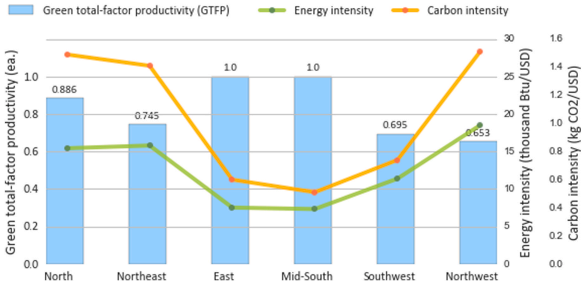
Fig. 10. GTFP and energy and carbon intensity in the six administrative regions of China in 2019.
