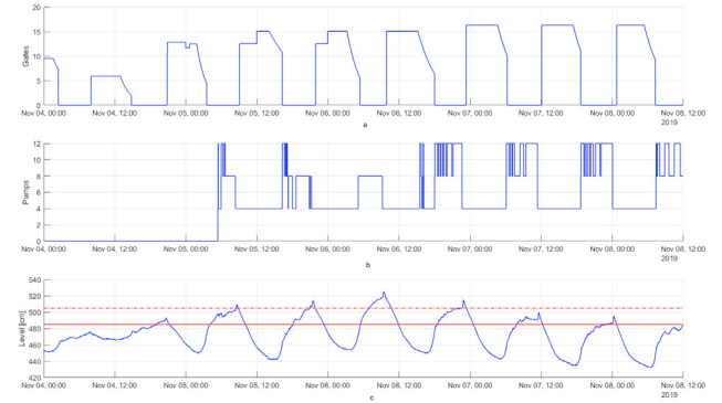
Fig. 3. Data corresponding to the Calais canal (Nov 4 to Nov 8). (a) Control of sea outlet gates. (b) Control of pumps. (c) Water level.
