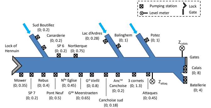
Fig. 2. Schematic representation of the Calais canal
