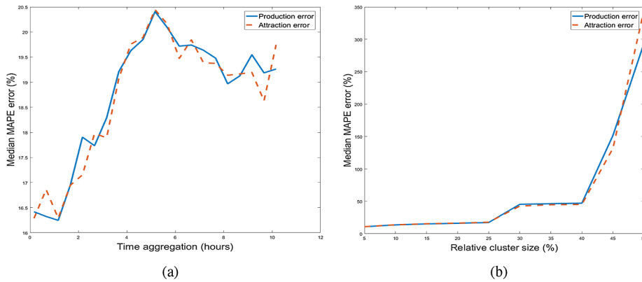
Fig. 6. Sensitivity analysis of production and attraction prediction accuracy with respect to time aggregation and number of 3D zones respectively.
