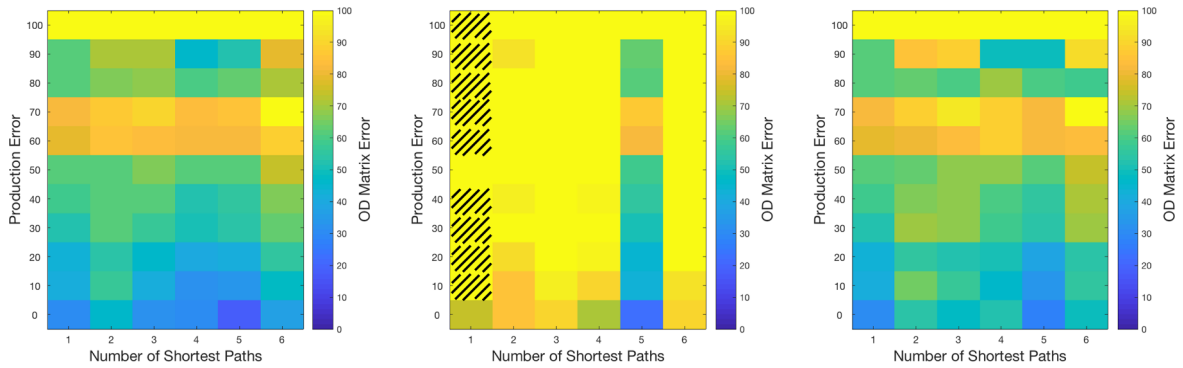
Fig. 7. Mean OD matrix estimation error for the 198 scenarios of the toy network (a) Case 1 - counts on the outer ring, (b) Case 2 - counts on the inner ring, and (c) Case 3 - counts on the inner and outer ring. The shaded region in the case 2 corresponds to the cases where some of the OD matrix estimates returned negative values implying there is no solution for these cases. These estimates were not considered when computing the mean OD matrix errors.
