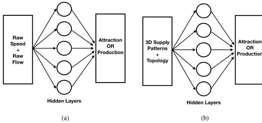
Fig. 2. Neural network model with 5 neurons in the hidden layers for (a) SF (with FV ) based predictions (b) SFT (with \hat{FV} ) based predictions.
