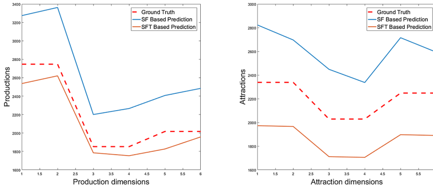
Fig. 4. Single instance of production and attraction prediction for 20 min time horizon respectively for toy network.
