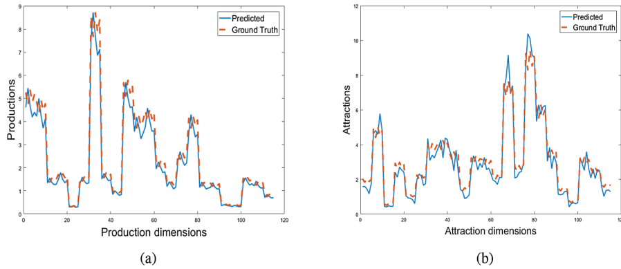
Fig. 8. Single instance of production and attraction prediction for 20 min time horizon respectively.
