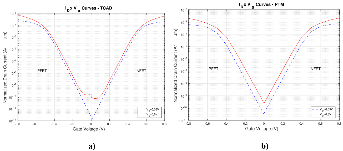
Fig. 4 Drain Current vs Gate Voltage for the transistors modeled in: a) TCAD, with physical parameter x b) SPICE, with PTM
