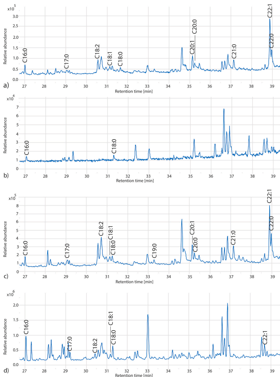
Fig. 2. Partial total ion chromatogram displaying fatty acids analyzed as TMS derivatives from solvent extracted tars produced using the following techniques: a) Condensation (Vla_C04.1); b) Ash mound (HOR_AM3); c) Pit roll (Vla_PR09.1); d) Raised structure (Vla_RS02.2).
