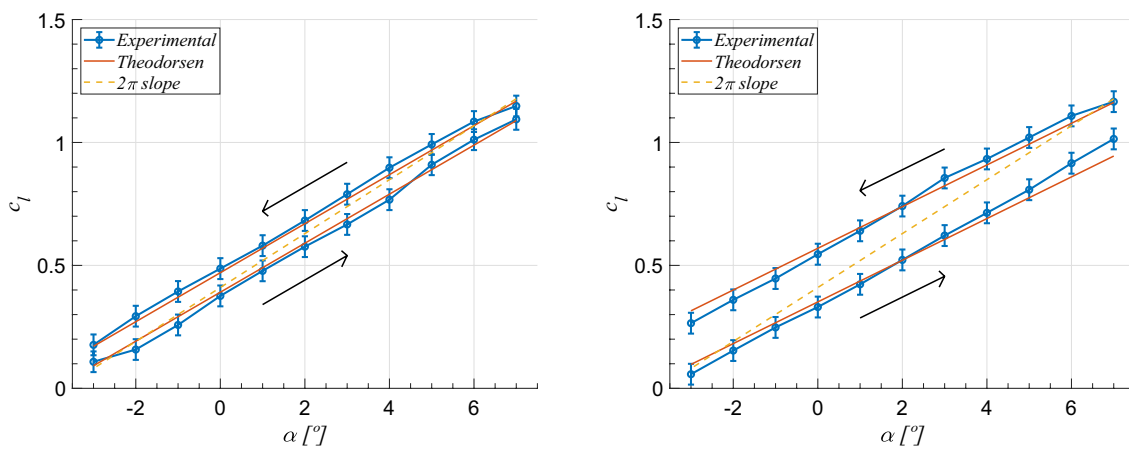
Fig. 22 Unsteady lift coefficient for the pitching wing, with k = 0.05 (left) and k = 0.15 (right)
