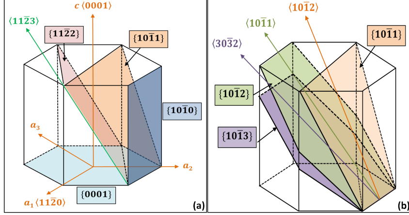
Figure 3: (Color online) Deformation modes in the hcp metals are shown. (a) Basal plane {0001} \langle 11\bar{2}0 \rangle , Prismatic plane {1010} \langle 11\bar{2}0 \rangle , Pyramidal plane type I {1011} \langle 11\bar{2}3 \rangle , and type II {1122} \langle 11\bar{2}3 \rangle slip systems (b) tension twinning (TTW) {1012} \langle 10\bar{1}1 \rangle , compression twinning (CTW1) {1013} \langle 30\bar{3}2 \rangle , and compression twinning (CTW2) {1011} \langle 10\bar{1}2 \rangle .
