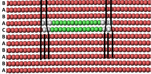
Figure 4: (Color online) A magnesium basal I2 stacking fault is shown here. Atoms are colored using CNA. Red and green atoms respectively represent the hcp and fcc atoms. The X and Y are two partials \frac{1}{3}[1100] and \frac{1}{3}[1010] , respectively.
