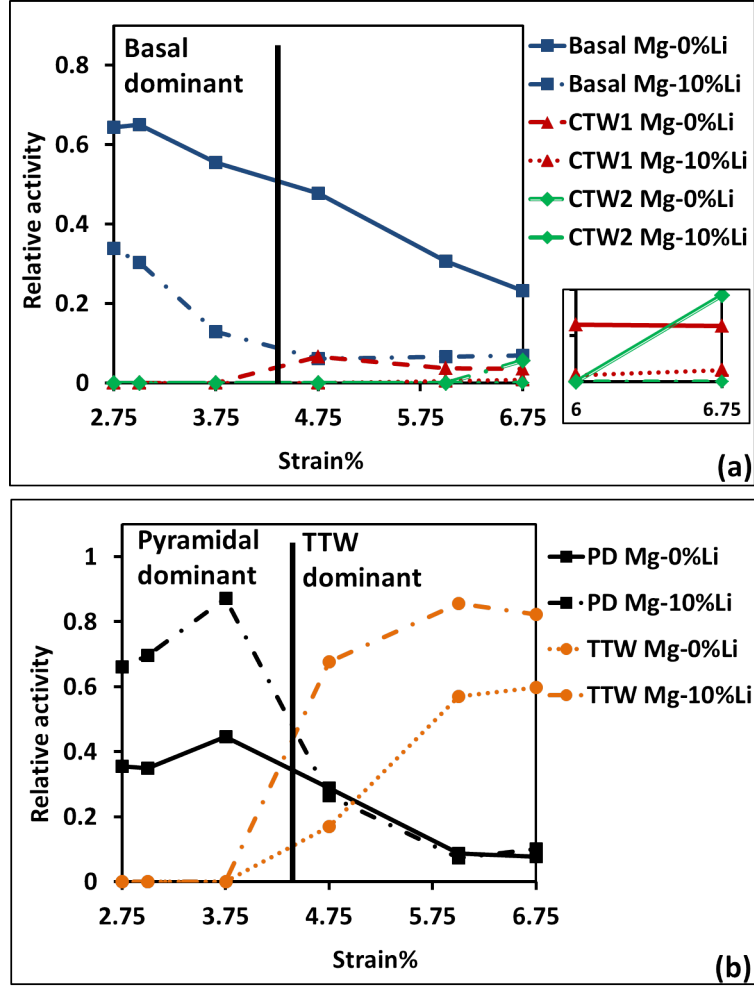
Figure 9: (Color online) The contribution of each deformation mode to total deformation (relative activity R ) is plotted as a function of strain and Li addition. PD refers to pyramidal type I dislocations. The dominant deformation modes at low and high strains are demarcated by a vertical solid black line at 4.3% strain. (a) Basal and CTW1/CTW2 modes show less activity with the Li addition, which suggests that they harden. Inset shows a magnified view at high strains. (b) Pyramidal and TTW modes show increased activity suggesting softening with Li addition. Figures also show the dominant deformation mechanisms in the early stage of plasticity (basal or pyramidal) and at high plastic strains (TTW). CTW contribution at high strains is relatively small for both compositions.
