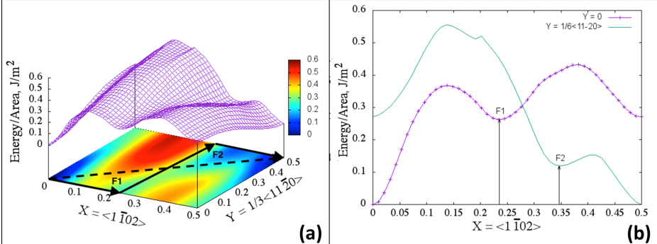
Figure 5: (Color online) (a) Stereographic and projection of the \gamma surface revealing the presence of two stable stacking faults F1 and F2 on the pyramidal I slip plane, and (b) GSFE curves obtained along the direction X = \langle \bar{1}102 \rangle with Y = 0 and Y = \frac{1}{6} \langle 11\bar{2}0 \rangle . The dashed arrow represents the Burgers vector \frac{1}{3} \langle 21\bar{1}3 \rangle , and the solid arrows represent the minimum energy path to form this Burgers vector.
