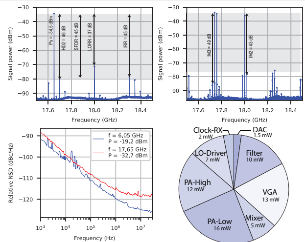
Figure 19.1.S3: RF-High output with NCO at 350MHz, Two-tone RF-High output with NCOs at 241MHz and 260MHz, Noise spectral density and power consumption of various circuit blocks, all at 3K.
