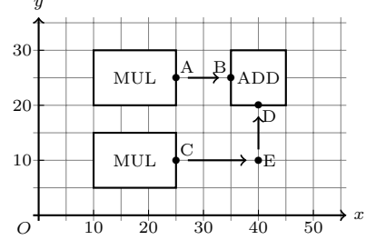
Figure 2: CIM Crossbar Communication
