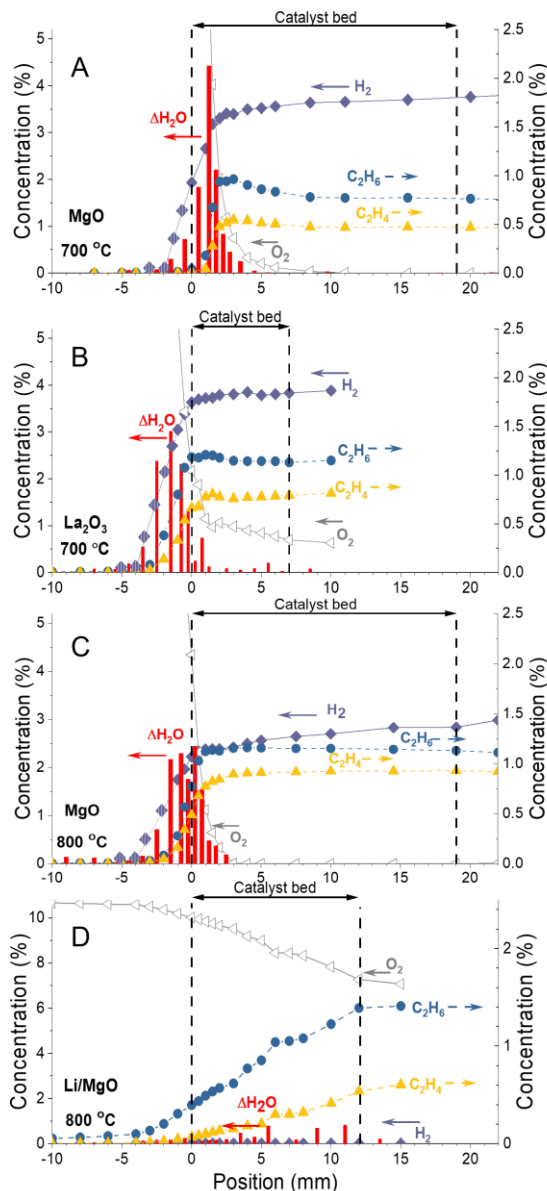
Figure 5.6: Space-resolved concentration profiles of O_2 , C_2H_6 , C_2H_4 , H_2 and formed water ( \Delta H_2O ) measured during OCM under steady-state operation on A) MgO at 700 °C, B) La_2O_3 at 700 °C, (C) MgO at 800 °C and (D) Li/MgO at 800 °C (same feed composition as in Figure 5.4)
