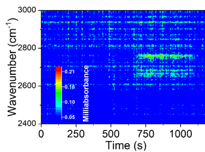
Figure B6: Dynamic evolution of surface species in the \nu(\text{CH}) stretching region from operando DRIFT spectroscopy during CCR at 350 °C with substitution of \text{CO}_2 with CO at the inlet.
