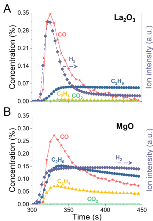
Figure 5.1: Concentrations of \text{C}_2\text{H}_6 , \text{C}_2\text{H}_4 , \text{CO}_2 and CO and ion intensity of \text{H}_2 (m/z = 2) in \text{CH}_4 pulse during OCM under unsteady-state operation on \text{La}_2\text{O}_3 (A) and \text{MgO} (B) at 900 °C. \text{C}_2\text{H}_4 , \text{CO}_2 and CO concentration is quantified by IR and \text{C}_2\text{H}_6 concentration is quantified with mass spectrometry data which are calibrated with a simultaneous gas chromatography analysis. The values are averaged over multiple stable cycles of operation.
