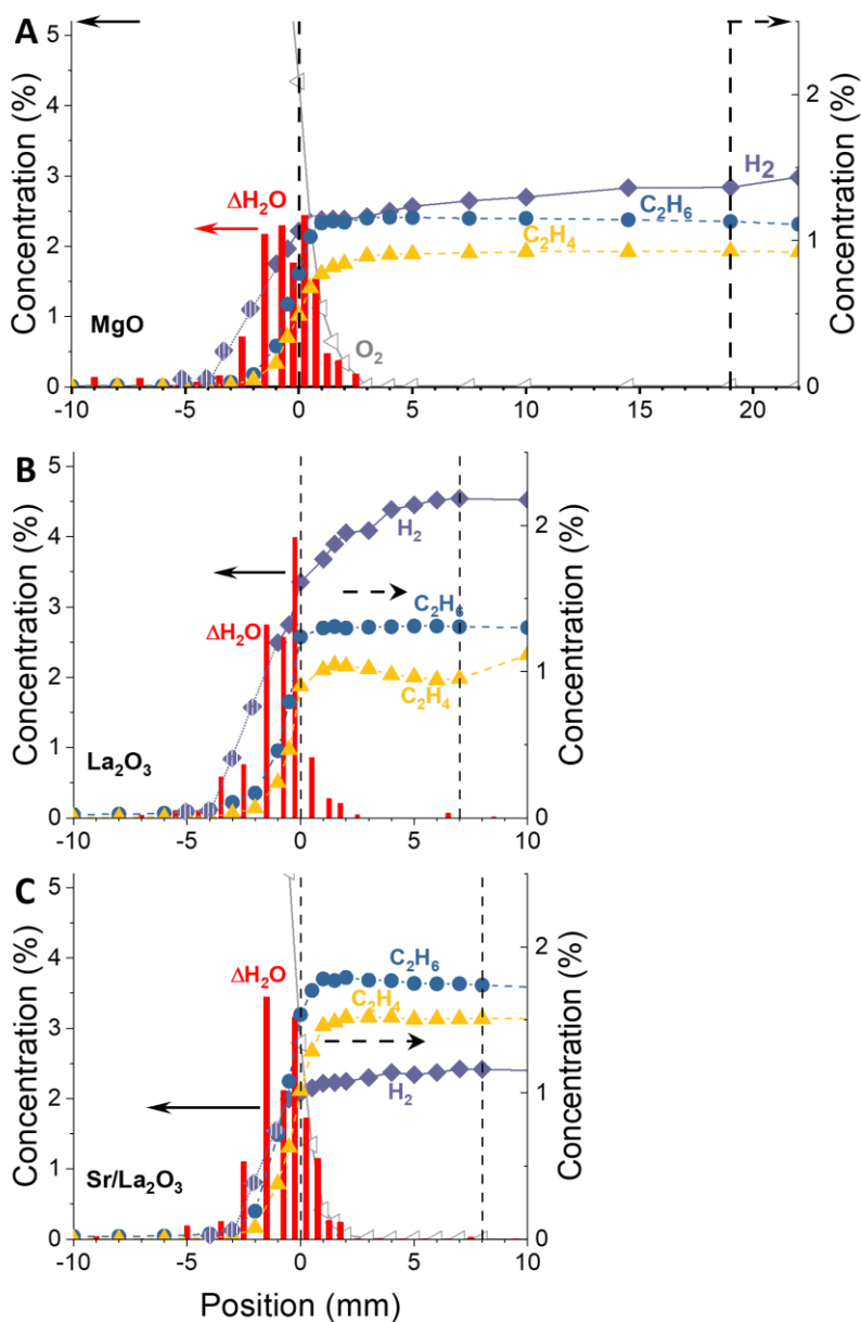
Figure D6: Spatial concentration profiles of O 2 , C 2 H 6 , C 2 H 4 , H 2 and formed water between two data points ( \Delta H_2O ) measured on MgO (A), La 2 O 3 (B) and Sr/ La 2 O 3 (C) during OCM under steady-state operation at 800 °C. \Delta H_2O is the difference value between H 2 O amount at one position and H 2 O amount at previous position, H 2 O amount is calculated by oxygen balance.
