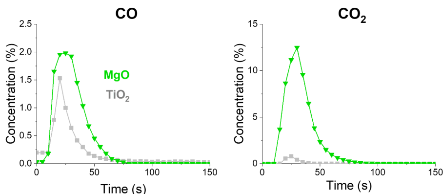
Figure 4.5: Transient analysis of CO x products (FTIR) evolved during the O 2 pulse (0-150 s, 25 vol% O 2 in He) of the catalytic tests performed at 900 °C with extended CH 4 pulse duration (900 s). The results are averaged over multiple stable cycles of operation. Results for MgO (green ▼) and TiO 2 (grey ■).
