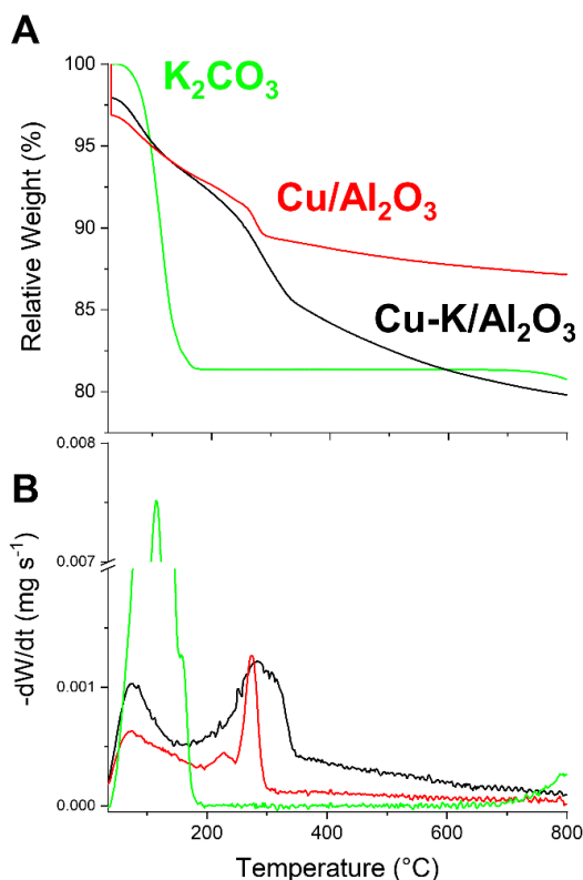
Figure B3: Thermogravimetric analysis of K_2CO_3 precursor, Cu/Al_2O_3 and Cu-K/Al_2O_3 catalysts under H_2 stream (5 vol% in Ar, 100 mL min -1 ). Sample is kept 10 min at room temperature then heated up at 10 °C min -1 rate until 800 °C. A) Relative weight change over temperature and B) derivative of weight loss with respect to time over temperature.
