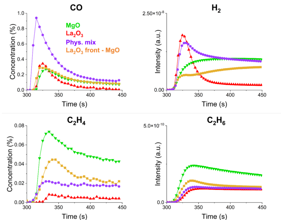
Figure 5.2: Transient analysis of products (FTIR + MS) during the CH 4 pulse (300-450 s) in unsteady-state OCM performed at 900 °C. The values are averaged over multiple stable cycles of operation. Results for La 2 O 3 (red ▲), La 2 O 3 -MgO 50 wt% physical mixture (violet ●), MgO (green ▼), La 2 O 3 (10 wt%, front of the bed)-MgO (yellow ■).
