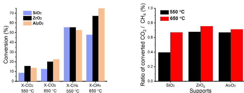
Figure 6.2: CO 2 and CH 4 conversion ( X_{CO_2} , X_{CH_4} ) obtained during DC-DRM at 550°C and 650 °C on different metal oxide-supported Ni catalysts (left, 15 wt% Ni) and ratio of converted CO 2 /CH 4 (right). DC-DRM cycle consists of the alternation of diluted CO 2 feed (10.6 vol% in He, 0-300 s), He flush (300-405 s), diluted CH 4 feed (11.2 vol% in N 2 , 405-510 s), He flush (510-615 s). Total flow rate was kept at 50 mL min -1 . Results are averaged over multiple stable cycles of operation.
