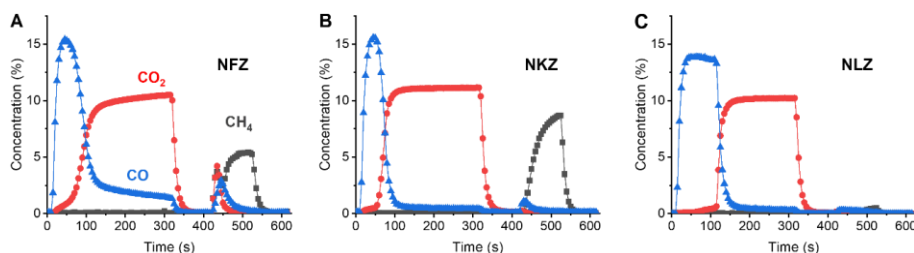
Figure 6.5: Reactor outlet gas concentrations obtained by FTIR spectroscopy during DC-DRM experiments at 800 °C on promoted Ni-ZrO 2 catalyst ('NXZ' where 'X' is 'F' for Fe, 'L' for La and 'K' for K; 15 wt% Ni, 5 wt% X). DC-DRM cycle consists of the alternation of diluted CO 2 feed (10.6 vol% in He, 0-300 s), He flush (300-405 s), diluted CH 4 feed (11.2 vol% in N 2 , 405-510 s), He flush (510-615 s). Total flow rate was kept at 50 mL min -1 . Results are averaged over multiple stable cycles of operation.
