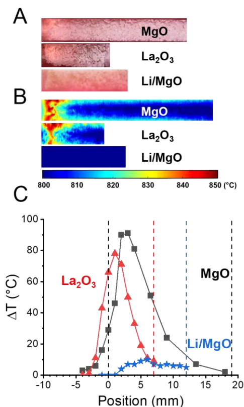
Figure 5.5: Visualization and quantification of hotspot formed during OCM under steady-state operation on \text{MgO} and \text{La}_2\text{O}_3 respectively at 800 °C: A, images of catalyst beds obtained by the digital microscope; B, images of catalyst beds acquired via infrared camera; C, spatial distribution of differential temperature of catalyst ( \Delta T ). The temperature rise is calculated by subtracting the temperature measured with 10 vol% \text{O}_2 in \text{N}_2 at 800 °C from the temperature measured during OCM under steady-state operation (the same feed composition as in Figure 5.4) at 800 °C at respective positions on corresponding catalysts.
