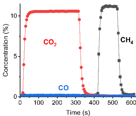
Figure 6.1: Reactor outlet gas concentrations obtained by FTIR spectroscopy during a blank DC-DRM experiment (SiC bed). DC-DRM cycle consists of the alternation of diluted \text{CO}_2 feed (10.6 vol% in He, 0-300 s), He flush (300-405 s), diluted \text{CH}_4 feed (11.2 vol% in \text{N}_2 , 405-510s), He flush (510-615 s). Total flow rate was kept at 50 \text{ mL min}^{-1} . Results are averaged over multiple stable cycles of operation.
