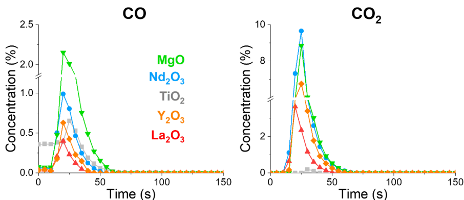
Figure 4.4: Transient analysis of CO x products (FTIR) evolved during the O 2 pulse (300-450 s, 25 vol% O 2 in He) of the catalytic tests performed at 900 °C. The results are averaged over multiple stable cycles of operation. Results for Y 2 O 3 (orange ◇), La 2 O 3 (red ▲), Nd 2 O 3 (blue ●), MgO (green ▼), TiO 2 (grey ■).
