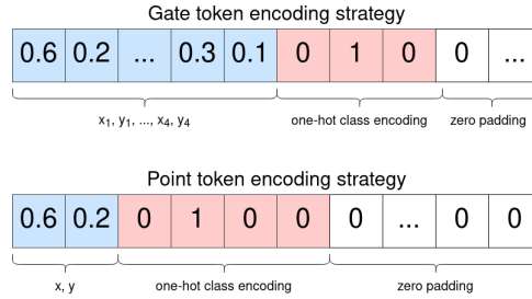
Figure 6.3: Token embeddings for predicting gates and polygons. The first 2n elements (in blue) of the vector represent the (x, y) coordinates of the n vertices/points, normalized by the image width and height. The following elements (in red) represent the class label in one-hot format. For gate detection, we have three red blocks because we have two special tokens start and end , and an object token gate . For polygon detection we have 4 red blocks because all possible tokens are start , end , point and end-of-polygon , as explained in 6.4.2. The vector is padded with zeros to reach the required dimensionality of 256.
