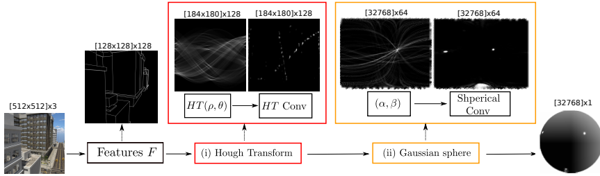
Figure 4.2: Overview: The model starts from an input image, and predicts vanishing points on the Gaussian hemisphere by relying on two geometric priors: (i) Hough Transform, and (ii) Gaussian sphere mapping. We use a convolutional network to learn features which are then mapped to Hough space, where each bin is a line. We filter the Hough space and project Hough bins to the Gaussian hemisphere and apply spherical convolutions to find vanishing points. We indicate the size of the learned features above, where the last dimension is the number of channels. We sample 32,768 points on the hemisphere using the Fibonacci lattice [59], resulting in feature maps of size 32,768. Our model learns to classify spherical points as vanishing points or not using a binary cross-entropy loss. There is no intermediate supervision.
