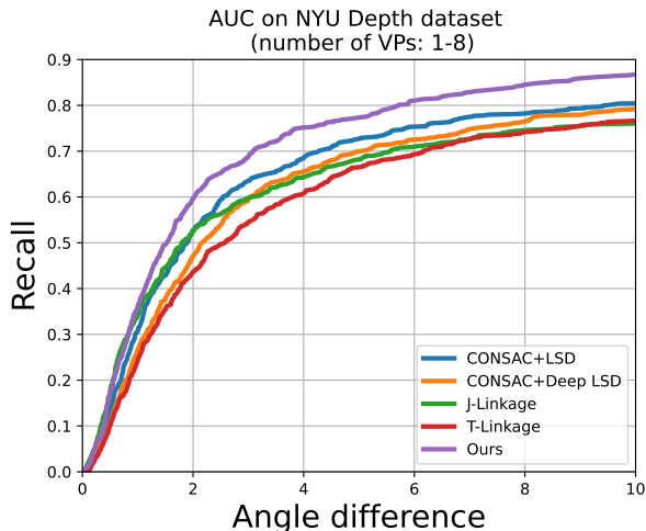
Figure 4.9: Exp 3(b): Non-Manhattan scenario. We plot the recall curve on the non-Manhattan NYU dataset. Our method outperforms state-of-the-art, illustrating the ability of the model to detect a varying number of vanishing points. See supplementary material for qualitative visualizations.
