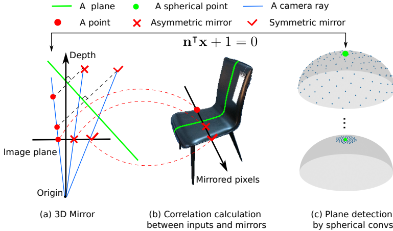
Figure 5.1: 3D mirror symmetry detection. We identify 3D mirror planes by measuring the correlations between the input and its mirrors over depth. The mirrors are calculated by 3D mirror geometry (a), which localizes the reflections of a given pixel directly on the image plane (b). We describe each candidate plane with feature correlations across points and their mirrors. We sample planes on a hemisphere, and adopt multi-stage spherical convolutions to localize the optimal plane hierarchically (c). The 3D mirror geometry is explicitly encoded in the model. We display the ground truth symmetry axis (in green) on top of the image.
