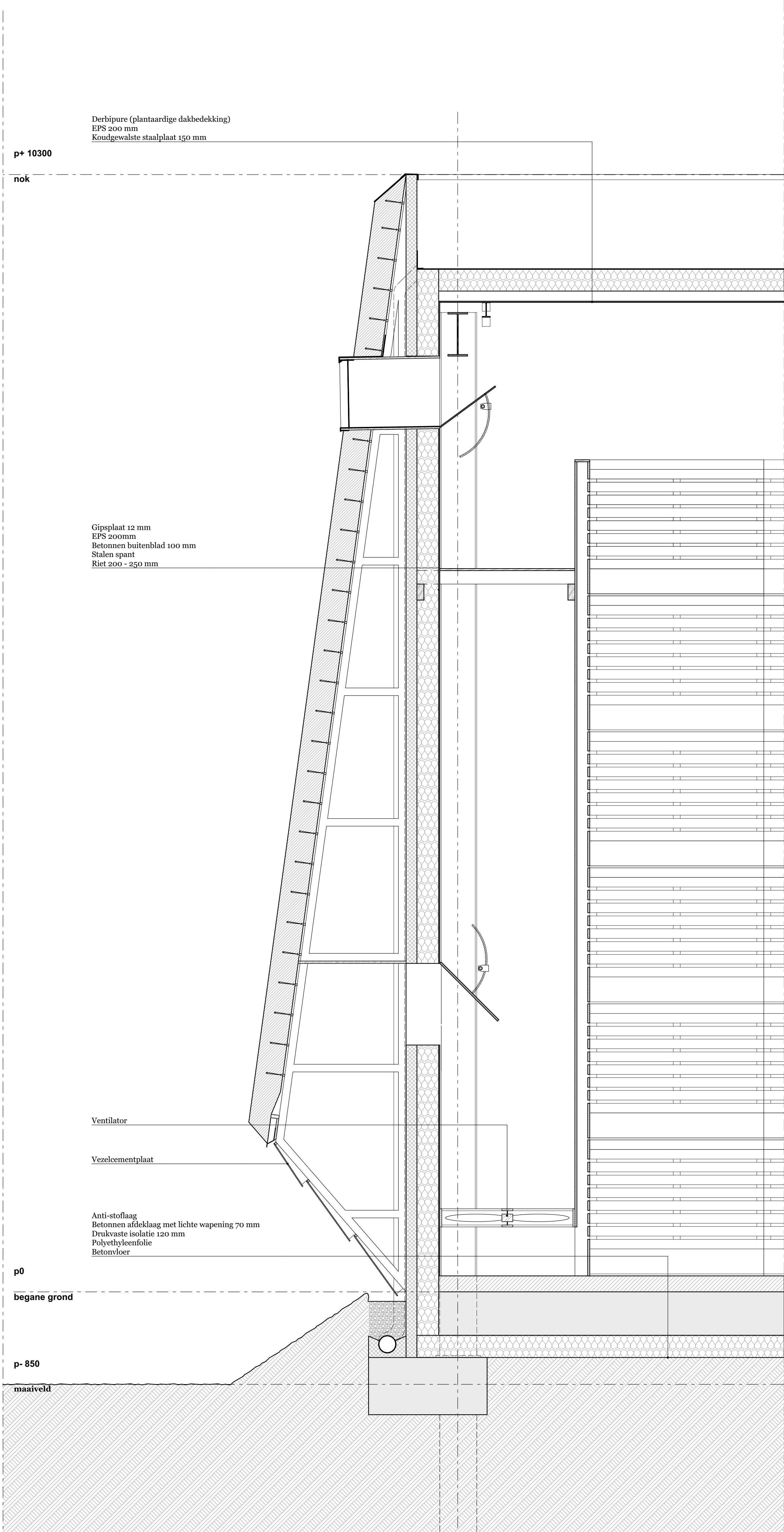
Section of Facade B Storage building 1:20
