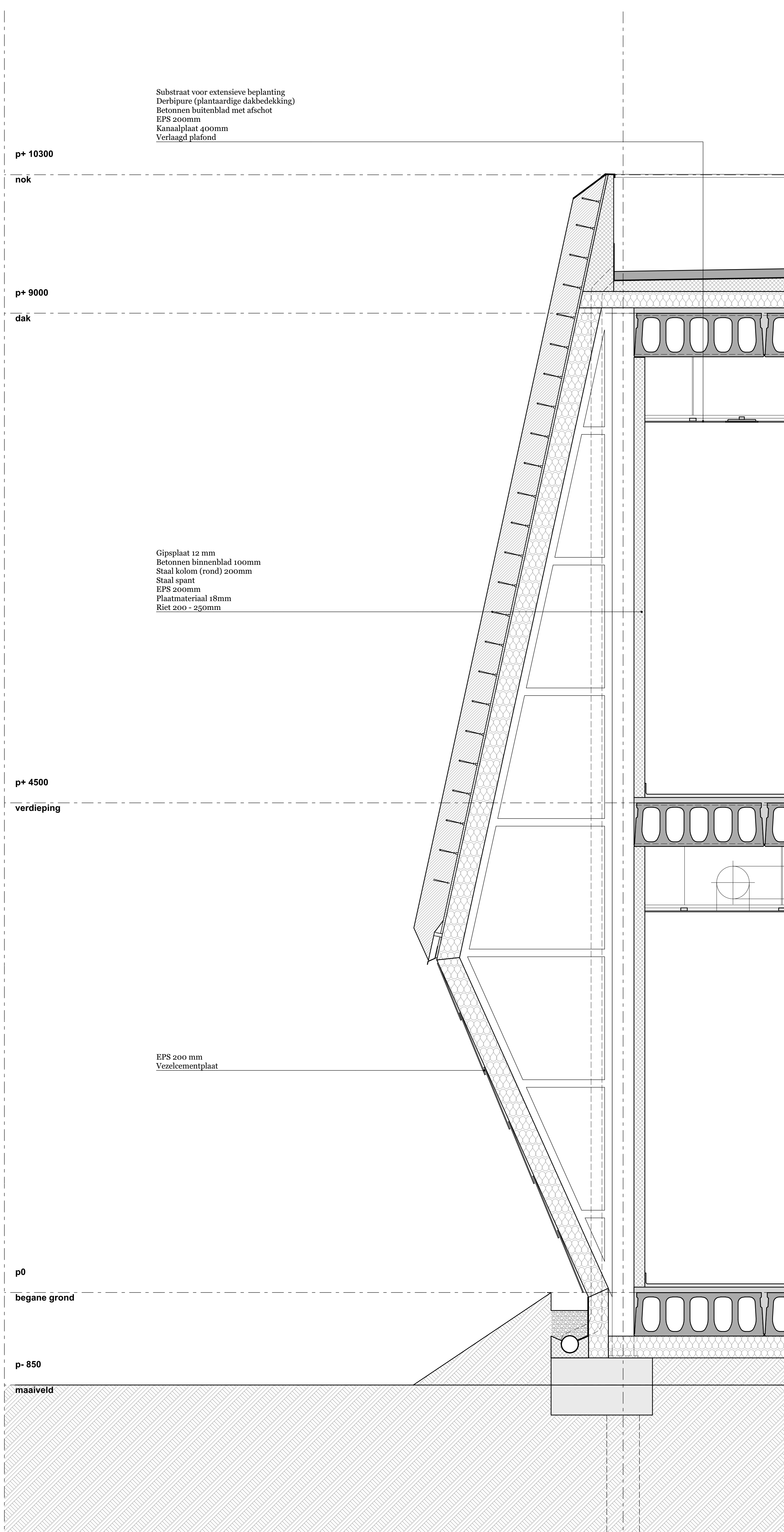
Section of Facade C Main building 1:20
