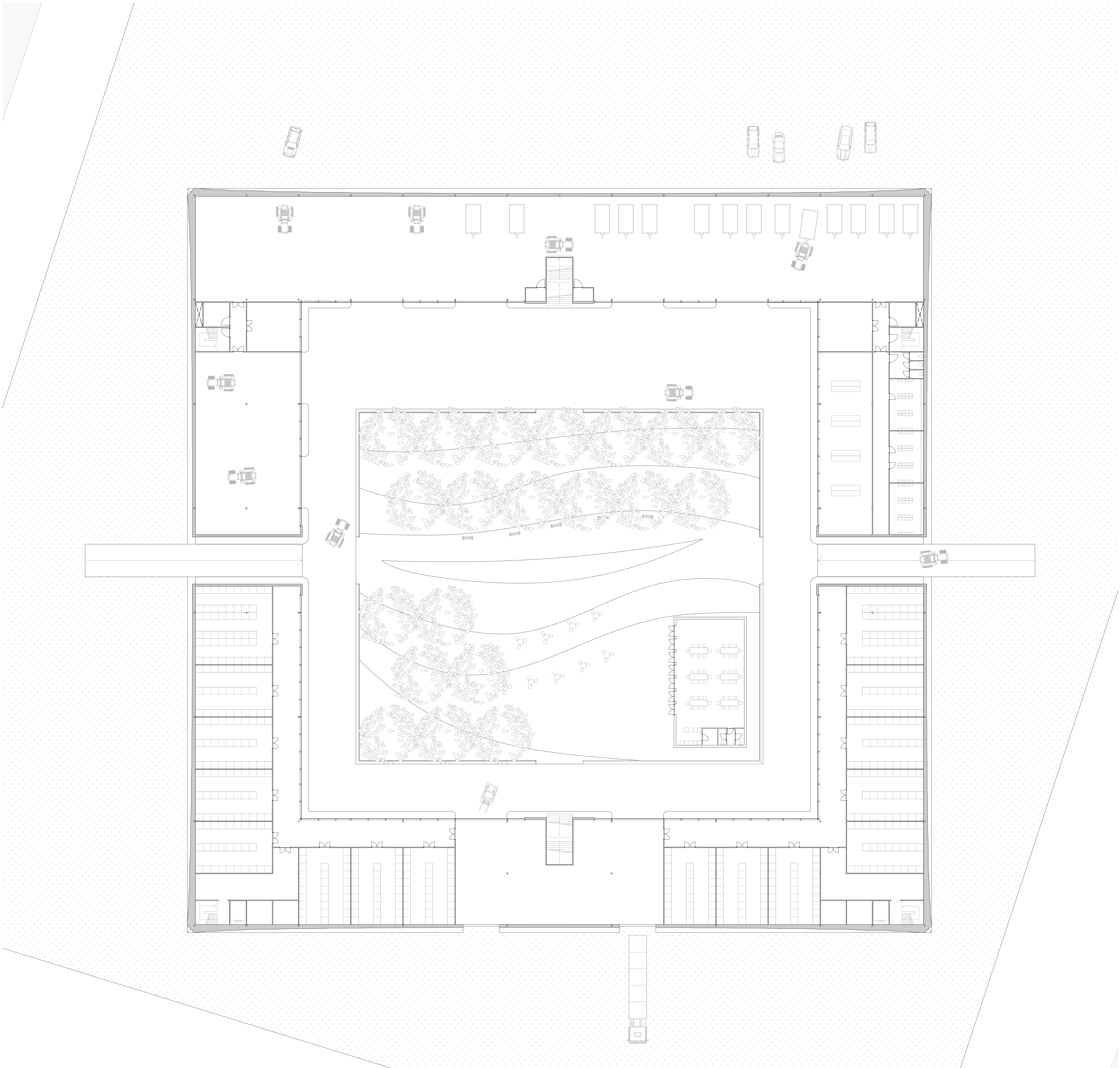
Plan Main building +0 1:200
