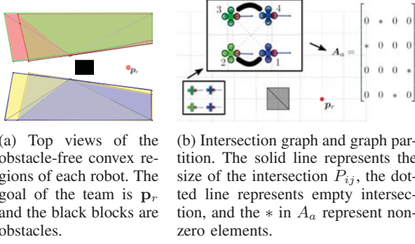
Fig. 2: Scheme of progress from the obstacle-free convex regions to the intersection graph for a team of four quadrotors.
