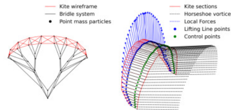
Particle system model representation (left), vortex step model discretization example (right).
