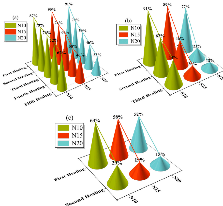
Fig. 16. Trends of FERR under cyclic "fracture-healing": (a) W2; (b) P2; (c) P4.
