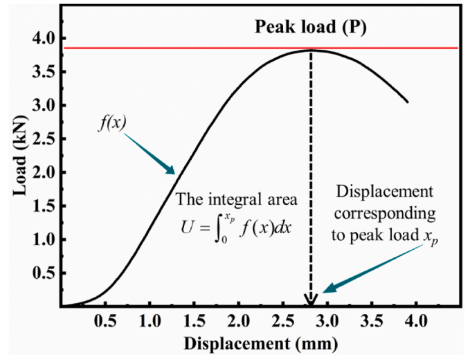
Fig. 6. SCB loading curve.
