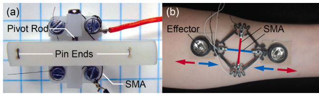
Fig. 4. (a) SMA tacter unit: two ends of the pin are fixed with a SMA and superelastic wire correspondingly. The pin can rotate around the pivot rod when the SMA is actuated, and generate pressure on skin. [62]. (b) SCWEES: working principle can be seen in of Table 2(d1) [73].
