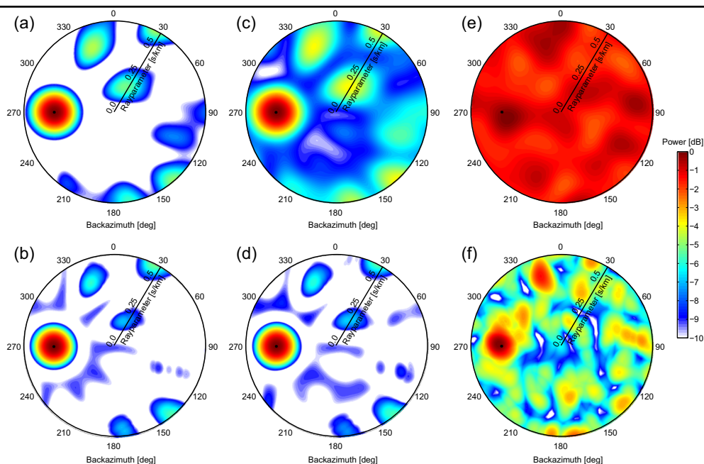
Fig. 4 A comparison of BF ( a , c , and e upper row) and CCBF ( b , d , and f lower row) with increasing levels of non-coherent noise from left to right. Synthetic data are beamformed for a continuous noise source west of the SPITS array (Fig. 1). The parameters of the induced wavefield are marked with black dots at (p_s, \theta_s) = (0.33 \text{ s/km}, 270^\circ) . The first column shows the
