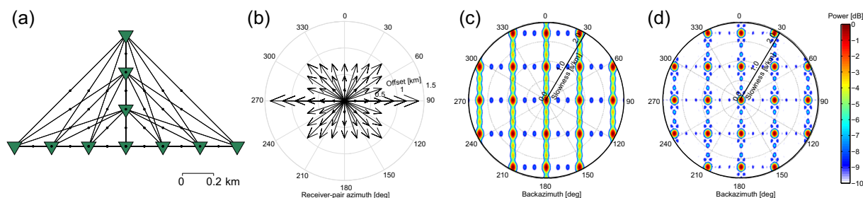
Fig. 5 Sampling and beamforming characteristics for an upside-down T-array. a Spatial configuration of the array with ten receivers (green triangles), with interconnecting lines between all receivers depicted. b Distribution plot showing the
