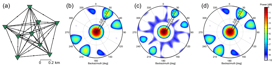
Fig. 3 a The configuration of array elements (green triangles) of the SPITS array (Fig. 1) and b–d corresponding ARFs for varying beamforming implementations, for a plane-wave source with p_S = 0 and f = 5 Hz. ARF for b conventional
