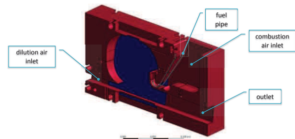
Figure 2 – Mid-plane cut-view of the 18° combustor employed in the experiments. Quartz window in blue.
