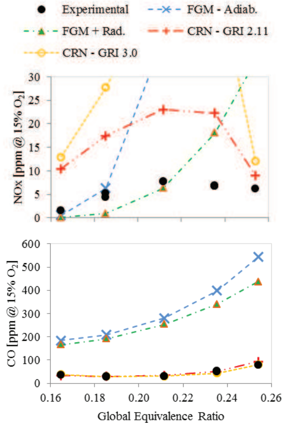
Figure 3 – NOx and CO emissions as functions of the global equivalence ratio.
