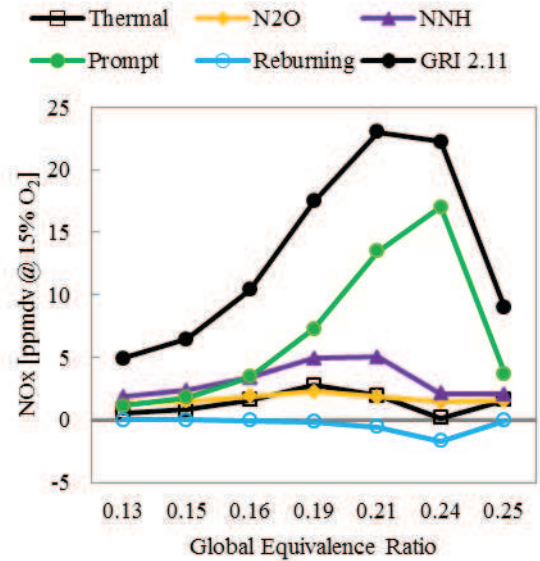
Figure 4 – Contributions of the different pathways to NOx formation according to the CRN modelling with the GRI 2.11 mechanism.
