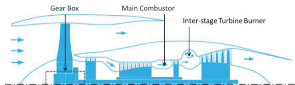
Figure 1 – Engine concept proposed along the AHEAD project 1 .
