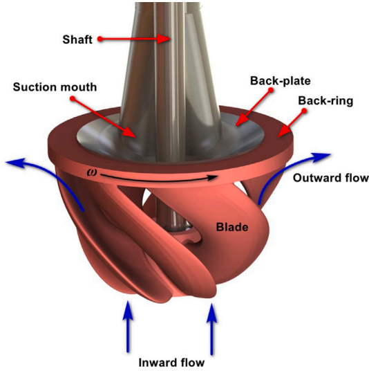
(a) Flow regime of a freely rotating cutter head (adapted from Nieuwboer (2022))
