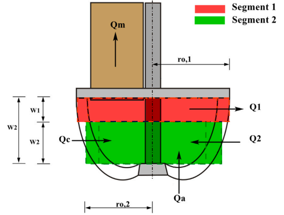
(b) Cutter head representation in the analytical spillage model of Miedema (adapted from Miedema (2019))
