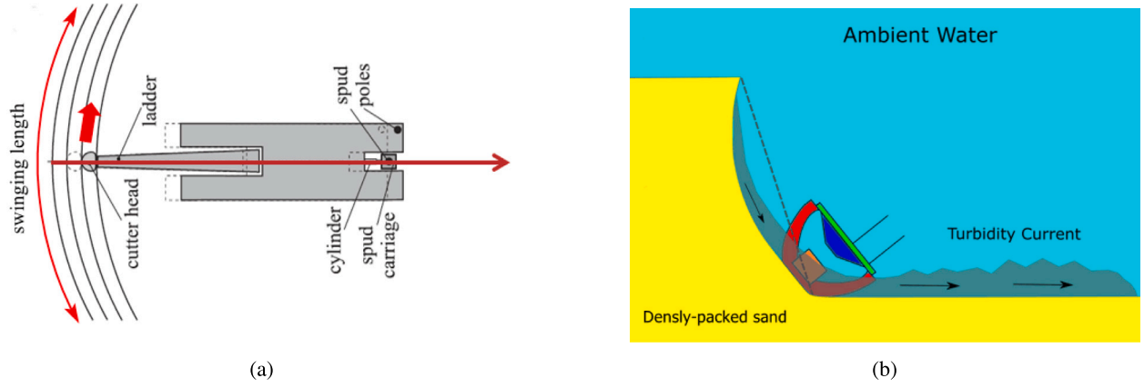
Fig. 6. Represented domain, (a) a top view of a CSD cutting and swinging along a swing path, (b) a cross-section showing the near-vertical breach generated by the cutter head and the propagation of the triggered turbidity current in the downstream.
