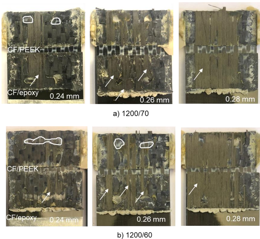
Figure 5.9: Representative matching fracture surfaces of a) 1200/70 specimens and b) 1200/60 specimens, welded at different displacement values. The 0.24 mm and 0.26 mm displacements correspond to the maximum weld strength. The highlighted areas indicate unwelded areas. The arrows point at failure in the CF/epoxy adherend.
