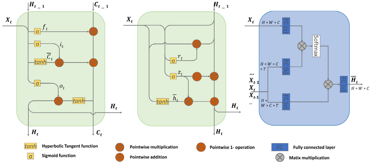
Fig. 3. Illustration of a LSTM block, a GRU block and an attention block. X_t : input feature maps; H_t : output feature maps; f_t : forget gate; i_t : input gate; o_t : output gate; \tilde{C}_t : candidate cell state; C_t : cell state; r_t : reset gate; z_t : update gate; \tilde{h}_t : candidate hidden state; H_t : hidden state; \odot : dot product; H : feature map height; W : feature map width; C : number of channels; T : number of sequential frames; q : queries; v : values; k : keys; [\dots, X_{t-1}, X_t, X_{t+1}, \dots] : context feature maps.
