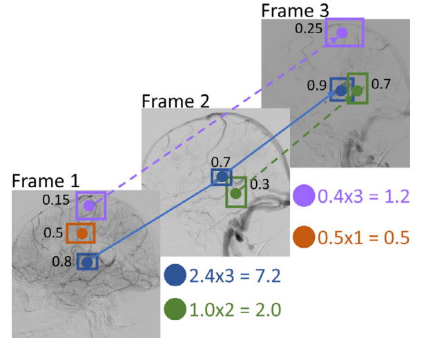
Fig. 4. Illustration of temporal consistency weighted series level bounding box optimization. Blue indicates the trajectory with the highest weighted accumulative score. The scores along the blue trajectory are then reassigned to the trajectory average score (0.8).
