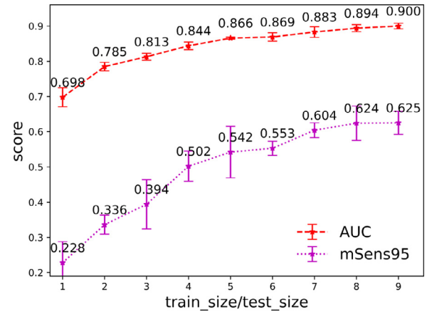
Fig. 9. Series level classification AUC and mSens 95 with respect to training/test data size ratio. mSens 95 : average sensitivity at 95% specificity over five runs.
