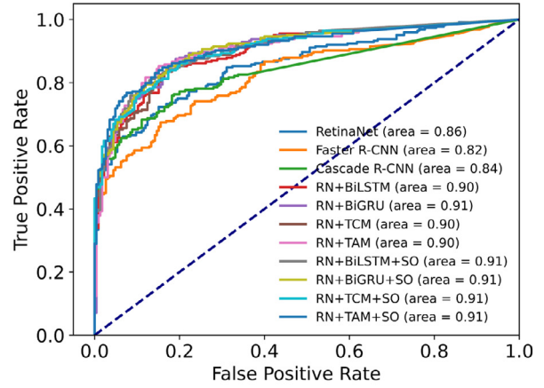
(b) ROC curve for series level perforation classification.
