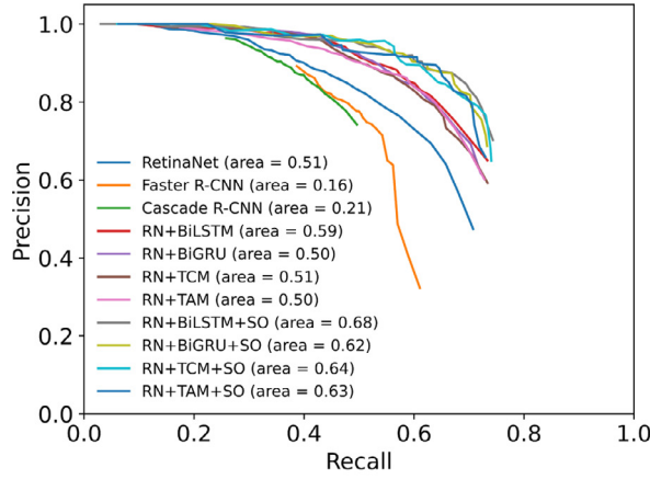
(a) Precision-recall curve for perforation localization with center overlapping metric.
