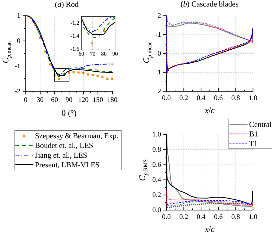
Figure 5.16: The surface pressure distribution on the rod (a) and on the cascade blades (b). Time-averaged surface pressure is normalised as pressure coefficient C_{p,mean} = (p_{mean} - p_{\infty})/q_{\infty} , where q_{\infty} = 0.5\rho_{\infty}U_{\infty}^2 . For the cascade blades, the data points at the suction side are drawn with lower opacity. In (a), the reference angle \theta = 0^\circ faces towards the upstream direction. In (b), the root-mean-square of surface pressure fluctuations is expressed as C_{p,RMS} = p_{RMS}/q_{\infty} . Reference data in (a) have been taken from Szepešsy and Bearman [26], Boudet et al. [27], and Jiang et al. [28].
