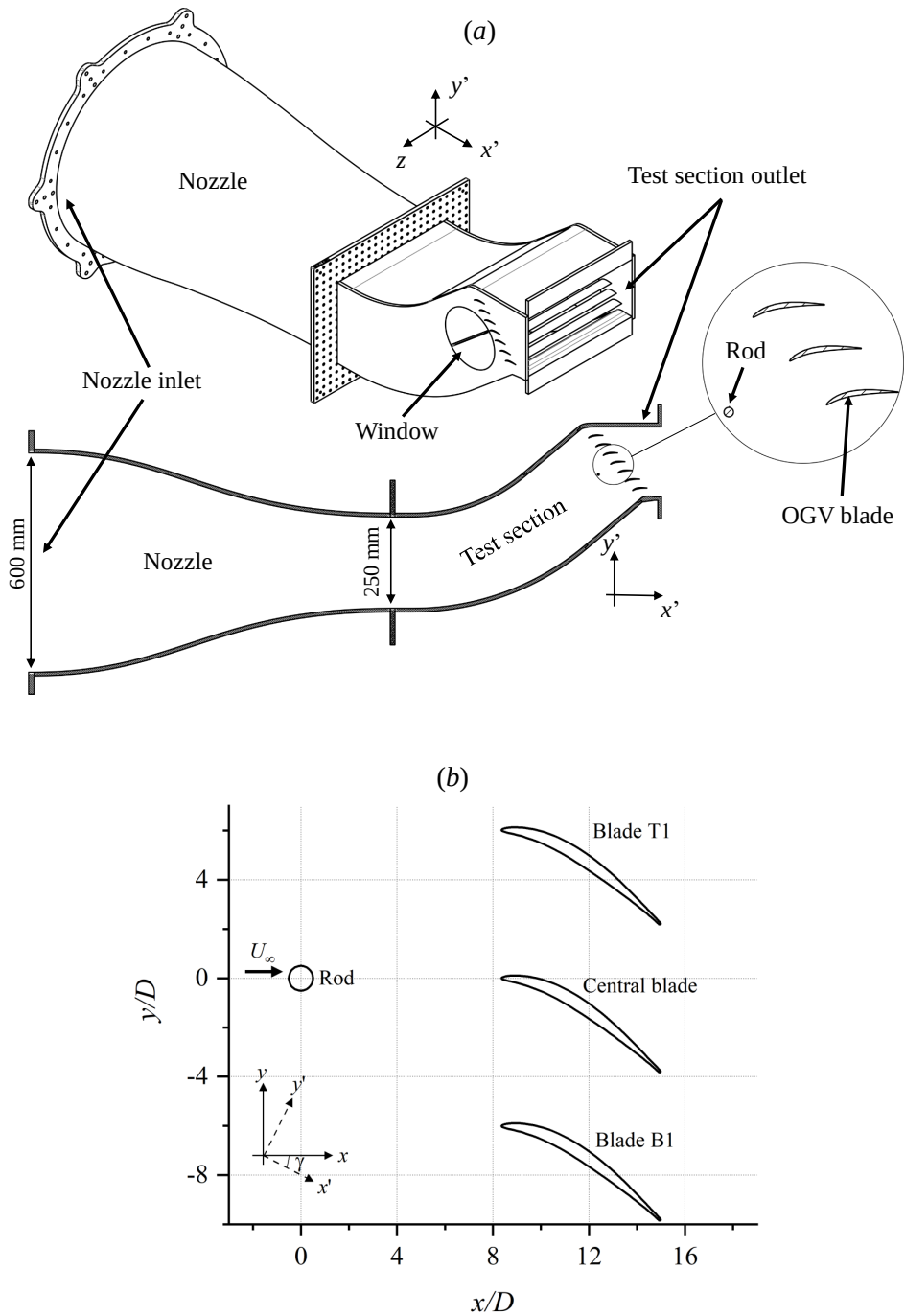
Figure 5.4: (a) A sketch of the RLC test rig revealing the rod and the OGV blade-row arrangement. (b) Closer detail of the rod-linear cascade components, showing 3 out of the 7 OGV blades.
