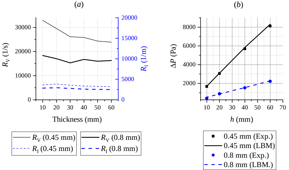
Figure 2.11: (a) Resistivity values for the Ni-Cr-Al metal-foam sample obtained from the experiment, and (b) the comparison of the pressure drop result between the experiment (Exp.) and simulation (LBM).
