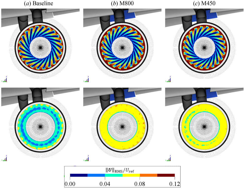
Figure 5.31: (Front view) Contours of phase-locked standard deviation of velocity magnitude \|\mathbf{U}_{\text{RMS}}\| at the SDT interstage (top row) and outlet (bottom row).
