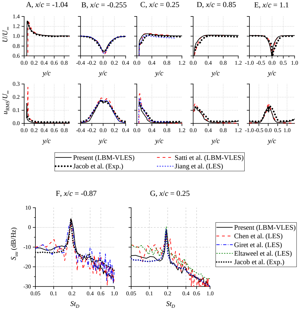
Figure 4.7: The upper row shows the profiles of mean ( U ) and root-mean-square (RMS) ( u_{\text{RMS}} ) of fluctuations of the streamwise velocity component at different locations along the rod-airfoil configuration. The lower row shows the power spectral density of streamwise velocity fluctuations S_{uu} at points (F) ( x/c = -0.87 , y/c = 0.05 ) and (G) ( x/c = 0.25 , y/c = 0.08 ), normalized with a reference velocity of 1 m/s. Current simulation results are compared against those from Jacob et al. [40] (experiment), Satti et al. [54] (LBM-VLES), Jiang et al. [55] (LES), Chen et al. [44] (LES), Giret et al. [56] (LES), and Eltaweel and Wang [57] (LES).
