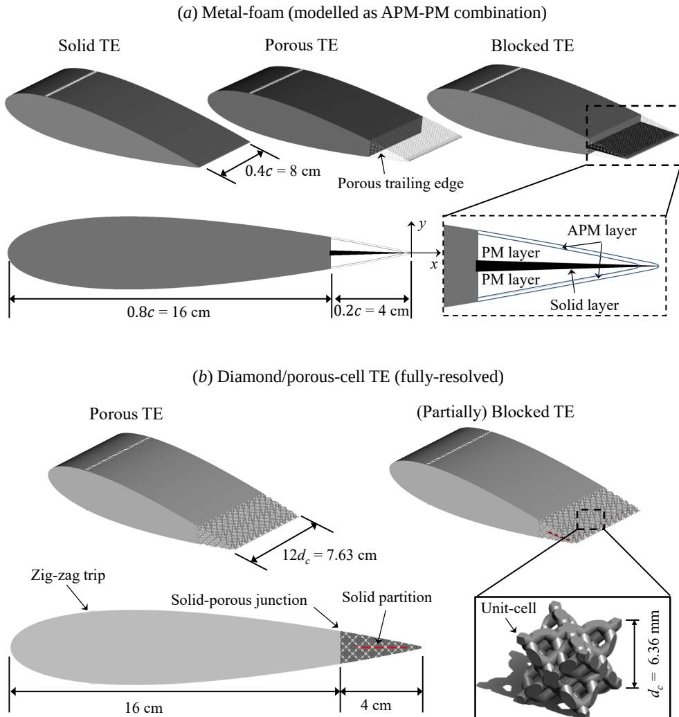
Figure 3.4: The NACA 0018 with three different trailing edge (TE) configurations. The side view of the blocked TE is shown at the bottom left, where an inset shows the internal arrangement of the trailing-edge region of the blocked TE.
