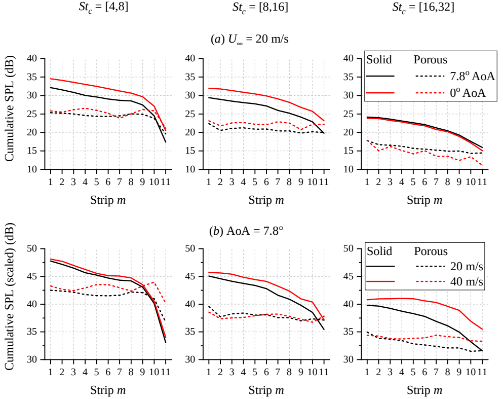
Figure 3.22: (Metal foam/modelled) The cumulative sum of noise contribution from different strips. The effect of AoA for the 20 m/s cases is shown in (a). In (b), the values at 20 m/s has been scaled to match that at 40 m/s following U_\infty^5 for solid TE and U_\infty^{5.7} for porous TE respectively.
