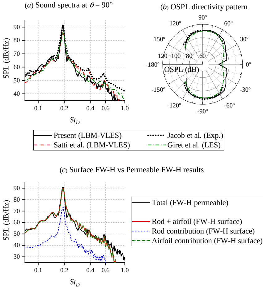
Figure 4.10: (a) Sound spectra in the far-field, computed at a location directly above the airfoil LE ( \theta = 90^\circ , i.e., x/c = 0 and y/c = 18.5 ) and (b) OSPL directivity pattern with zero degree reference towards the downstream direction. Plot (c) shows the far-field noise contribution of the rod, the airfoil, and both combined using the surface FW-H approach in comparison with that from the permeable FW-H approach.
