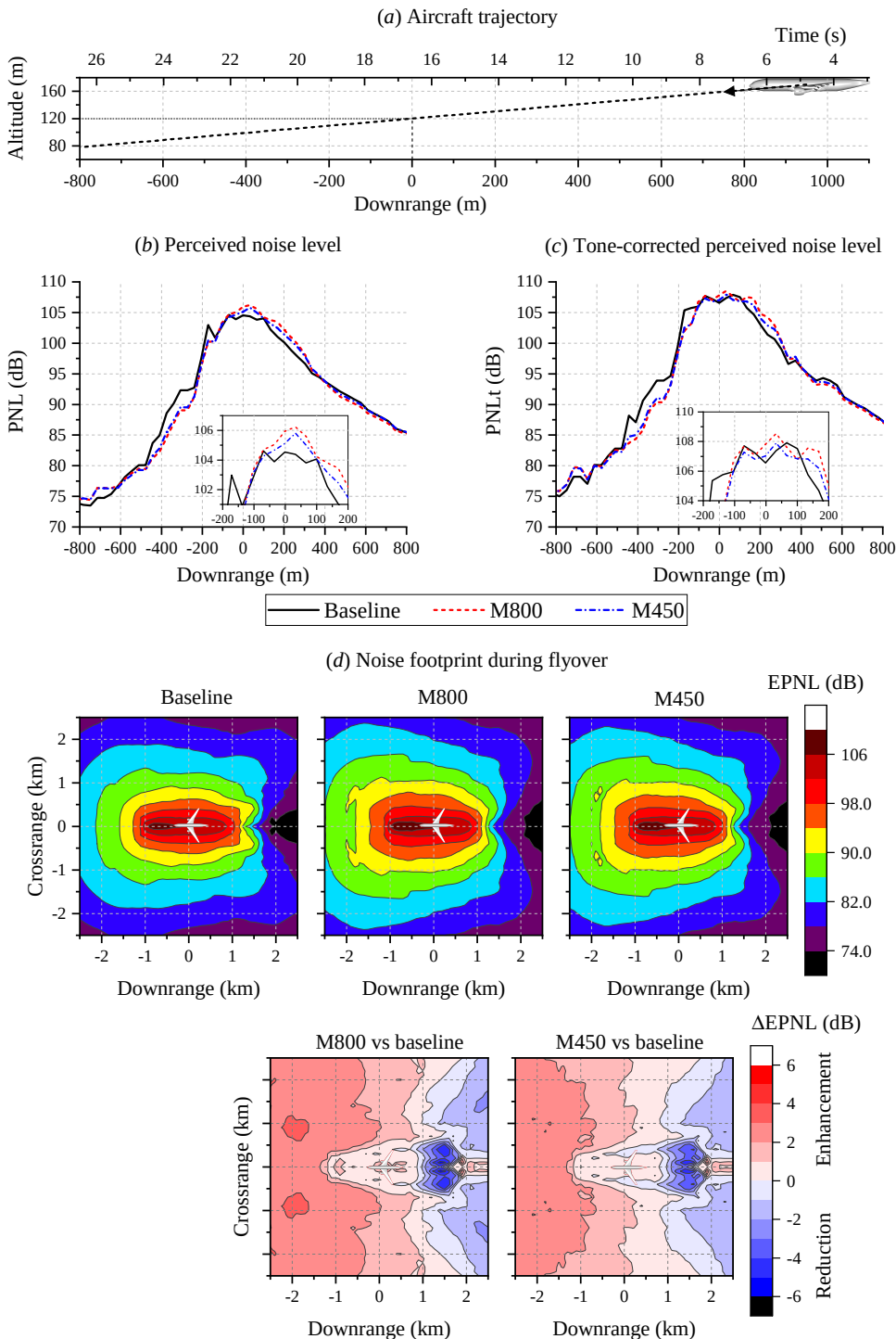
Figure 5.38: (a) The aircraft trajectory for noise footprint analysis. (b) The variation of perceived noise level (PNL) and (c) the tone-corrected PNL (PNLt) for a reference aircraft approach scenario. The noise footprints during the flyover are given in (d). The reference flyover microphone is located at the origin of the downrange axis, where the aircraft altitude is 120 m.
