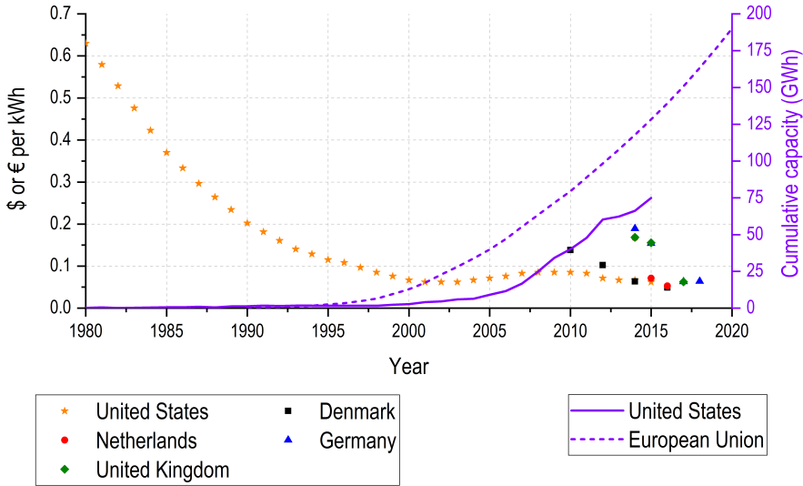
Figure 1.4: The trend of cost per unit of wind electricity and the cumulative capacity of wind energy across the global north [24, 30].
