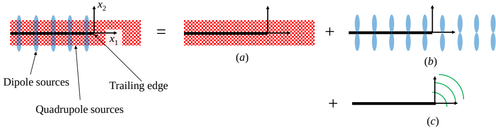
Figure 3.2: The distributions of dipole and quadrupole sources representing Amiet's solution to the TE noise problem. (a) and (b) show the quadrupole and dipole distributions that extend in both upstream and downstream directions, and (c) is the scattered acoustic pressure.
