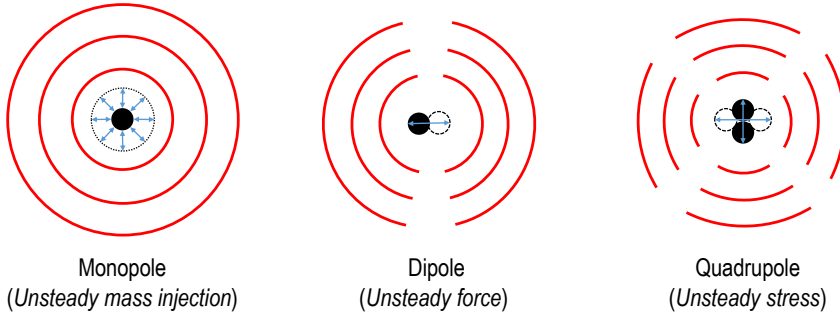
Figure 2.6: An illustration of different types of elementary acoustic sources in linear acoustic theory. The directivity for each source can be inferred from the wave propagation pattern.
