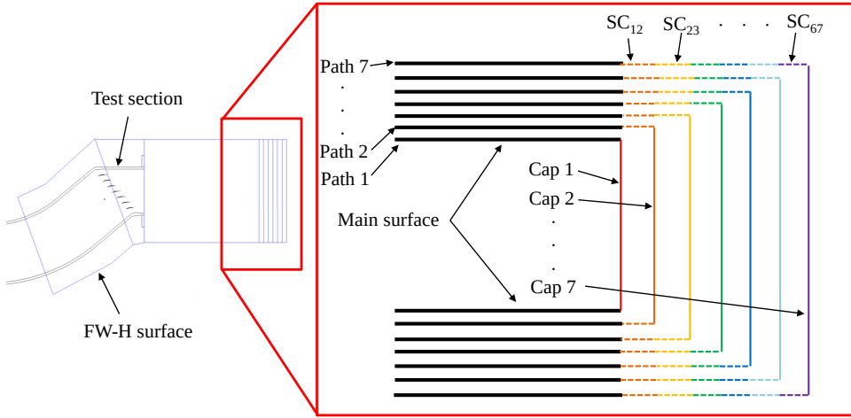
Figure 5.7: The nomenclature of integration paths on the FW-H permeable surface with cap and connector surfaces.
