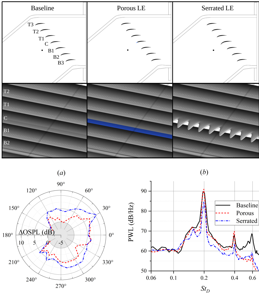
Figure 5.20: The upper half shows the computer drawings of the RLC configurations, including those with porous and serrated LE. The lower half shows (a) the noise reduction directivity pattern given as \Delta\text{OSPL} = \text{OSPL}_{\text{baseline}} - \text{OSPL}_{\text{porous, serrated}} , and (b) the comparison of the sound power level.
