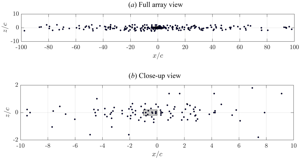
Figure 3.16: The distribution of 320 microphones in a modified Underbrink [74] configuration. The grey area represents the planform of the airfoil with the flow towards the positive x direction. The source maps are shown in figure 3.17.
