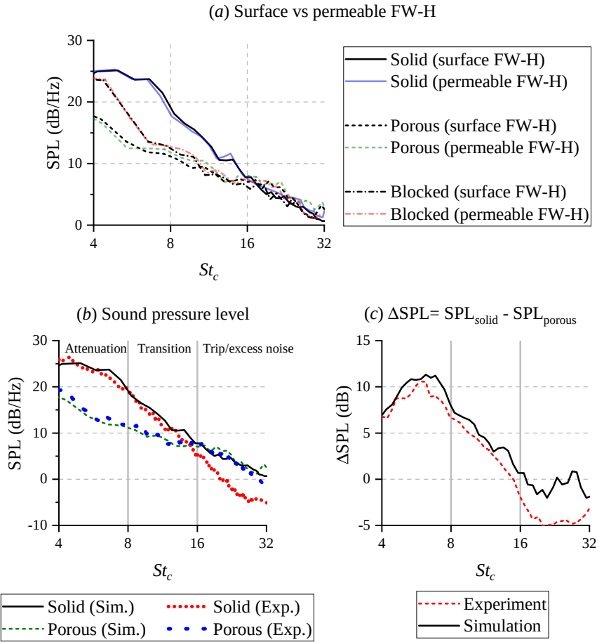
Figure 3.12: (Porous cell) Plot (a) shows the comparison between far-field noise spectra obtained using the FW-H analogy applied on the surface pressure fluctuations (surface FW-H), and that from the permeable surface (permeable FW-H) enclosing the airfoil. The far-field noise level and the noise reduction level are validated in plots (b) and (c). Observer location is at x/c = 0 , y/c = 5 .
