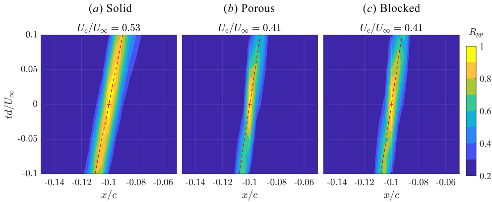
Figure 3.42: (Porous cell/fully-resolved) Contours of spatio-temporal correlation coefficient of surface pressure fluctuations R_{pp} . The reference location is at x/c = -0.1 , marked by the red cross at the center of each contour. The gradient that corresponds to the convection velocity U_c is plotted as red dashed-line.
