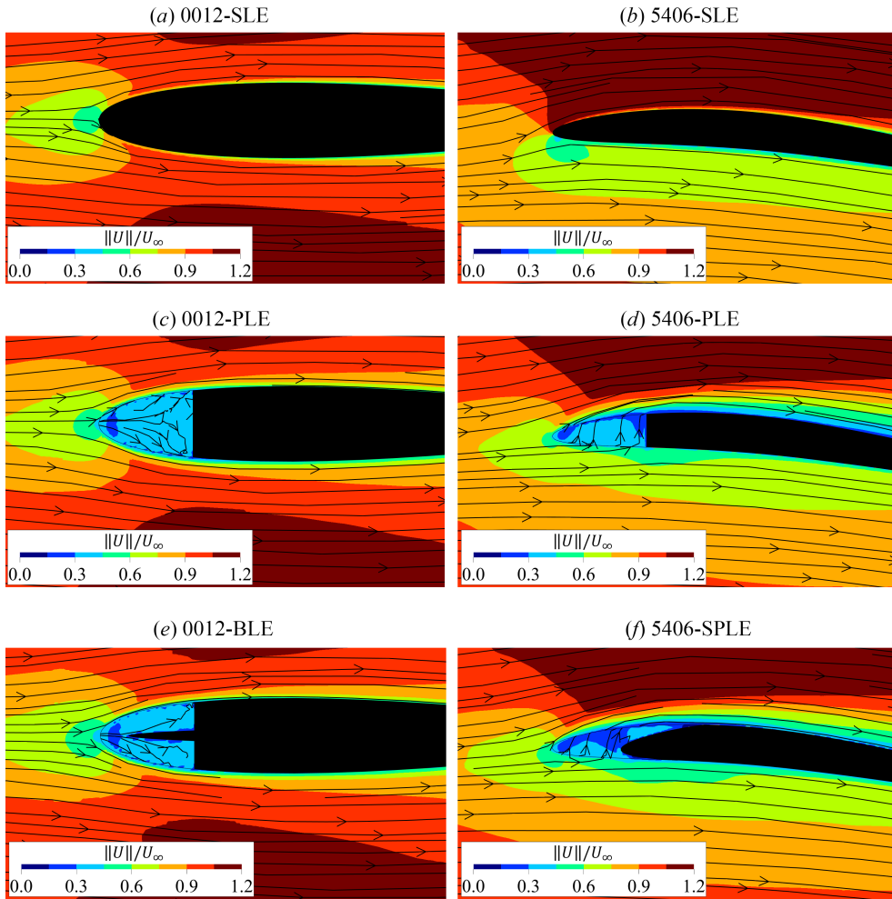
Figure 4.24: Pathline plots and contours of time-averaged velocity magnitude \|U\|/U_\infty at the midspan of airfoils with porous LE (c to f) in comparison to the SLE (a to b). Note that some pathlines may enter or leave the sampling plane in the direction normal to this page.
