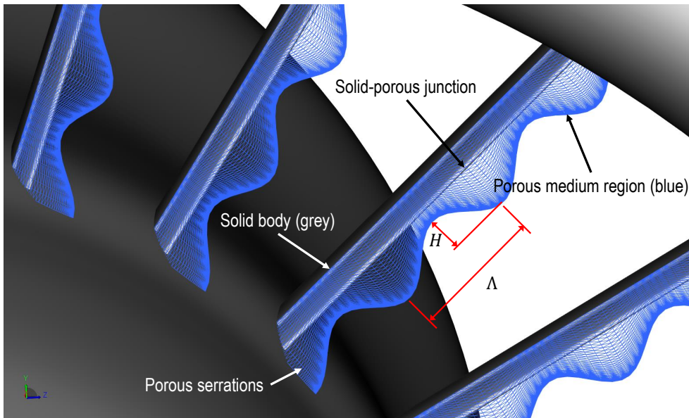
Figure 5.25: A closer view on the modified OGV in the fan stage, highlighting the amplitude H and wavelength \Lambda of the serration planform.
