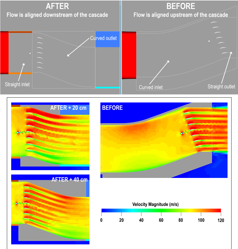
Figure 5.3: A comparison of the model arrangement and flow field inside the test section between a setup with flow turning downstream (AFTER) and upstream (BEFORE) of the cascade. The velocity magnitude contours have been obtained using PowerFLOW simulations with a coarse grid resolution level.
