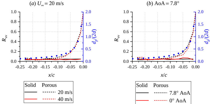
Figure 3.41: (Metal foam/ modelled) The correlation coefficients of vertical velocity fluctuations ( R_{vv} ) between the suction and pressure sides of the porous TE. The secondary vertical axis (in blue) shows the ratio between the mean pore diameter of the metal-foam ( d_p ) and the local airfoil thickness ( 2d ).
