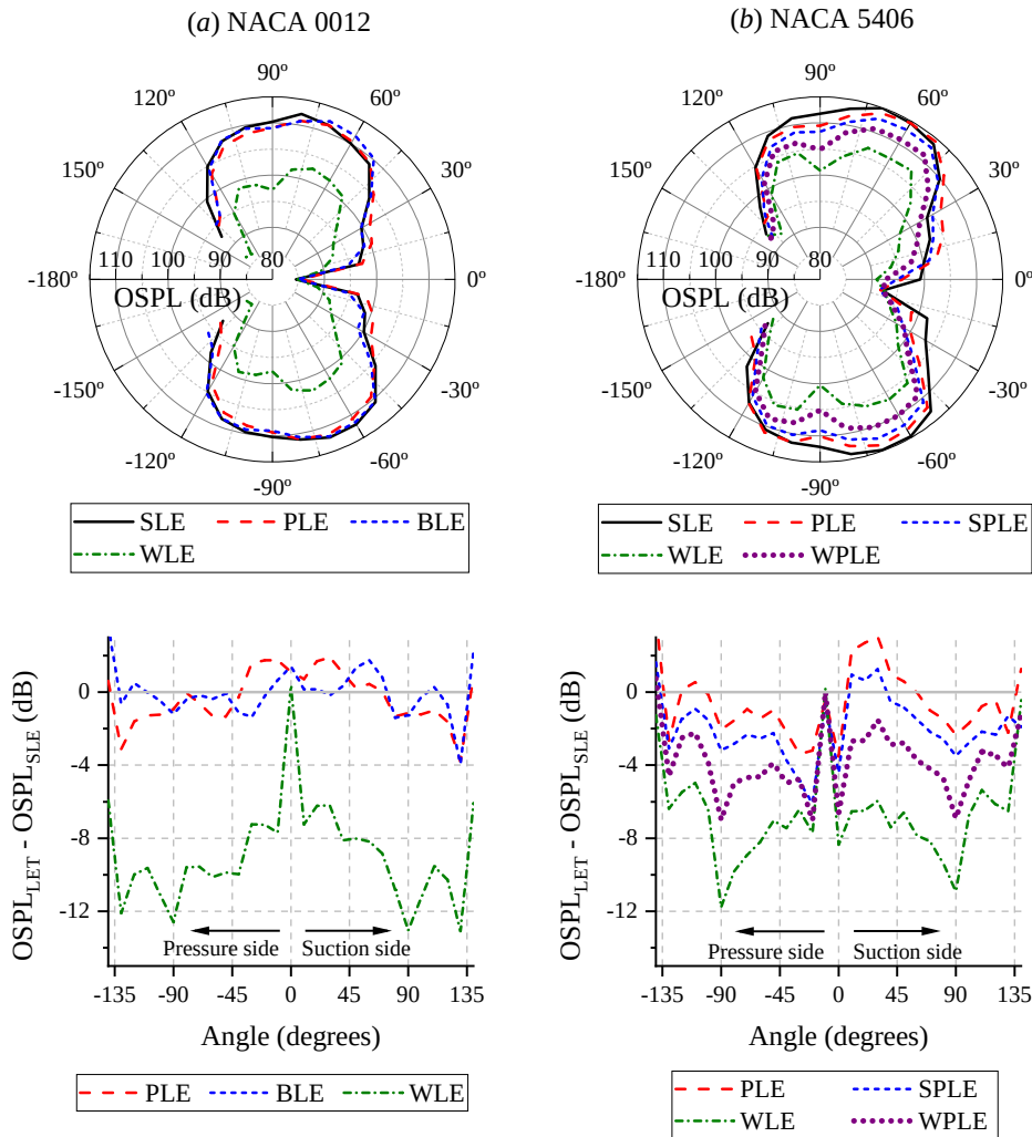
Figure 4.14: The comparison of the far-field noise directivity pattern for the different LE treatments is given at the upper row. The lower row shows the OSPL difference between the LET cases and the baseline.
