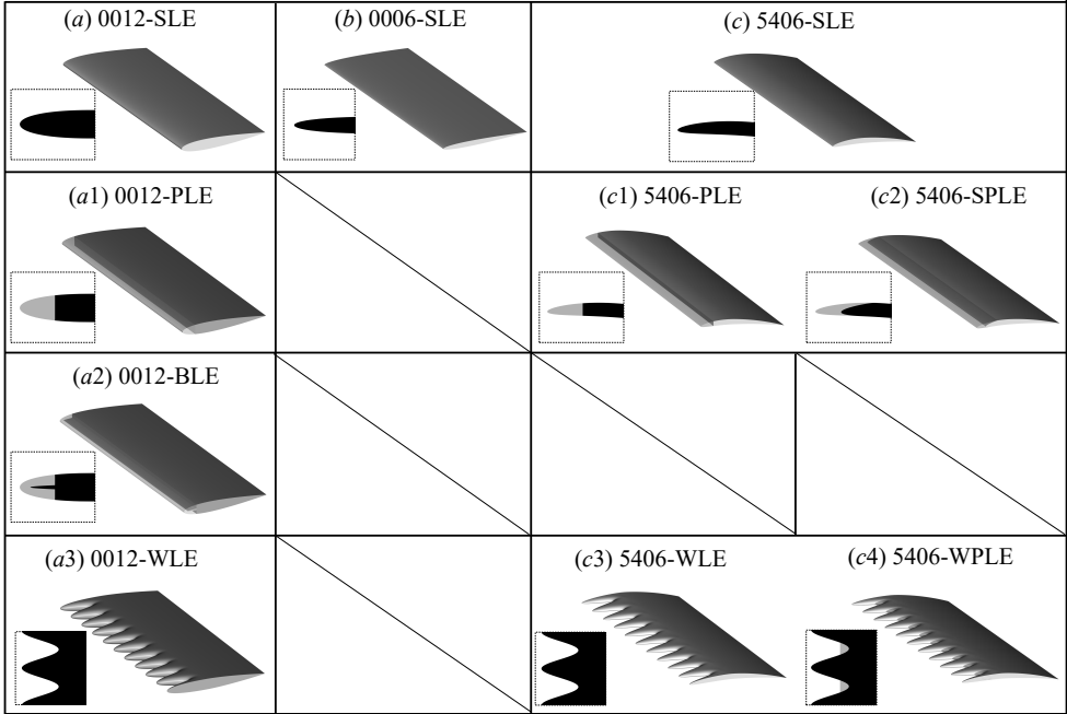
Figure 4.4: The types of airfoil and leading-edge treatments; SLE (straight-LE), PLE (porous-LE), SPLE (streamlined porous-LE), BLE (blocked porous-LE), WLE (serrated/wavy-LE), WPLE (serrations-porous-LE). The porous section of the airfoil is shown with lower opacity. Insets provide the zoomed-in lateral view at the LE. Note that for the insets of WLE/WPLE configurations, the top-down view is shown instead.
