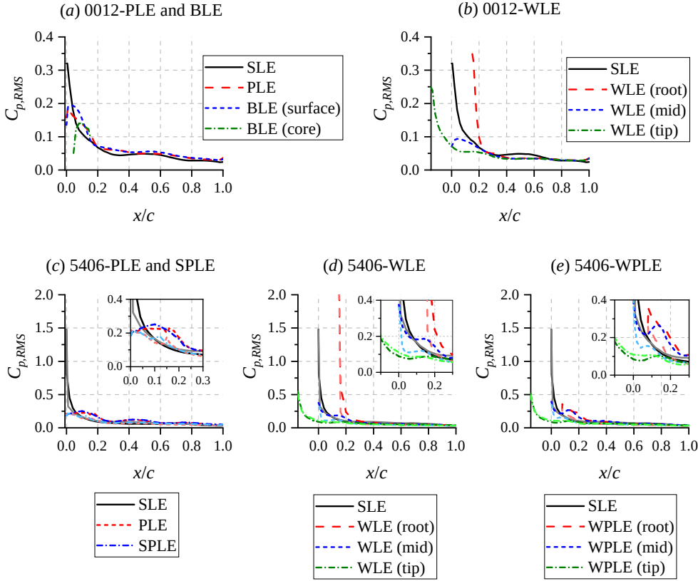
Figure 4.18: Root-mean-square of surface pressure fluctuations C_{p,RMS} = p_{RMS}/0.5\rho_\infty U_\infty^2 distribution along the airfoil chord. For the 5406 airfoils, the values on the pressure side are plotted using lighter colour.
