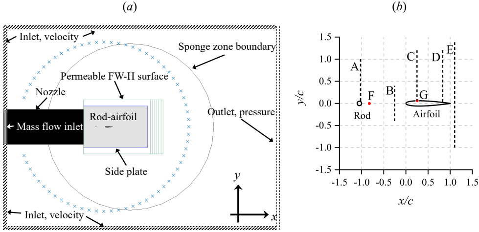
Figure 4.6: (a) Side view of the simulation domain for the rod-airfoil configuration; the outer boundaries are not drawn to scale. Blue crosses indicate microphone locations for far-field noise computation. A closer view on the baseline rod-NACA 0012 configuration (0012-SLE) is provided on the right (b). Vertical dashed lines indicate the locations where the velocity statistics are sampled and shown in figure 4.7.
