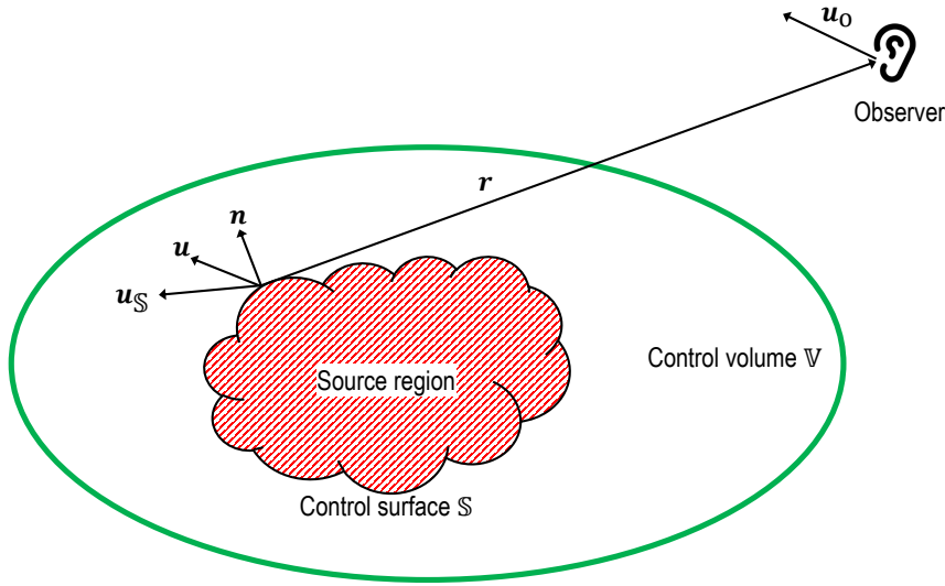
Figure 2.5: A schematic of the notations used in the formulation of the Ffowcs-Williams & Hawkins (FW-H) analogy. The source region \mathbb{V} is enclosed by a control surface \mathbb{S} . Vectors \mathbf{u} and \mathbf{v} refer to the flow velocity and the velocity of the control surface respectively. \mathbf{u}_o is the velocity of the observer.
