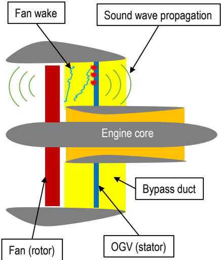
Rotor-stator interaction in a high-bypass turbofan (side view)
