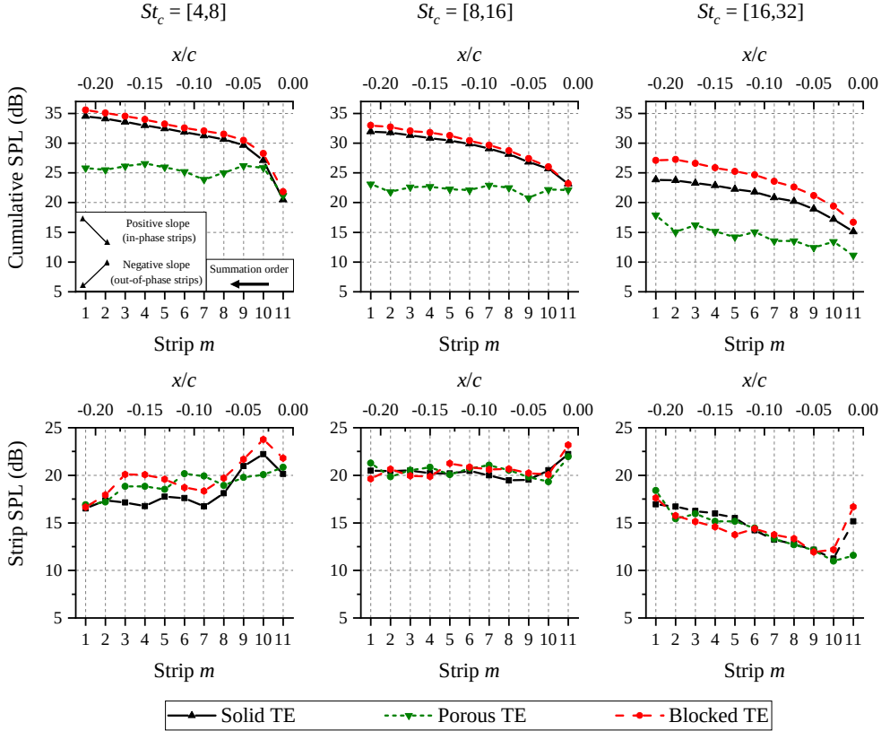
Figure 3.21: (Metal foam/modelled) The sound pressure level (SPL) produced by each strip and its cumulative, integrated over 3 different frequency bands. Note that the cumulative SPL is computed following a descending order (i.e., starting from strip 11).
