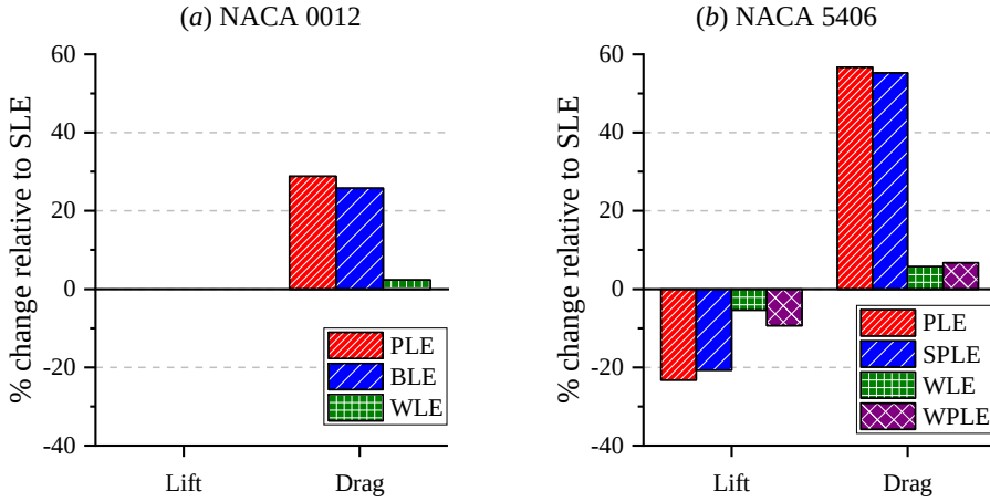
Figure 4.26: Time-averaged aerodynamic forces of the airfoils with LE treatments expressed in term of the relative difference to those of the baseline configurations (SLE).
