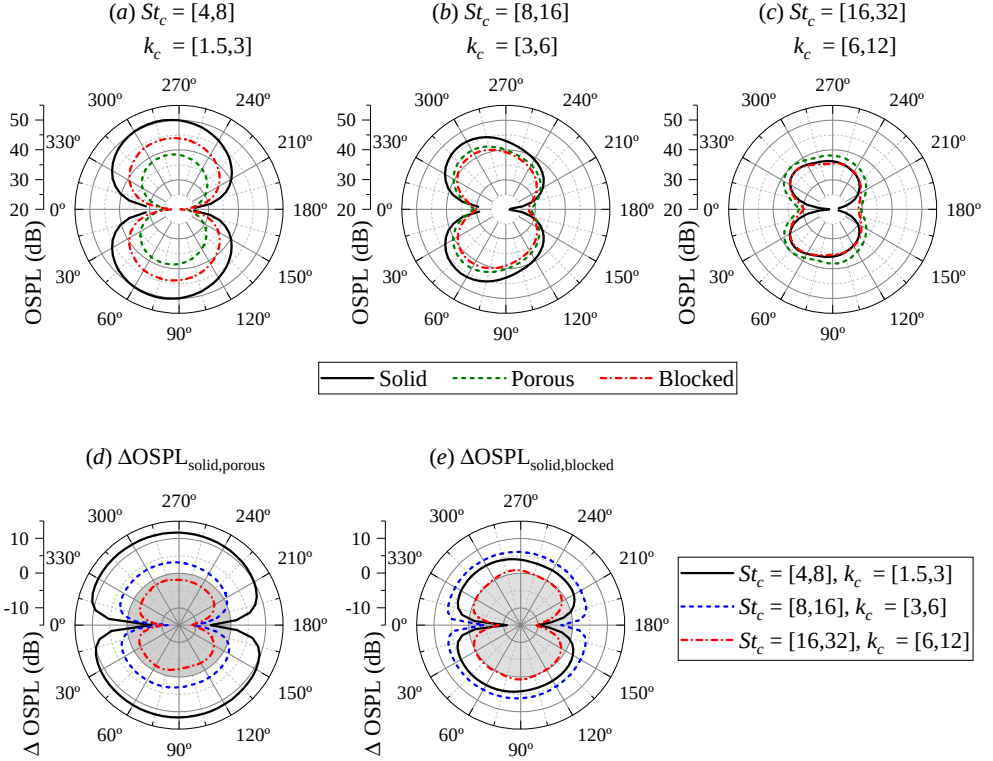
Figure 3.15: (Porous cell/full-resolved) Far-field noise directivity for solid and porous TE cases, plotted as the overall sound pressure level (OSPL) integrated over three different frequency ranges (a) 4 < St_c < 8 , (b) 8 < St_c < 16 , and (c) 16 < St_c < 32 . The OSPL difference relative to the solid TE is plotted in (d) and (e);
