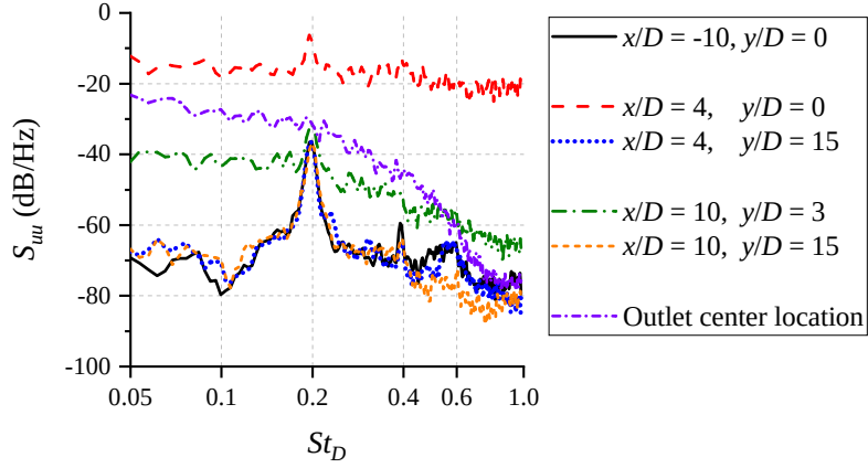
Figure 5.14: Power spectral density of streamwise velocity fluctuations S_{uu} at the midspan of the test section. S_{uu} has been normalised with a reference velocity of 1 m/s.
