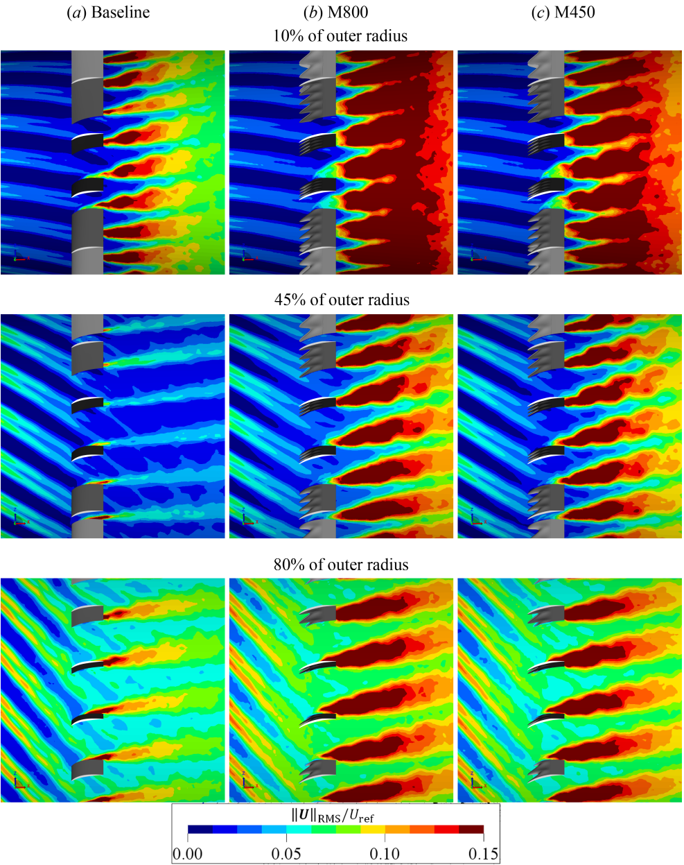
Figure 5.32: (Side view) Contours of phase-locked standard deviation of velocity magnitude \|U_{\text{RMS}}\| at the different radial sections in the fan stage.
