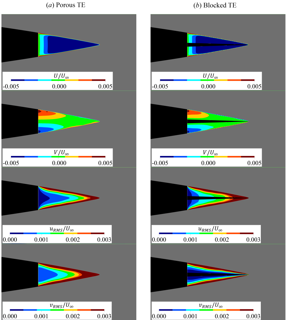
Figure 3.28: (Metal foam/modelled) Contours of velocity statistics in the porous-medium region of porous and blocked TE normalised with U_\infty ; the mean velocity components in x ( U ) and y directions ( V ) are in the first and second rows respectively, and the corresponding root-mean-square of velocity fluctuations ( u_{RMS} and v_{RMS} ) are in the third and fourth rows respectively. Regions outside of the porous medium are masked in grey.
