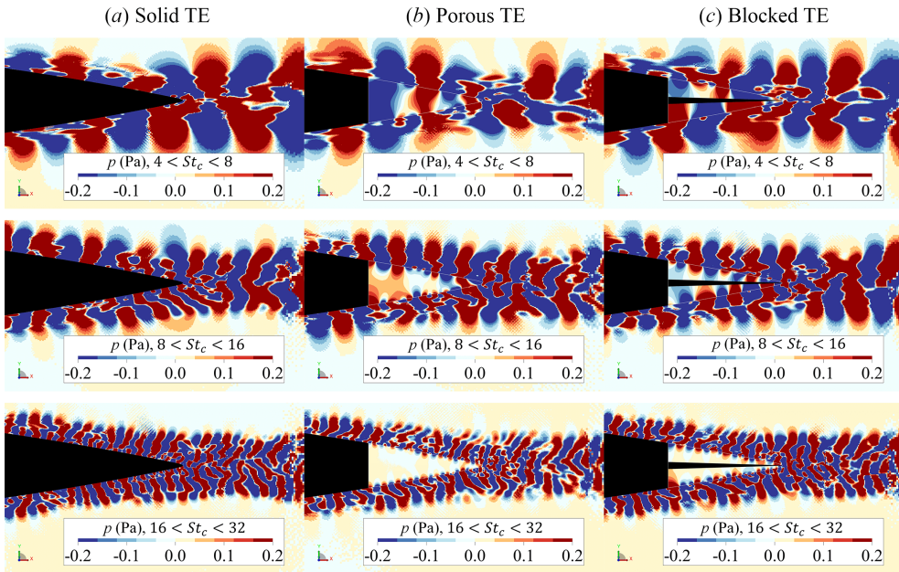
Figure 3.37: (Metal foam/modelled) Instantaneous contours of band-passed pressure fluctuations ( p' ) at the mid-span of the three trailing edge treatments at different frequency bands, i.e., 4 < St_c < 8 at the top row, 8 < St_c < 16 at the middle, and 16 < St_c < 32 at the bottom.
