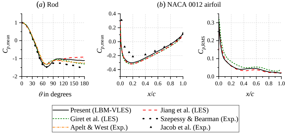
Figure 4.8: Validation of surface pressure statistics on the rod and the 0012-SLE airfoil. Time-averaged surface pressure is normalised as pressure coefficient C_{p,\text{mean}} = (p_{\text{mean}} - p_{\infty})/q_{\infty} , where q_{\infty} = 0.5\rho_{\infty}U_{\infty}^2 . In (a), the reference angle \theta = 0 faces towards the inflow direction. In (b), the root-mean-square of surface pressure fluctuations is expressed as C_{p,\text{RMS}} = p_{\text{RMS}}/q_{\infty} . Additional experimental data for the rod C_{p,\text{mean}} have been taken from Apelt et al. [59] and Szepessy and Bearman [60].
