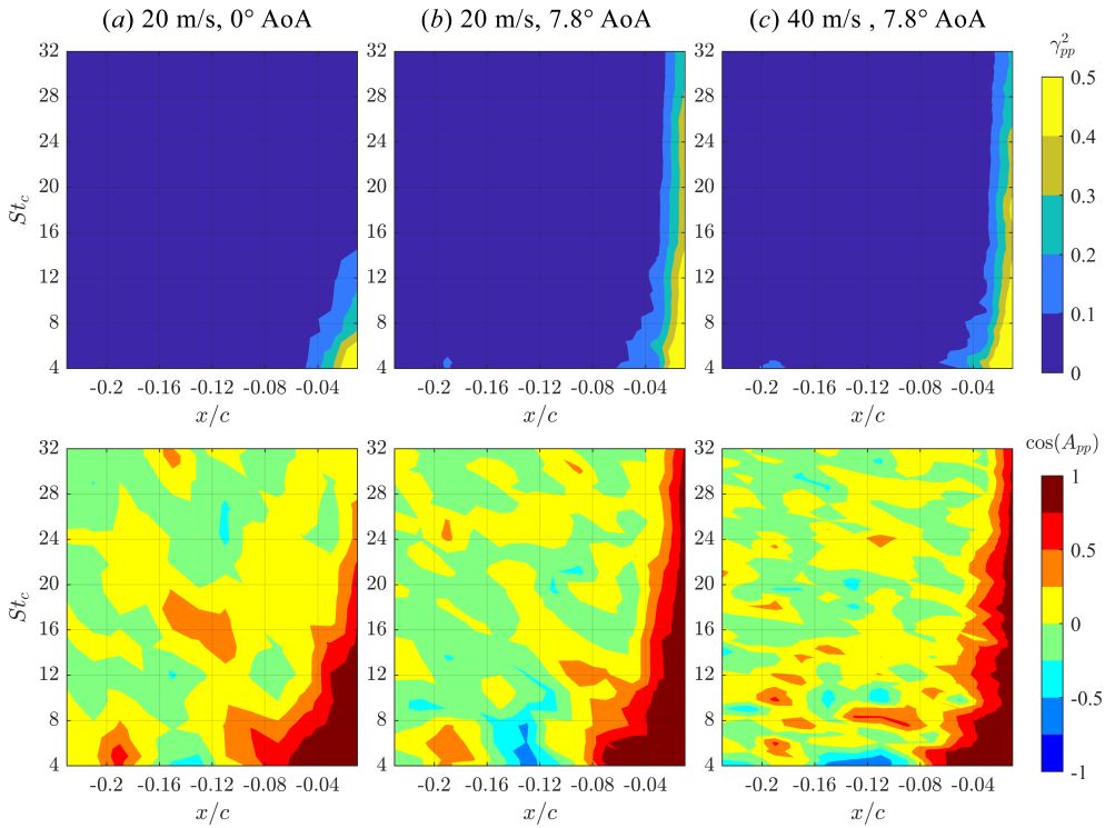
Figure 3.40: (Metal foam/modelled) The spatial distribution of magnitude-squared coherence of surface pressure fluctuations \gamma_{pp}^2 at the airfoil surface and the corresponding phase angle A_{pp} between the suction and pressure sides.
