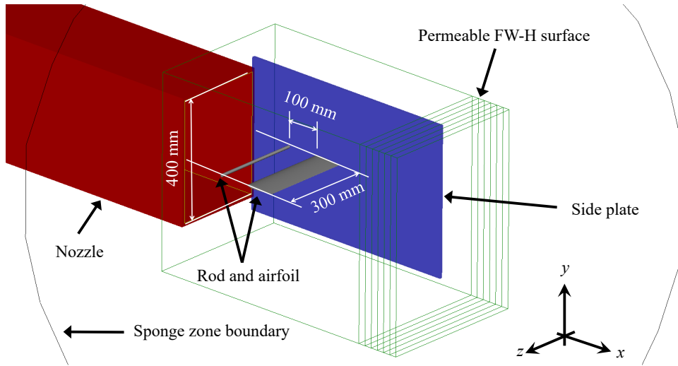
Figure 4.3: An isometric view of the rod-airfoil simulation setup. One of the side plate has been hidden from view. The outer black circular boundary delimits the sponge region.
