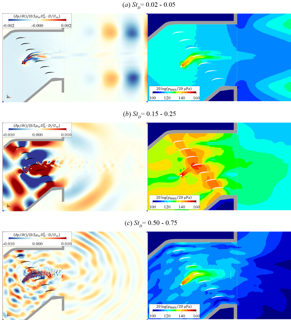
Figure 5.18: Bandpass-filtered contours of instantaneous dilatation field as time derivative of pressure \frac{\partial p}{\partial t} (left column) and the near-field pressure fluctuations p_{RMS} in decibel scale (right column).
