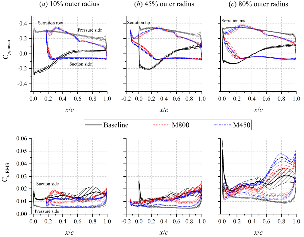
Figure 5.34: Plots of (top row) time-averaged surface pressure coefficient and (middle row) RMS of surface pressure fluctuations. The pressure distributions at the pressure side are plotted with lower opacity. The standard deviation of the pressure distributions on the different OGV blades is indicated by the shaded region.
