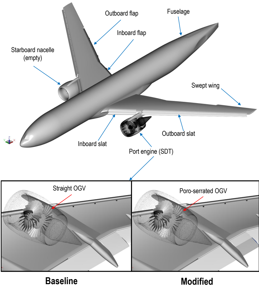
Figure 5.24: The NASA-CRM/SDT configuration in the present study. The lower part of the figures shows a comparison between the baseline configuration and another with porous treatments.
