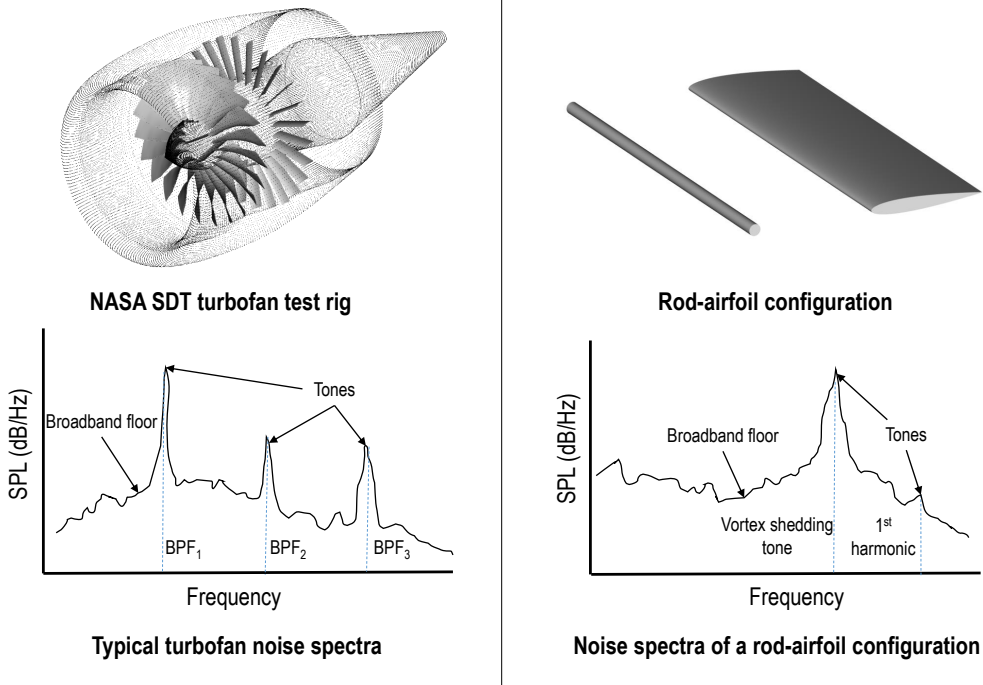
Figure 4.2: A comparison of typical noise spectra between a turbofan and a rod-airfoil configuration. BPF: blade-passing frequency.
