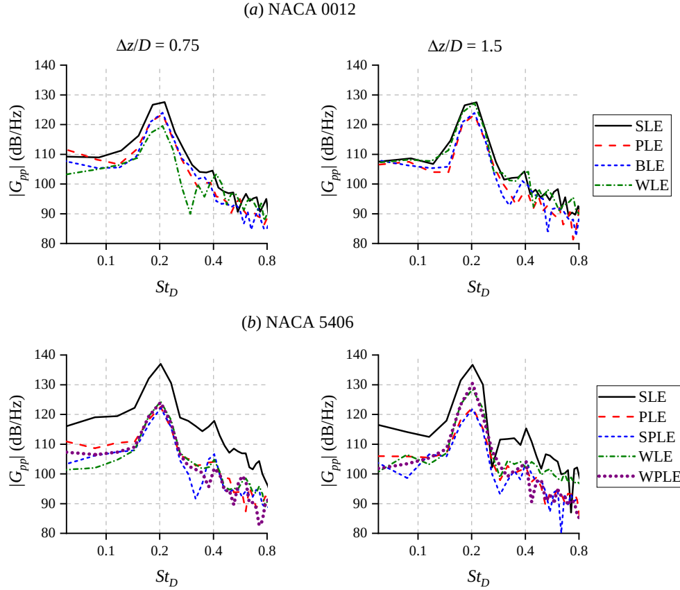
Figure 4.21: The magnitude of cross-spectral density |G_{pp}| at two locations separated by \Delta z/D = 0.75 (left column) and \Delta z/D = 1.5 (right column) from the airfoil midspan. The top row (a) corresponds to 0012 airfoils, while the 5406 ones are at the bottom (b).
