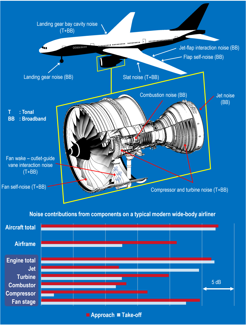
Figure 1.3: (Top) Several of the most relevant noise sources on a modern airliner, including those inside a turbofan (middle). (Bottom) A comparison between the noise contribution from engine components, airframe, and the total from the entire aircraft [18].
