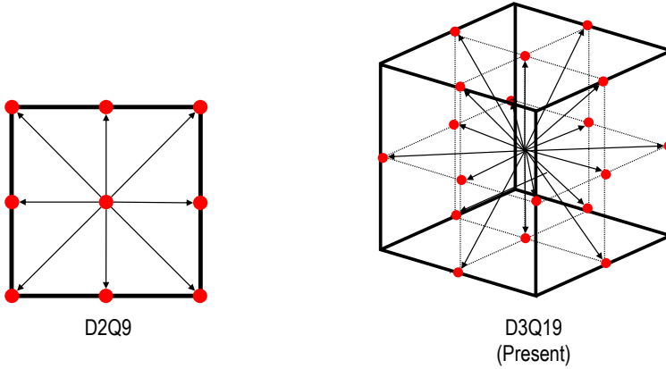
Figure 2.3: The illustration of two different LBM stencil examples: 2-dimension, 9-velocity vectors (D2Q9) and 3-dimension, 19-velocity vectors (D3Q19).
