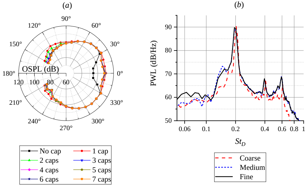
Figure 5.11: (a) Effect of the number of caps on the overall sound pressure level (OSPL) at different observation angles 1 m away from the rod center (fine grid resolution setting). (b) The convergence trend of the acoustics source power level (PWL) against various grid resolutions.
