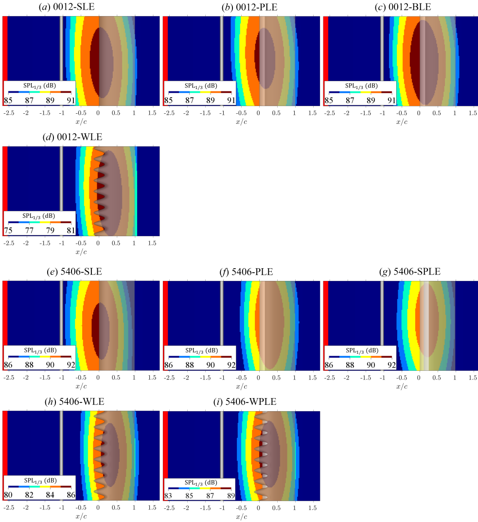
Figure 4.16: Acoustic source map of the different LE treatments for the one-third octave band at the fundamental tone ( St_D = 0.2 ). The nozzle outlet is shown as the red area at the left of each plot. Porous medium region is coloured with brighter shade.
