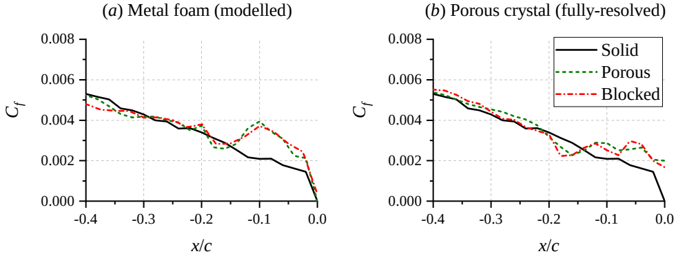
Figure 3.44: Streamwise distribution of mean wall-friction coefficient C_f for the different TE types at zero AoA and U_\infty = 20 \text{ m/s} .
