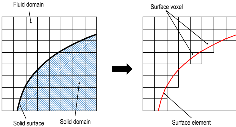
Figure 2.2: An illustration of the discretisation of the simulation domain. Note that although the surface voxels are drawn with a cubic shape, this is no longer accurate as the part of their volume inside the solid domain will be removed.
