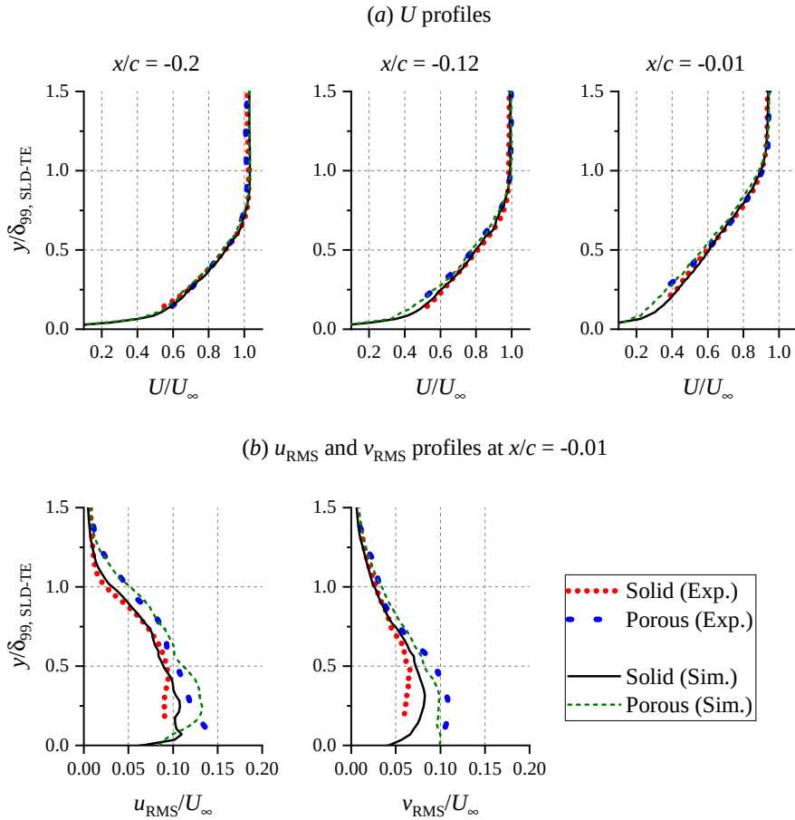
Figure 3.11: (Porous cell) Comparisons of flow statistics in the turbulent boundary layer. All data points have been extracted at the airfoil midspan. Mean wall-parallel velocity ( U ) profiles at several chordwise locations are shown in (a); profiles of root-mean-square (RMS) of velocity fluctuations in the wall-parallel ( u_{\text{RMS}} ) and wall-normal ( v_{\text{RMS}} ) directions are shown in (b). Note that "experiment" is abbreviated as (Exp.).
