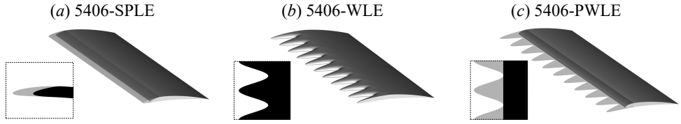
Figure 4.27: The isometric view of 5406-SPLE, 5406-WLE, and 5406-PWLE. The porous section of the airfoil is shown with lower opacity. The inset for SPLE shows a lateral view of the airfoil; for WLE/PWLE configurations, the insets show the top-down view of the planform.
