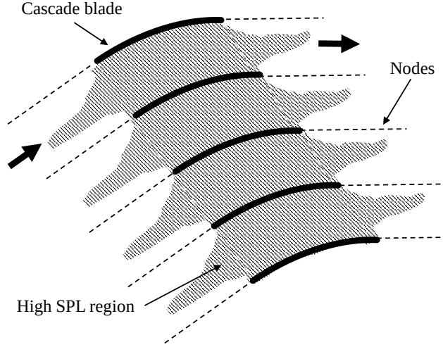
Figure 5.19: The resonant mode \beta (i.e., half-wavelength mode) in a linear cascade as reported by Parker [32].
