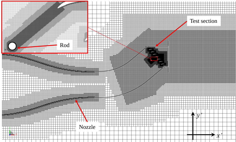
Figure 5.6: A cut plane showing the grid arrangement at the domain midspan for the finest grid resolution setting. The inset shows a close-up view on the region bounded by the red box.
