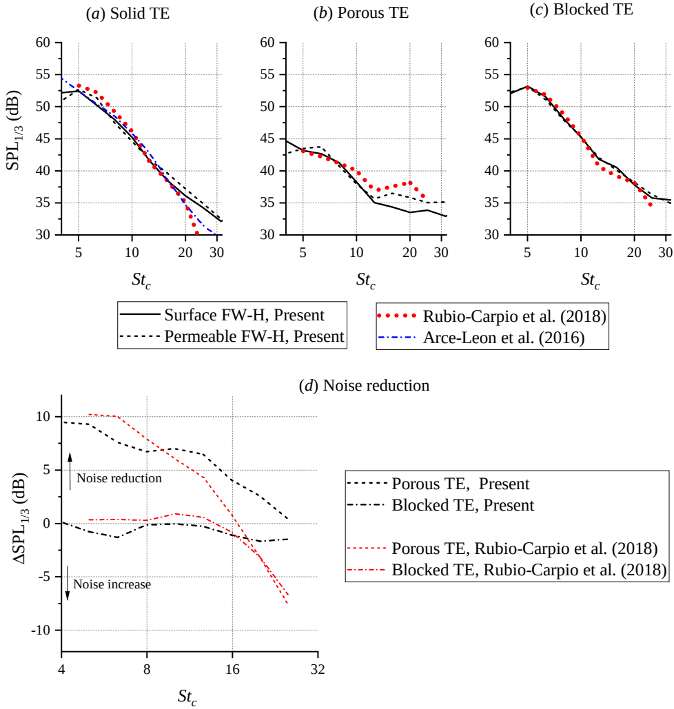
Figure 3.9: (Metal foam) Normalised one-third octave far-field sound spectra SPL_{1/3} of the (a) solid, (b) porous, and (c) blocked trailing edge. The noise reduction spectra is shown in (d). Sound pressure is calculated directly above the TE ( x/c = 0 ). Experimental data are extracted from León et al. [70] and Rubio Carpio et al. [51].
