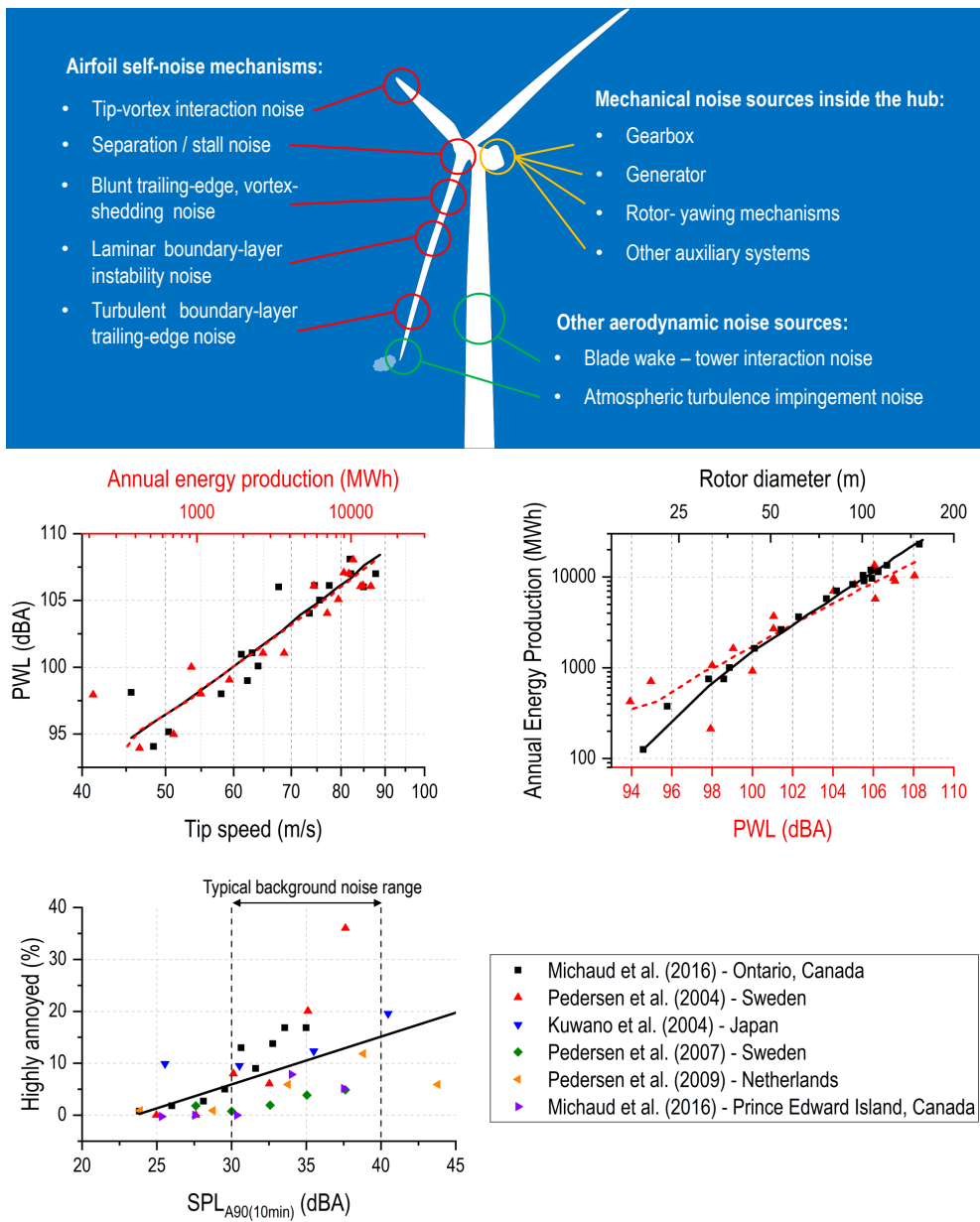
Figure 1.6: (Top) Various noise sources on a modern horizontal-axis wind turbine. (Middle) The correlation between sound power level (PWL) with rotor tip speed, rotor diameter, and the energy output of various types of Siemens wind turbines [36]. (Bottom) The correlation between the percentage of highly-annoyed people surveyed and the sound pressure level (SPL) of wind turbine noise that exceeds background noise level 90 % of the time within a 10-minute period. Data points were reproduced from Davy et al. [37].
