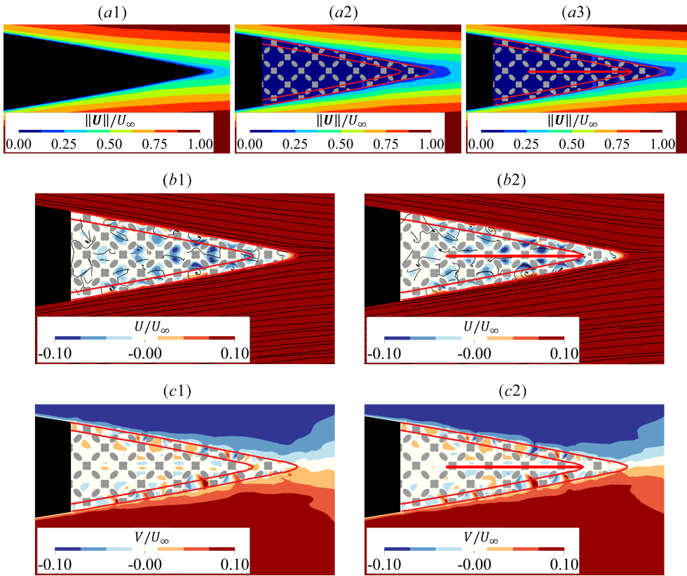
Figure 3.30: (Porous cell/fully-resolved) Comparison of contours of velocity magnitude \|\mathbf{U}\| (a), and contours of mean velocity components in the streamwise U (b) and vertical V (c) directions for the porous and blocked TE cases. The estimated entrance length is outlined with red lines. Streaklines are also provided in contours (b1) and (b2).
