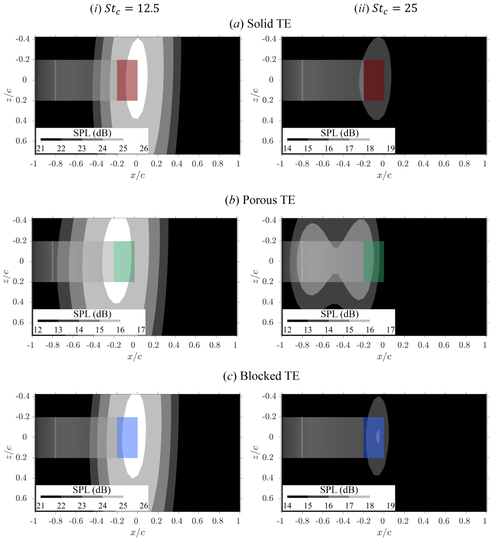
Figure 3.17: (Metal foam/modelled) Source maps for one-third octave band, centered at (i) 1250 Hz ( St_c = 12.5 ) and (ii) 2500 Hz ( St_c = 25 ) for the (a) solid, (b) porous, and (c) blocked TE cases. The trailing-edge region ( -0.2 < x/c < 0 ) for each respective case is highlighted in different colours.
