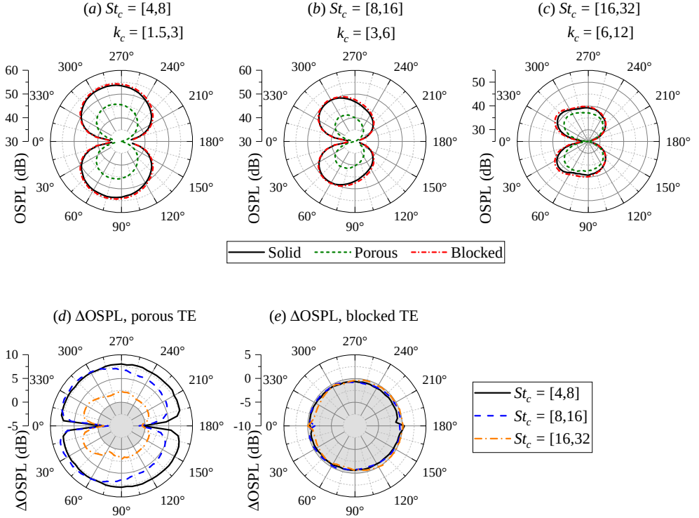
Figure 3.13: (Metal foam/modelled) Directivity of the far-field sound spectra for the different TE types, plotted in three different frequency ranges (a) 4 < St_c < 8 , (b) 8 < St_c < 16 , and (c) 16 < St_c < 32 . The airfoil leading edge is facing towards 0^\circ . The directivity of the noise reduction level is given in plots (d) and (e) with the area in grey delimiting the noise increase region. The airfoil leading edge is facing towards 0^\circ .
