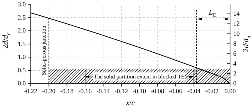
Figure 3.36: (Porous cell/fully-resolved) The chordwise distribution of TE thickness normalised by unit-cell dimension 2d/D and mean pore size 2d/d_p . The estimated two-sided extent of the entrance length is shown as the shaded region. L_E is the chordwise extent of the porous insert where the local thickness is equal to the aforementioned entrance length extent.
