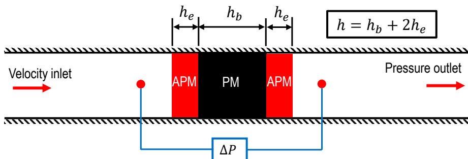
Figure 2.10: A sketch of the porous material permeability test rig in the numerical simulation.
