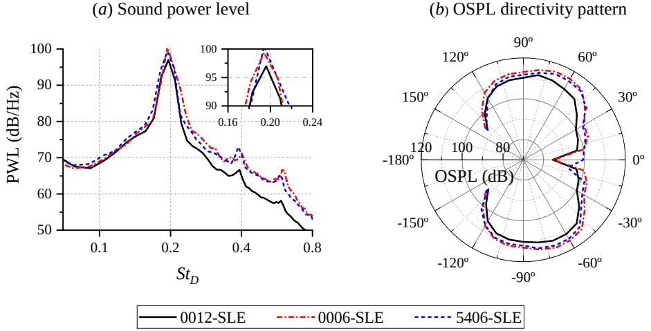
Figure 4.12: The comparison of the sound power level (PWL) (a) and the far-field directivity pattern (b) of the baseline airfoils.
