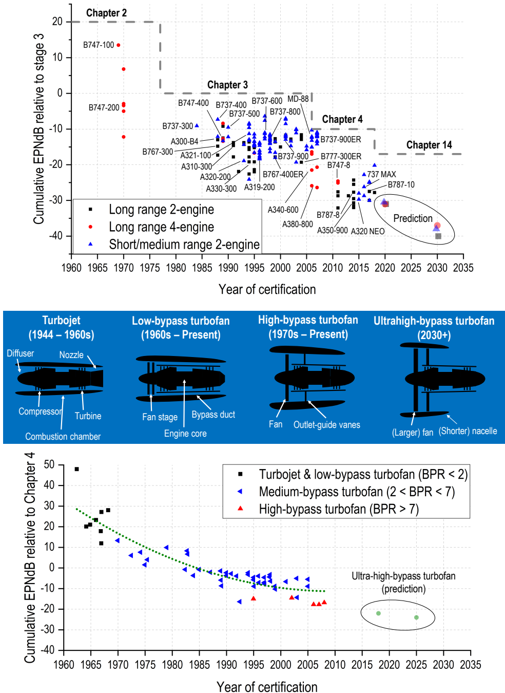
Figure 1.2: (Top) The trend of aircraft noise in term of the cumulative effective-perceived noise level in decibel (EPNdB) relative to the Stage 3 limit [13]. (Middle) Types of turbomachinery as aircraft propulsion system. (Bottom) The correlation between the aircraft noise in cumulative EPNdB relative to the Chapter 4 limit and the propulsion system [14].
