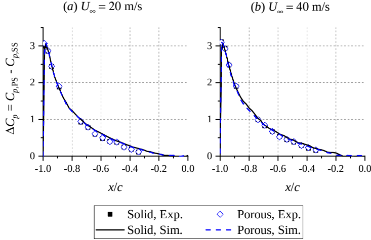
Figure 3.45: (Metal-foam/modelled) The mean surface pressure difference \Delta C_p between the pressure and suction sides of the airfoil at 7.8^\circ AoA. Plot (a) shows the distribution for U_\infty = 20 m/s, and (b) for U_\infty = 40 m/s.
