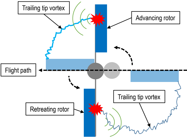
Blade-Vortex Interaction (BVI) on a two-blade rotor (top view)
