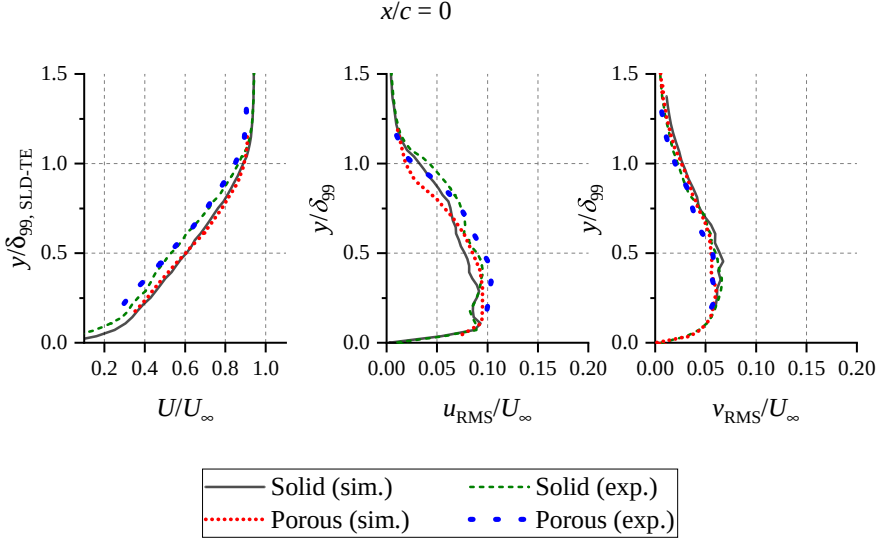
Figure 3.8: (Metal foam) Profiles of the time-averaged ( U ) and the root-mean-square of the wall-parallel ( u_{\text{RMS}} ) and of the wall-normal ( v_{\text{RMS}} ) velocity components at x/c = 0 . Experimental data are extracted from Rubio Carpio et al. [51, 60].
