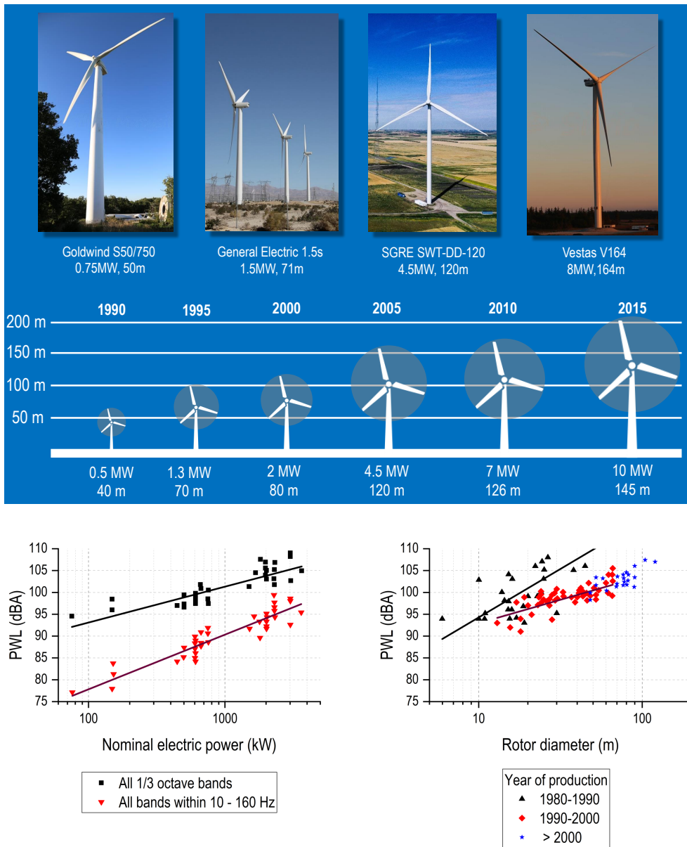
Figure 1.5: (Top) The trend of wind-turbine rotor diameter for the past 3 decades [32]; photos were taken from online databases [33], SGRE: Siemens-Gamesa Renewable Energy. (Bottom) The correlation between acoustic power level (PWL) with power output and rotor diameter [34, 35]. Logarithmic fit of the dataset is shown as solid lines.
