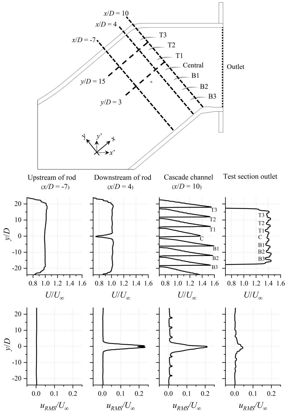
Figure 5.13: Profiles of mean velocity ( U/U_\infty ) and root-mean-square of velocity fluctuations ( u_{RMS}/U_\infty ) in the x direction, measured at different sampling lines along the test section midspan ( z/D = 0 ). These lines are indicated in the sketch at the upper half of the figure. Note that the sampling line and velocity vector at the test section outlet are based on the global coordinate system ( x' and y' ).
