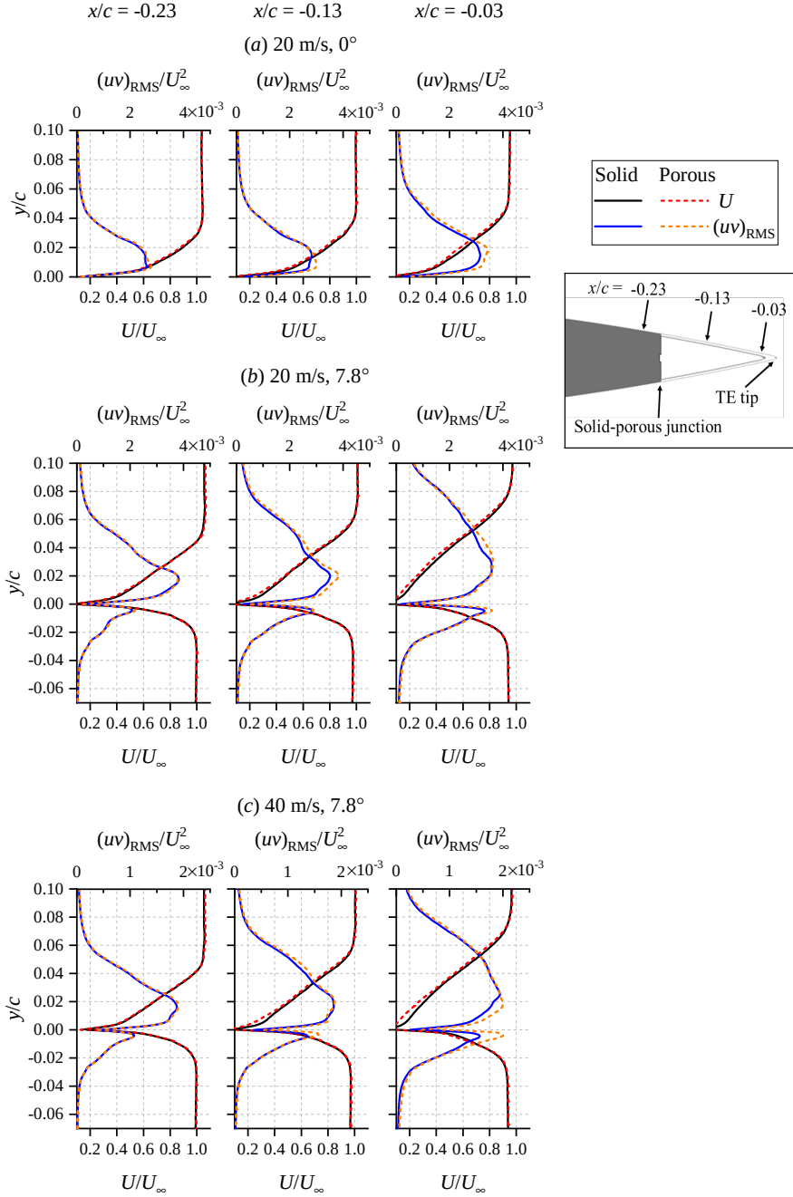
Figure 3.27: (Metal foam/modelled) Comparison of boundary layer profiles for solid and porous TE, depicting the mean wall-parallel velocity U and the root-mean-square of Reynolds stress (uv)_{\text{RMS}} . The profiles are plotted along the local wall-normal direction. The inset below the legend illustrates the locations where the profiles are sampled.
