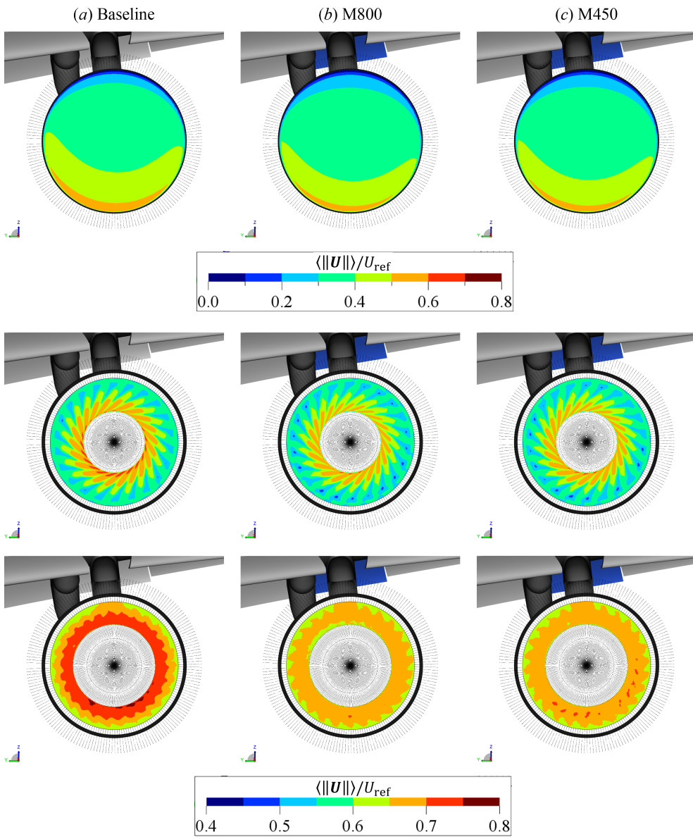
Figure 5.29: (Front view) Contours of phase-locked average of velocity magnitude \langle ||\mathbf{U}|| \rangle at the SDT inlet (top row), interstage (middle row), and outlet (bottom row).
