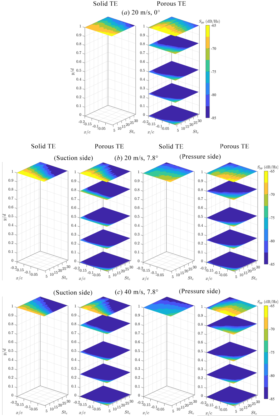
Figure 3.33: (Metal foam/modelled) Contours of spanwise-averaged pressure fluctuations spectra S_{pp} along the last 20% of the airfoil chord. For porous TE, the contours are plotted for different depth ratio y/d ; for pressure side plots, the y/d direction is reversed. S_{pp} has been normalized against freestream dynamic pressure q_\infty^2 .
