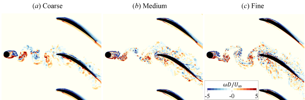
Figure 5.10: Comparison of spanwise vorticity ( \omega_z ) contour between the different resolution settings. These instantaneous snapshots were taken at approximately the same shedding phase.
