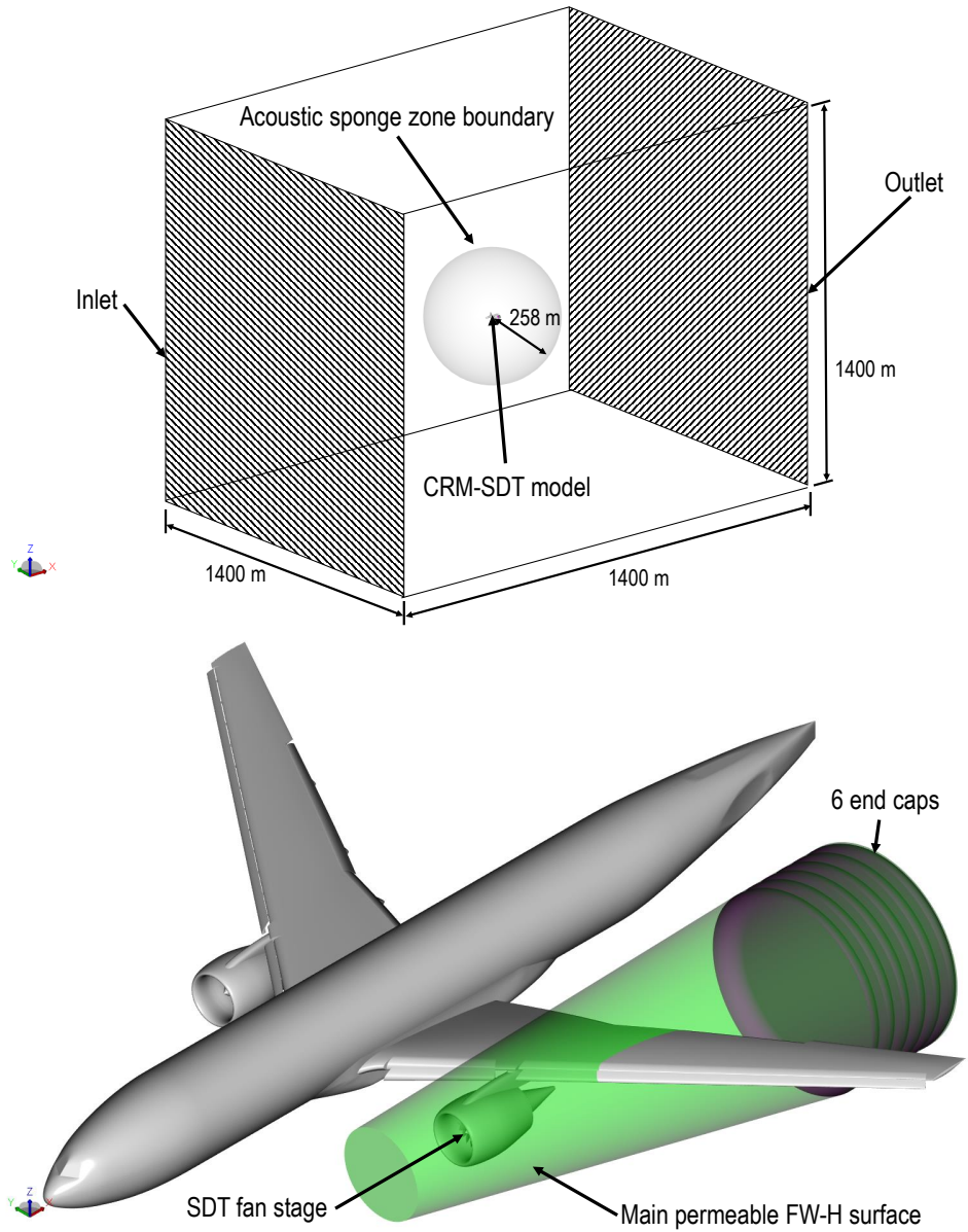
Figure 5.26: (Top) The simulation domain enclosing the CRM/SDT model. (Bottom) The configuration of permeable FW-H surface for noise analyses.
