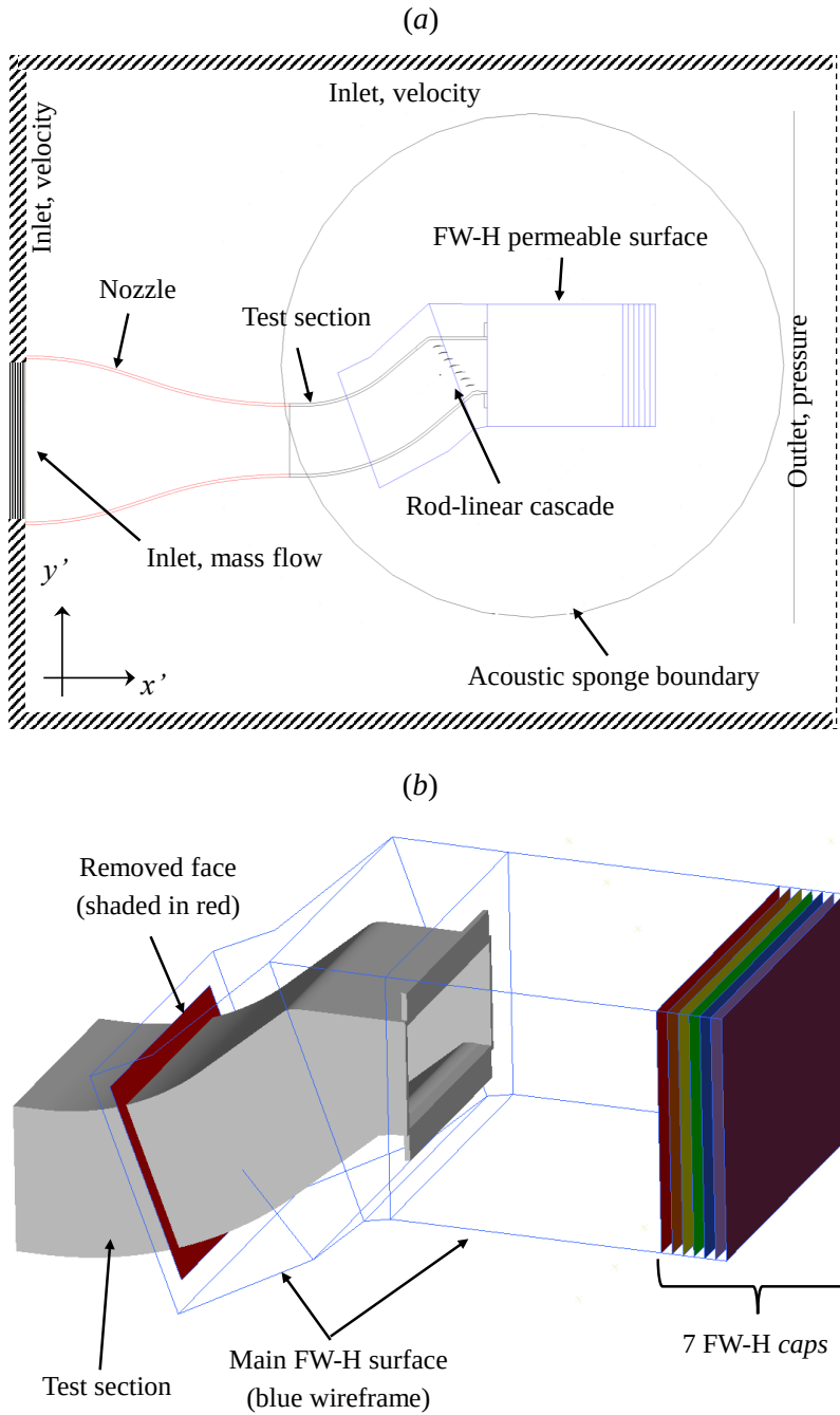
Figure 5.5: (a) A (not-to-scale) lateral view of the simulation domain. (b) A closer view the FW-H permeable surface setup, revealing the 7 caps. The nozzle is hidden in this view and the edges of the main FW-H surface are drawn as a wireframe.
