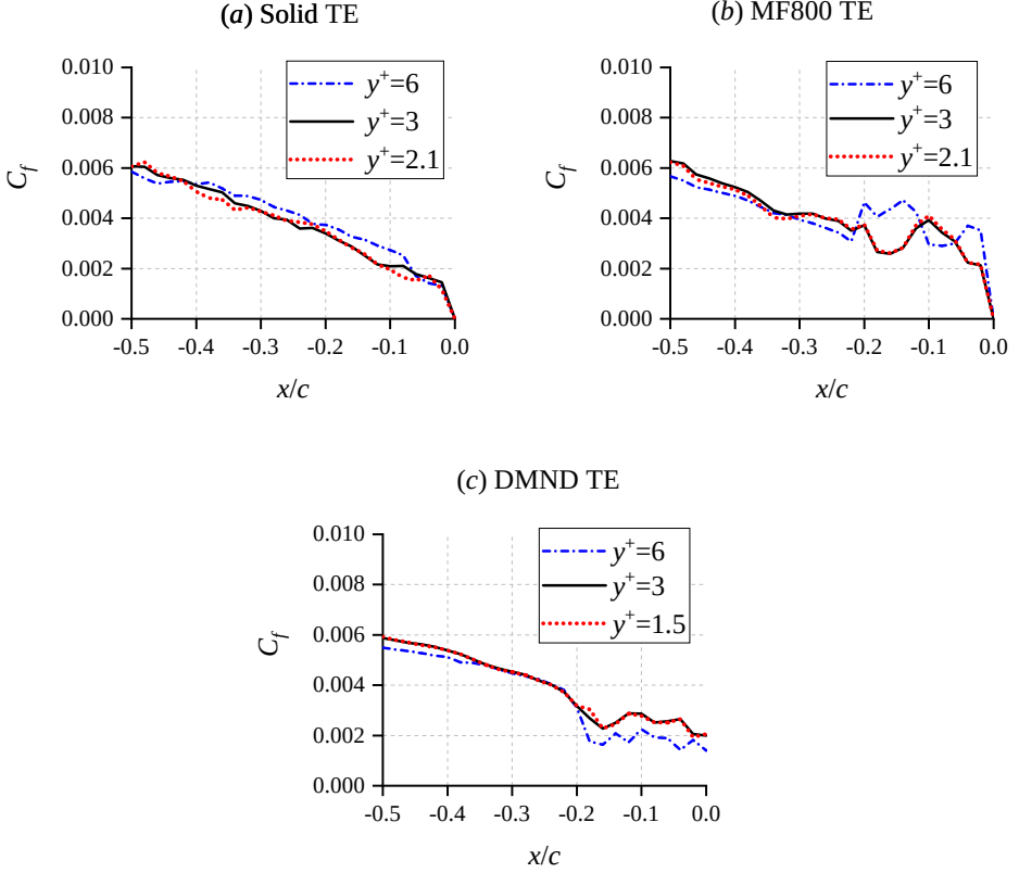
Figure 3.7: The comparison of mean wall-friction coefficient along the airfoil midspan ( -0.5 < x/c < 0 ) for the different grid resolutions.
