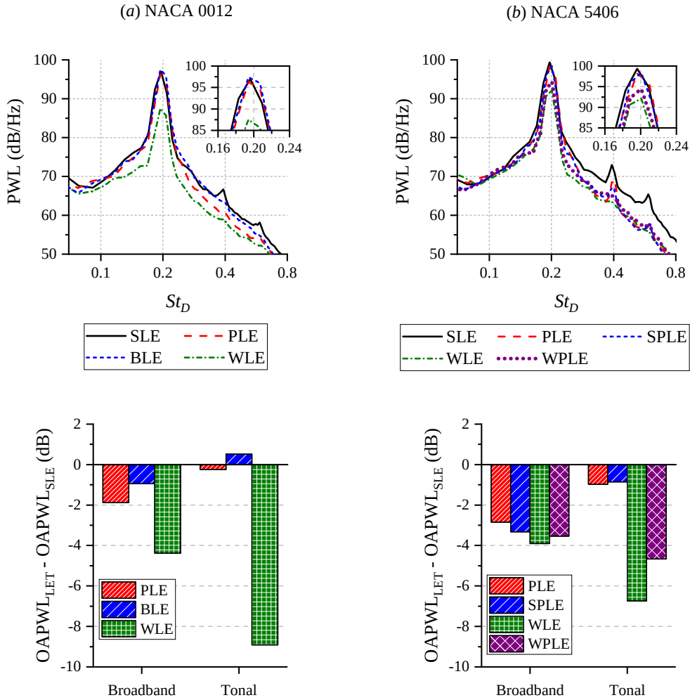
Figure 4.13: The upper row shows the comparison of the sound power level (PWL) for the different LE treatments. The lower one shows the OAPWL difference between the airfoils with LE treatments (LET) and the baseline (SLE) in tonal ( 0.15 < St_D < 0.25 ) and broadband noise components ( St_D > 0.25 ).
