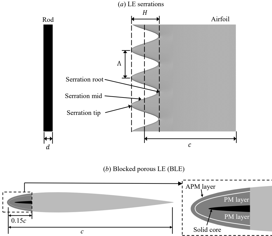
Figure 4.5: The nomenclature for the rod-serrated airfoil (WLE) configuration (a), and for the porous LE arrangement of the 0012-BLE configuration (b).
