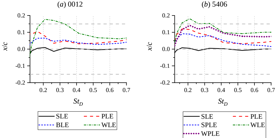
Figure 4.17: The x/c position of maximum SPL in the acoustic source map at different frequencies.
