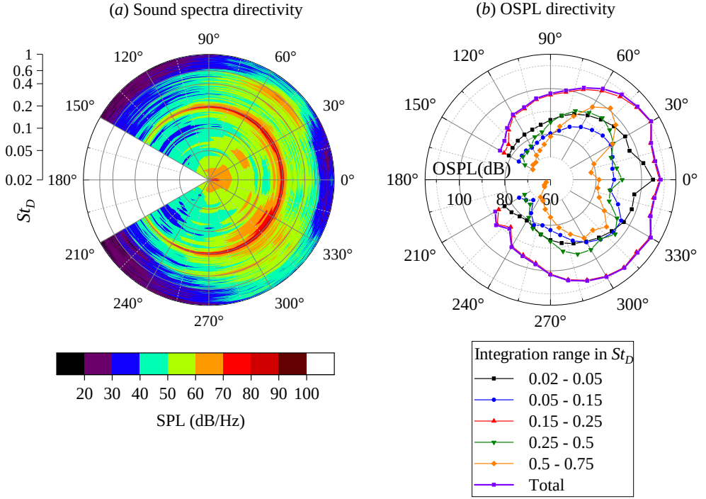
Figure 5.17: Far-field sound spectra and OSPL directivity pattern along an arc in the x' - y' plane. The arc has a radius of 1 m centered at the rod midspan.
