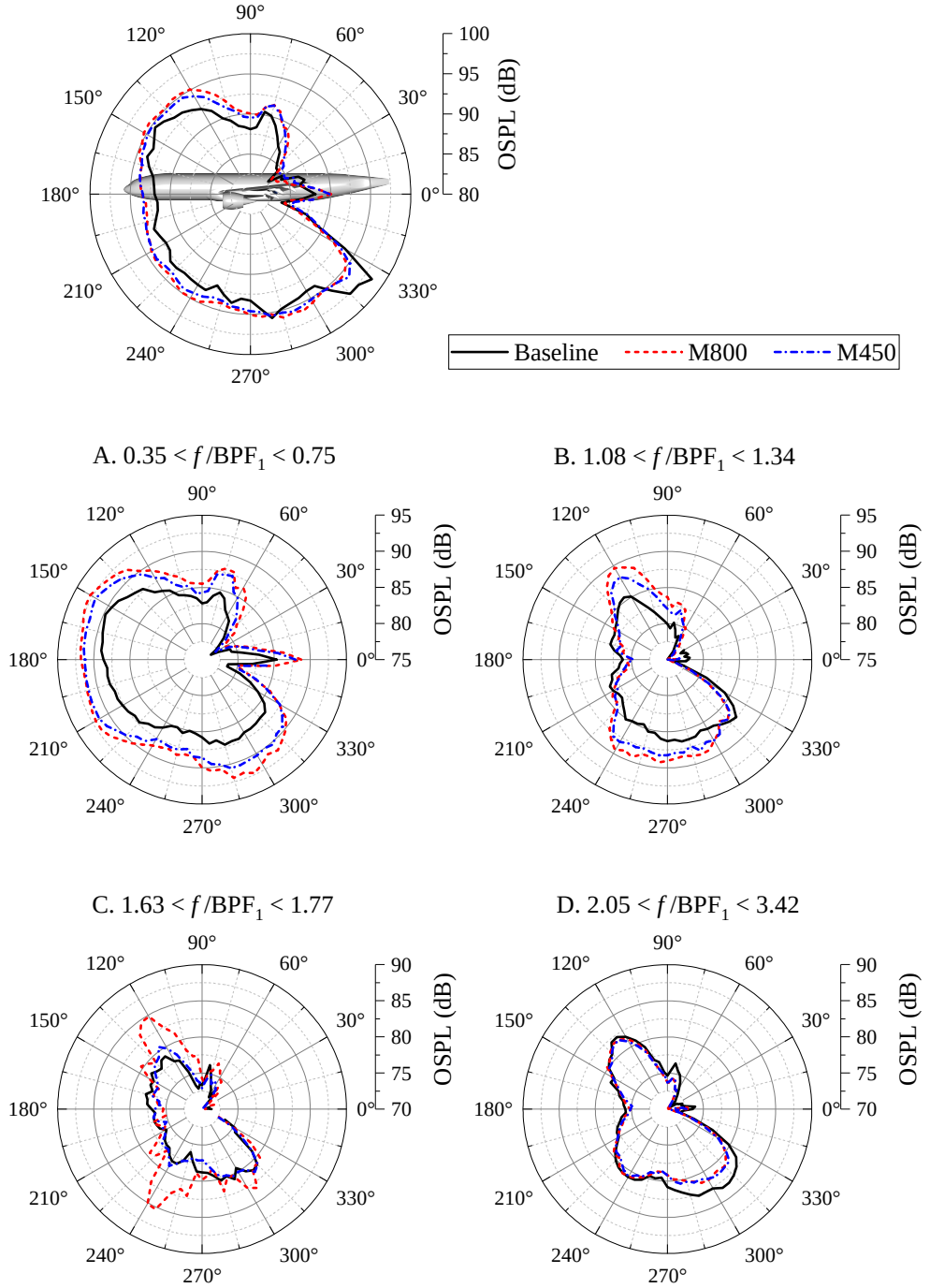
Figure 5.37: The noise directivity pattern along the lateral axis. Directivity plots are also provided at frequency bands where notable discrepancies between the modified and baseline configurations are present in figure 5.36.
