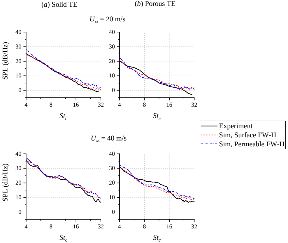
Figure 3.10: (Metal foam) Validation of far-field noise spectra from the simulation for a higher AoA ( 7.8^\circ ) and Reynolds number cases. Observer location is x/c = -0.68 , y/c = 4.95 .
