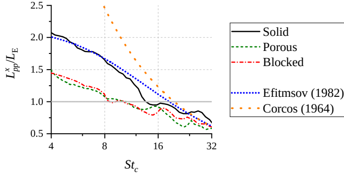
Figure 3.39: (Porous cell/fully-resolved) Streamwise correlation length of surface pressure fluctuations L_{pp}^x at x/c = -0.05 . A comparison with Corcos [19] and Efimtsov [90] models are also provided.
