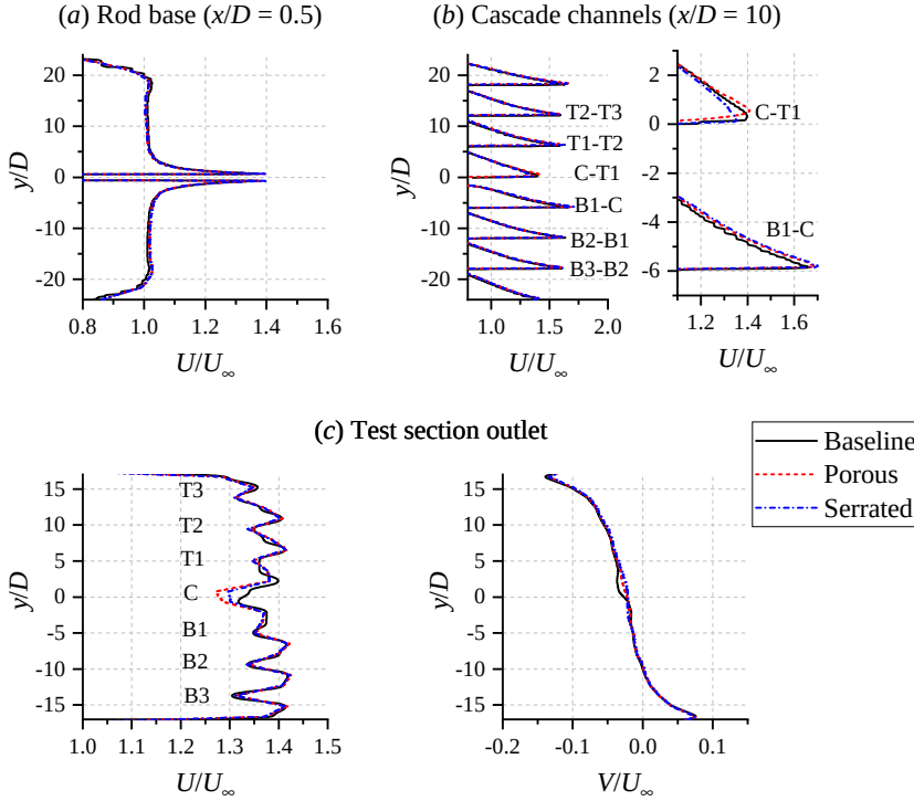
Figure 5.21: Velocity profiles sampled at various segments in the test section for the RLC with different central blade configurations.
