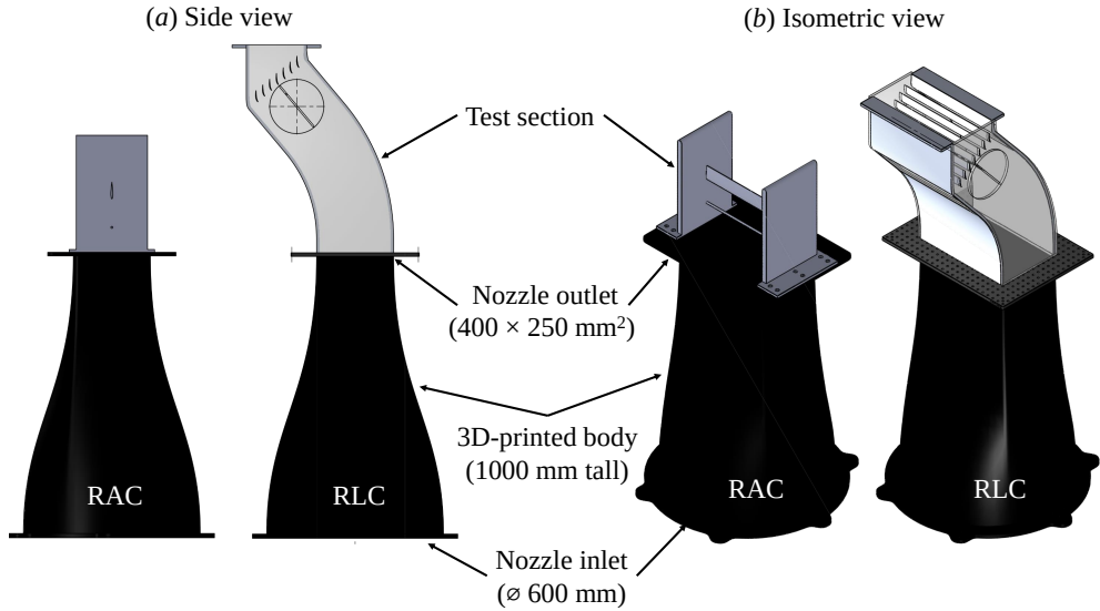
Figure 5.2: A comparison between a rod-airfoil configuration (RAC) setup and the rod-linear cascade (RLC) one when mounted in the vertical wind tunnel of TU Delft.
