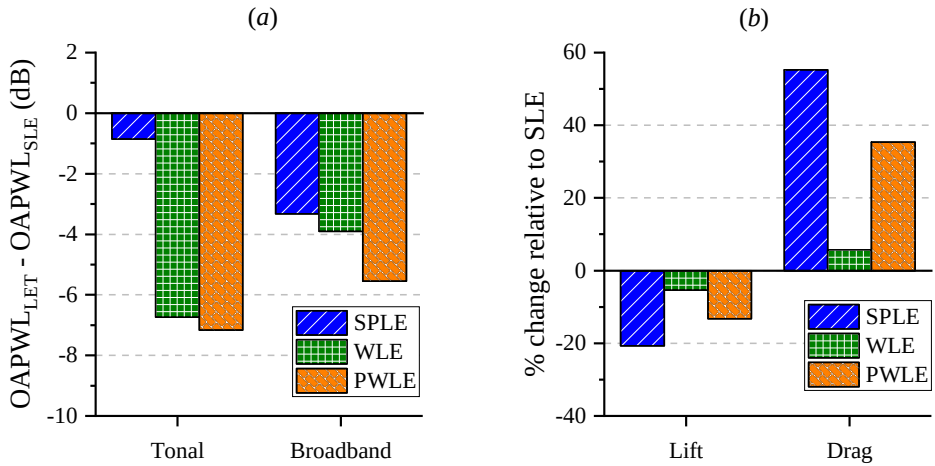
Figure 4.28: Comparisons of (a) source power level and (b) time-averaged lift and drag coefficients between the 5406-PWLE and those with different LE treatments. The values are relative to the 5406-SLE.
