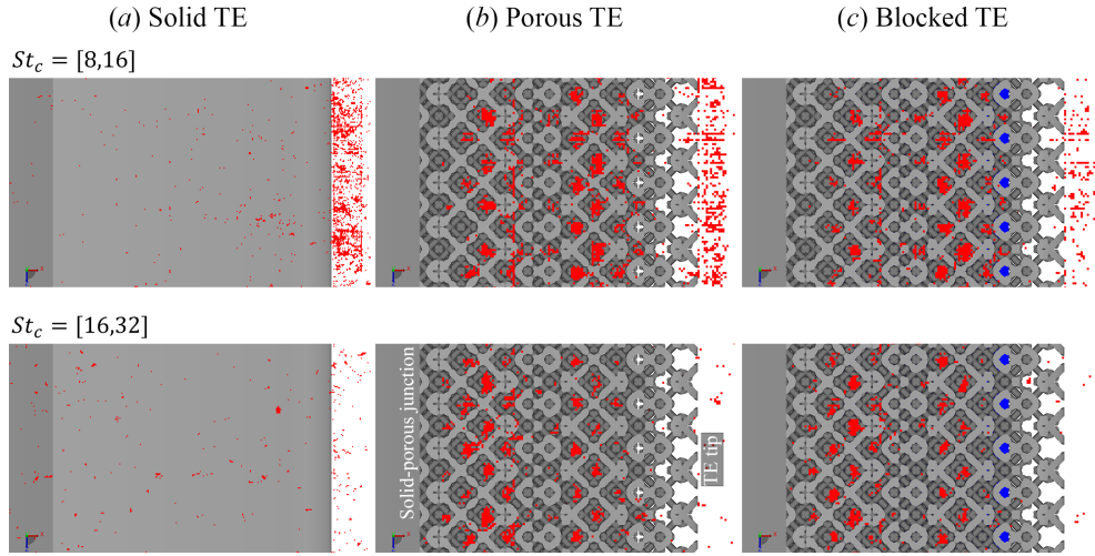
Figure 3.18: (Porous cell/full-resolved) Noise source localisation based on the vortex sound theory algorithm [77], FIND. The figure illustrates a top view of the airfoil. Clusters of noise sources are coloured in red, while the solid partition in the blocked TE is shown in blue. The last 20 % of the airfoil chord is coloured in light grey.
