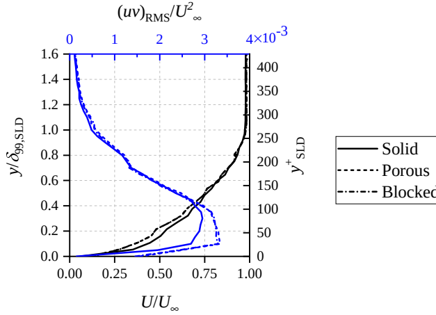
Figure 3.43: (Porous cell/fully-resolved) Boundary-layer profiles at x/c = -0.1 . The plots show mean wall-parallel velocity component U (black lines) and the root-mean-square of Reynolds stress component in the wall-parallel and wall-normal directions (uv)_{RMS} (blue lines). The wall-normal coordinates are also provided in term of y^+ based on the solid TE case.
