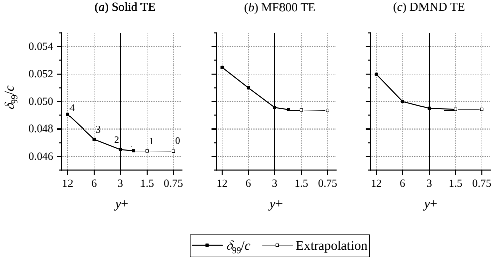
Figure 3.6: The comparison of boundary layer thickness at x/c = -0.002 for different grid resolutions. The Richardson extrapolation of the boundary layer thickness is plotted as empty square. The thick line at y^+ = 3 denotes the adopted grid resolution for the rest of the chapter. The corresponding resolution levels that are considered for the grid convergence index (GCI) studies are numbered next to the data point. MF800 - metal foam; DMND - porous cell.
