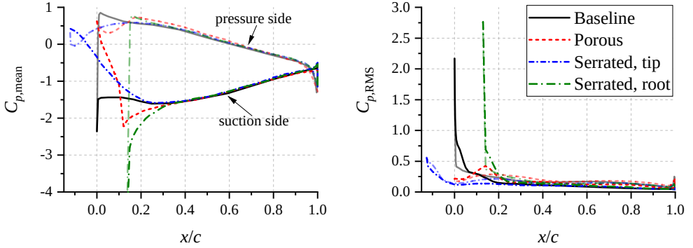
Figure 5.22: The comparisons of surface pressure statistics for the RLC with different central blade configurations. The pressure side distributions are plotted with lower opacity.
