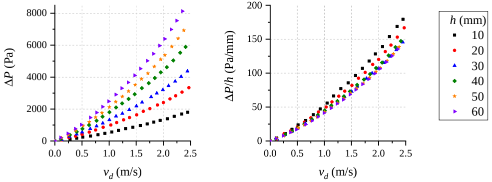
Figure 2.8: Pressure drop test result for a Ni-Cr-Al metal foam with the mean pore diameter of 0.45 mm. Data has been extracted from reference [61].
