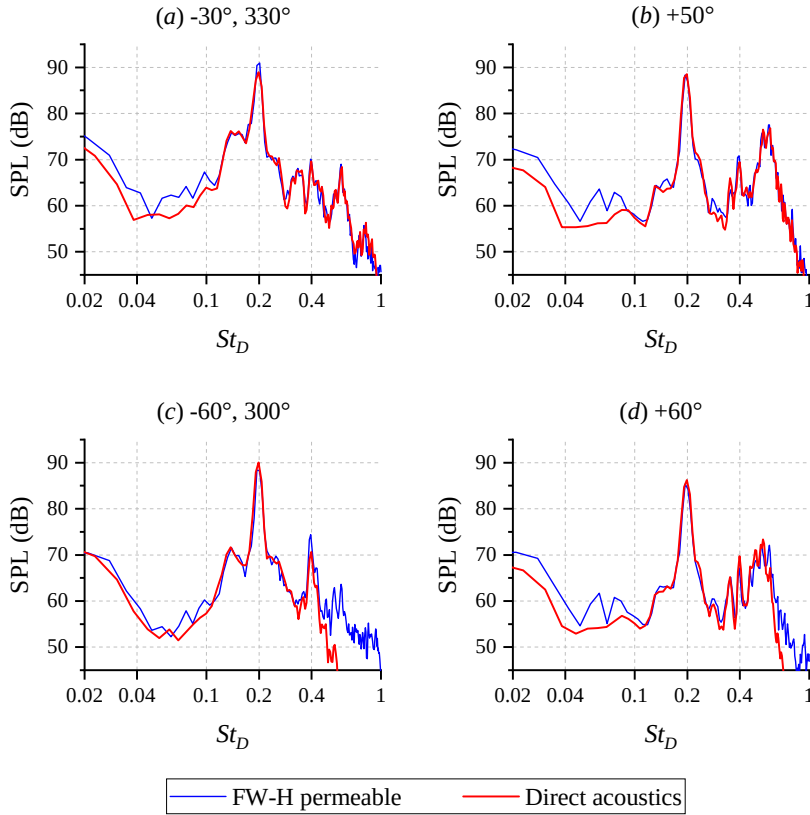
Figure 5.12: Comparison between results from FW-H analogy and direct acoustics computation for the fine grid resolution level at several observer angles and a radial distance of 0.6 m.
