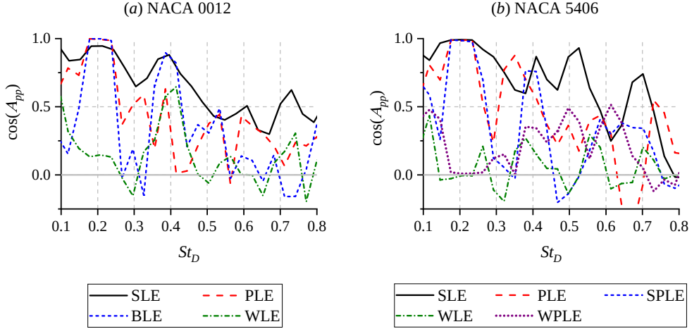
Figure 4.22: The spanwise-averaged ( 0 < z/D < 3 ) phase angle of the cross-power-spectra of surface pressure fluctuations A_{pp} for the different LE treatments.
