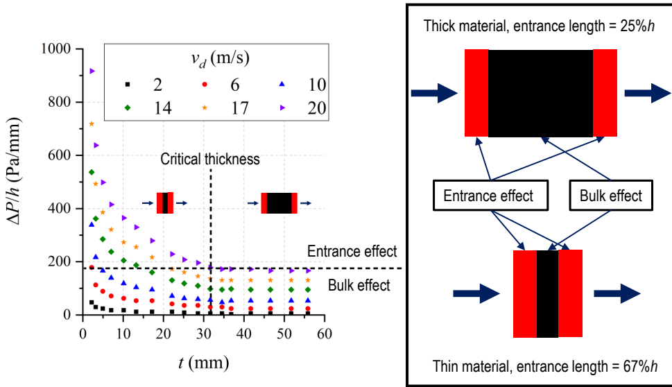
Figure 2.9: The entrance and bulk effects on the pressure drop data of a metal foam with the mean pore diameter of 0.6 mm. Data has been extracted from reference [65].
