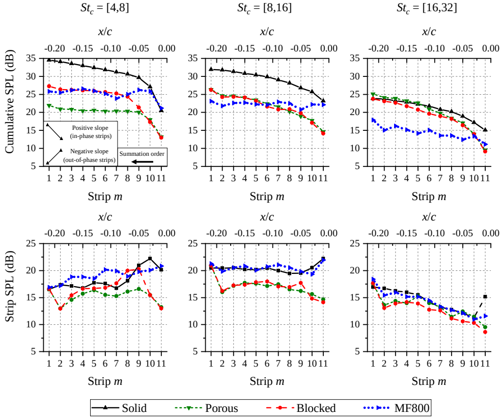
Figure 3.23: (Porous cell/fully-resolved) The sound pressure level (SPL) produced by each strip and its cumulative, integrated over 3 different frequency bands. The trends for the metal-foam TE are indicated as MF800.
