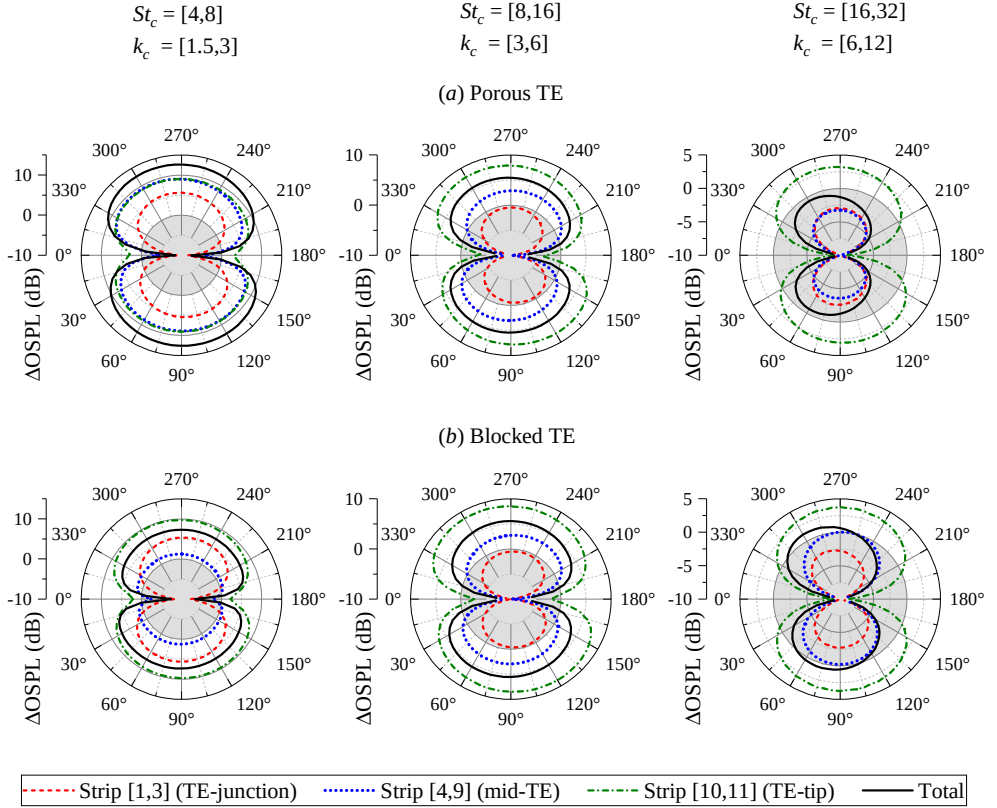
Figure 3.24: (Porous cell/fully-resolved) Noise directivity pattern, plotted as the difference between the SPL of permeable (porous and blocked TE) and solid TE cases, i.e., \Delta OSPL = OSPL_{solid} - OSPL_{permeable} , for groups of strips at different frequency bands. The grey circle at the center of the polar plot indicates regions of noise increase.
