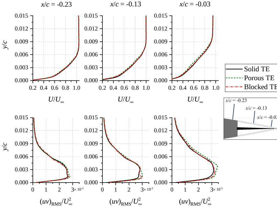
Figure 3.26: (Metal foam/modelled) Boundary layer profiles for the time-averaged streamwise velocity ( U ) and the root-mean-square of the Reynolds stress (uv)_{\text{RMS}} at different locations along the TE region. The sampling lines for the boundary layer profiles are shown in the inset depicting a segment of the blocked TE.
