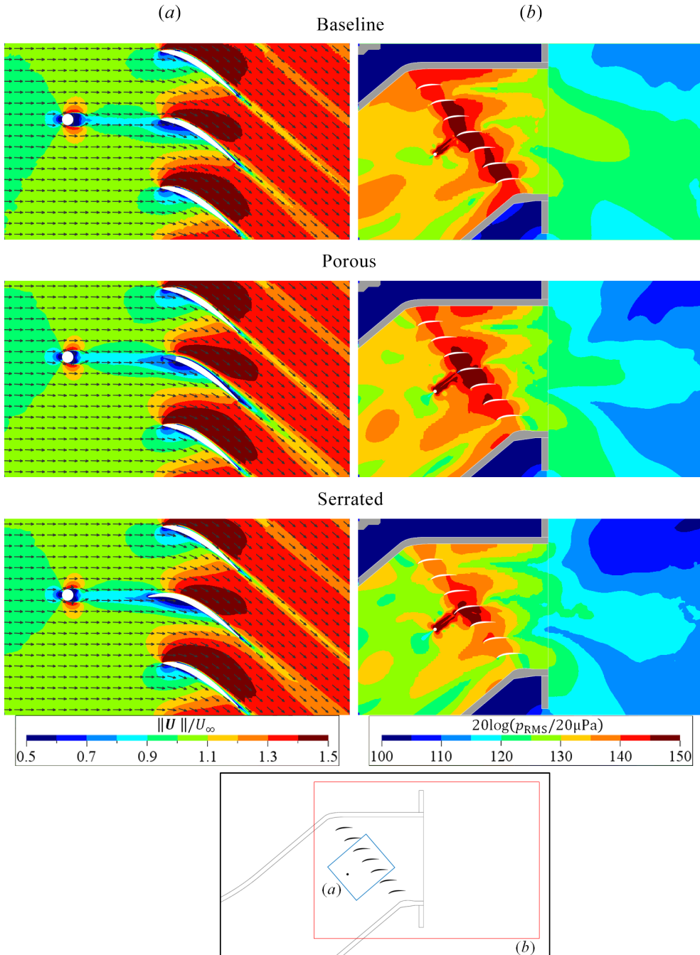
Figure 5.23: (a) Contours of time-averaged and normalised velocity magnitude, with the velocity contours plotted on top. (b) The contours of near-field pressure fluctuations, bandpassed between 0.15 < St_c < 0.25 , presented in decibel. The field of view of each contour is indicated in the inset at the lower part of the figure.
