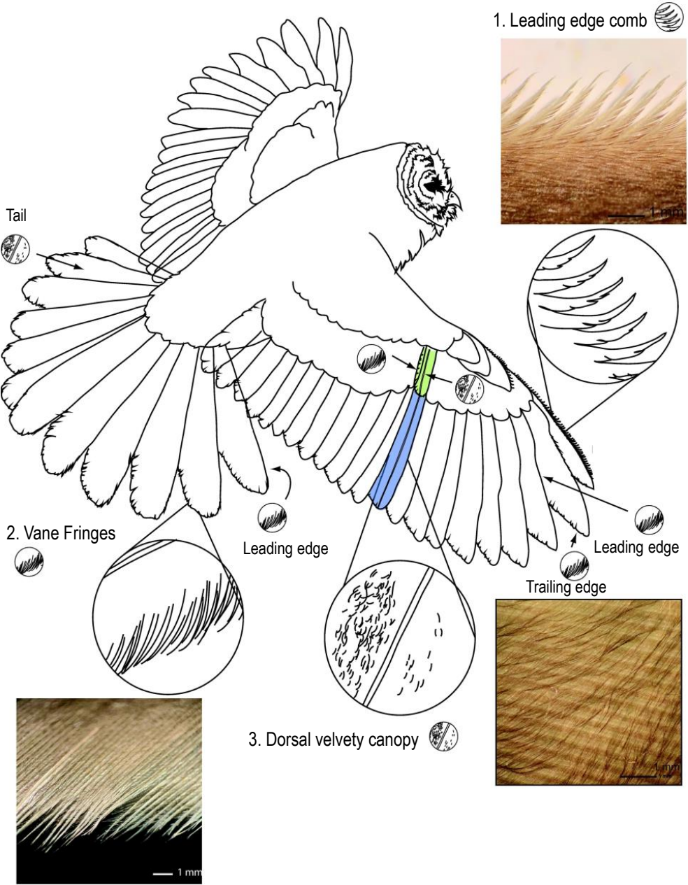
Figure 3.3: Typical features of owls' wings that are associated with the silent flight capability [24, 25]. This figure has been reproduced from Clark et al. [27].
