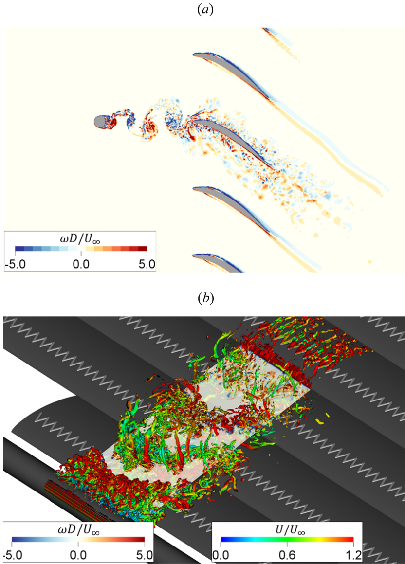
Figure 5.15: (a) Instantaneous contour of spanwise vorticity ( \omega_z ) at the midspan and (b) lambda-2 iso-surface ( \lambda_2 = -3 \times 10^9 \text{ s}^{-2} ) with y = 0 plane included for highlighting the wake pattern. The iso-surface is shown up to z = \pm 5D in the spanwise direction. Both contours have been extracted at the same time instance.
