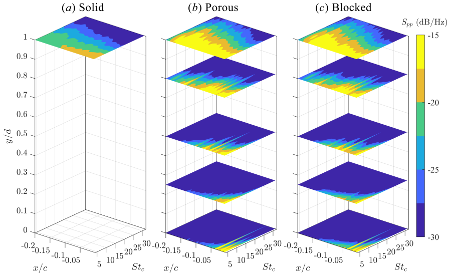
Figure 3.35: (Porous cell/fully-resolved) Contours of spanwise-averaged pressure fluctuations spectra S_{pp} along the last 20% of the airfoil chord. For porous TE, the contours are drawn at different depth ratio y/d . S_{pp} is normalised with the reference pressure of 1 Pa.
