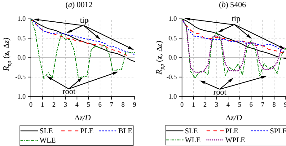
Figure 4.20: The spanwise correlation R_{pp} of the surface pressure fluctuations for the different LE treatments. The locations of serration tips and roots for the WLE are indicated in the plots.
