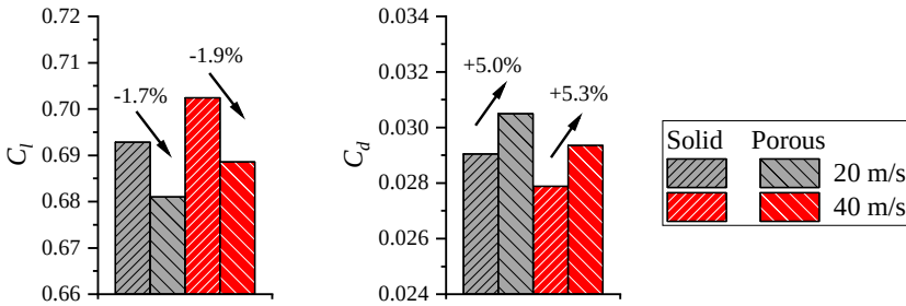
Figure 3.46: (Metal-foam/modelled) The comparison of lift and drag coefficients between the airfoils with solid and porous TE at 7.8^\circ AoA. The percentage and the arrow above the bars indicate the difference between the coefficients for the porous TE relative to the solid TE.
