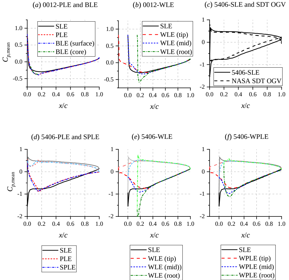
Figure 4.23: Time-averaged surface pressure distribution C_{p,mean} for the different LE treatments. For the 5406 airfoils, the pressure distribution at the pressure side is plotted in lighter shade.
