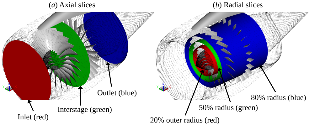
Figure 5.28: A sketch of the slice planes that will be used for plotting contours in the subsequent figures.
