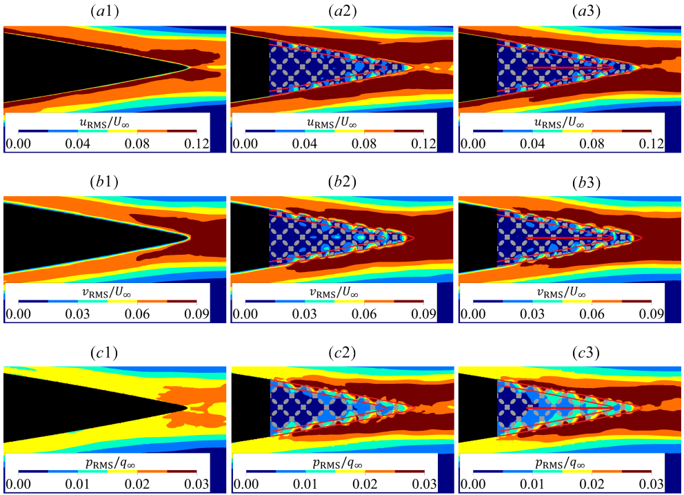
Figure 3.31: (Porous cell/fully-resolved) Contours of root-mean-square of velocity fluctuations in the streamwise u_{RMS} (a) and vertical directions v_{RMS} (b), and the contours of root-mean-square of pressure fluctuations p_{RMS} (c). The estimated entrance length is outlined with red lines. Solid TE is shown at the left column, porous TE at the middle, and blocked TE at the right one.
