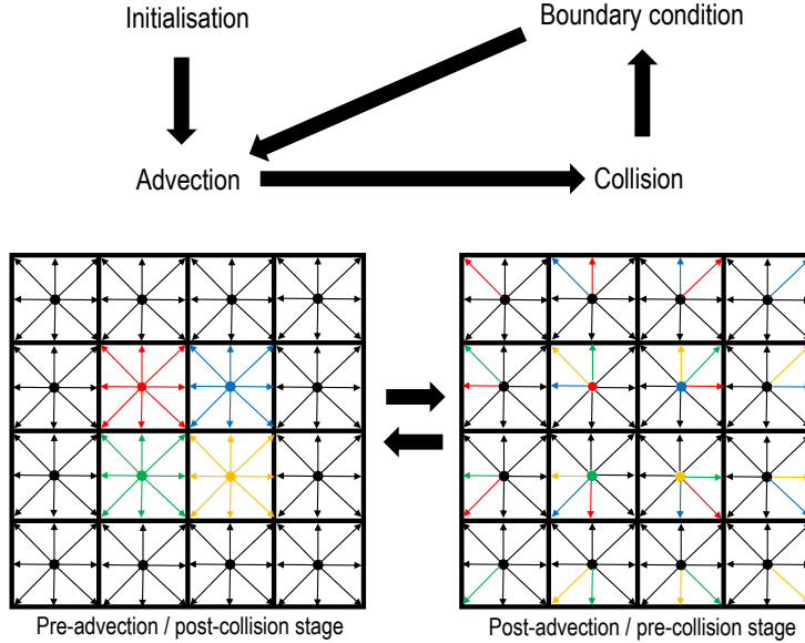
Figure 2.1: A schematic of LBM algorithm. Fluid particles in the lattice are represented as dots and the discrete particle velocity vectors as arrows. Coloured arrows have been used to indicate the advection of the velocity vectors from the 4 voxels at the center of the lattice.
