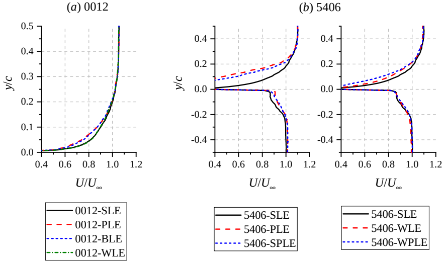
Figure 4.25: The time-averaged streamwise velocity profile at x/c = 1 for each LE treatment. The plots are sampled at the midspan ( z/c = 0 ), except for WLE and WPLE configurations, where the values are averaged over a serration wavelength.
