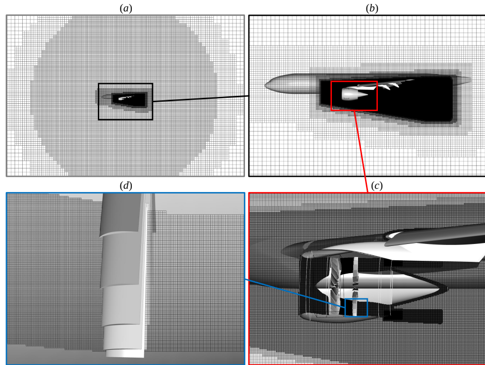
Figure 5.27: The voxel distribution in the simulation domain: (a) near the borders of the acoustic sponge boundary; (b) surrounding the airframe; (c) surrounding the SDT fan stage; (d) near the OGVs.
