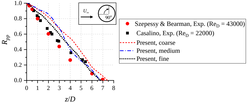
Figure 5.8: Spanwise correlation of surface pressure fluctuations on the rod surface. The rod Re_D is 26,600 in the present simulation. Reference results were obtained from Szepessy [21] and Casalino et al. [22].
