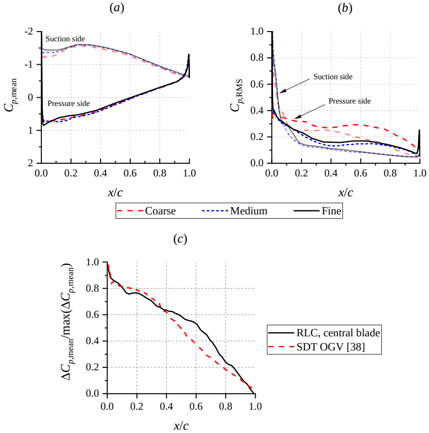
Figure 5.9: The mean surface pressure and the root-mean-square (RMS) of surface pressure fluctuations are plotted in (a) and (b) respectively. The distributions along the suction side are shown with lower opacity. Plot (c) compares the distribution of pressure difference between the suction and pressure sides of the RLC central blade and the SDT OGV; this plot is based on the fine grid resolution level.
