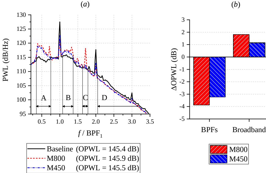
Figure 5.36: (a) Source power level (PWL) of the CRM/SDT configuration. The capital letters denote the frequency ranges where the directivity patterns are plotted in figure 5.37. Plot (b) shows the OPWL difference between the modified configurations and the baseline, divided into two categories: BPFs (the tonal peaks \text{BPF}_1 to \text{BPF}_3 ) and broadband (the broadband noise component and other tones up to f / \text{BPF}_1 = 3.5 ).
