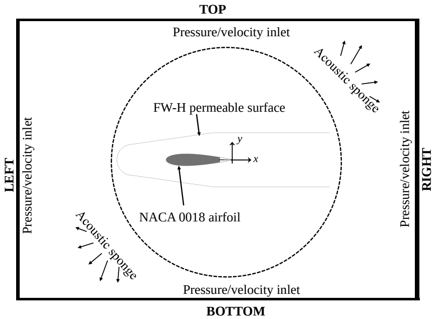
Figure 3.5: A sketch of the computational domain. Note that domain boundaries are not drawn to scale.
