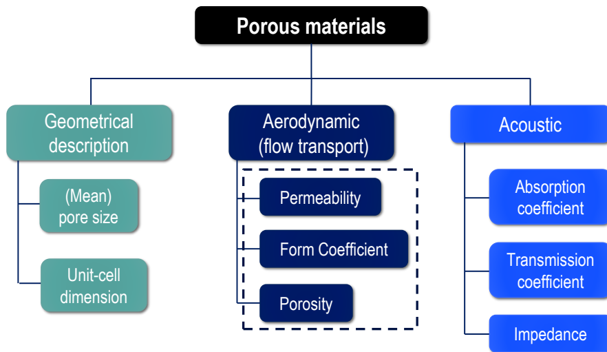
Figure 1.10: Porous material characteristics based on various aspects. The segment in dashed box contains the parameters that are commonly considered in aeroacoustics investigations.
