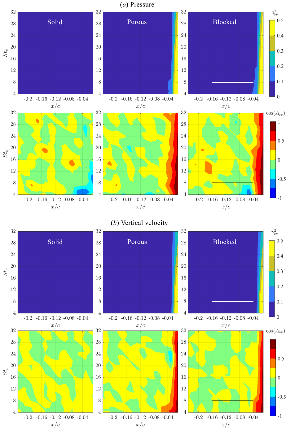
Figure 3.38: (Porous cell/fully-resolved) Contours of magnitude-squared-coherence of surface pressure fluctuations ( \gamma_{pp}^2 ) and vertical velocity fluctuations ( \gamma_{vv}^2 ), with the corresponding phase angle ( A_{pp} and A_{vv} ) between the suction and pressure sides of the airfoil.
