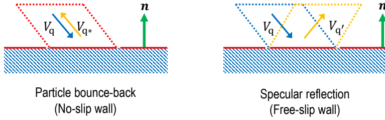
Figure 2.4: An illustration of the wall boundary conditions in LBM: the bounce-back process for no-slip wall, and specular-reflection for slip wall.
