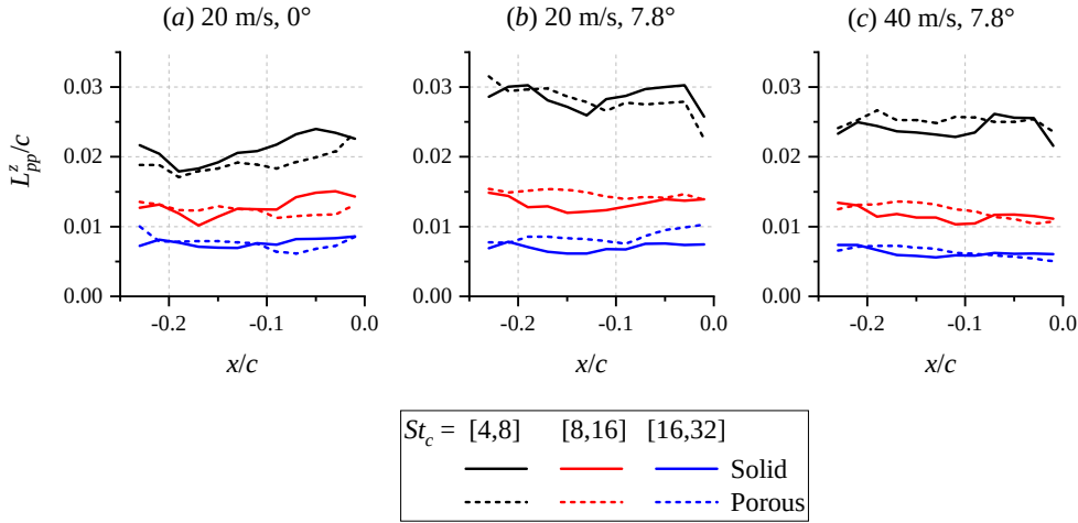
Figure 3.34: (Metal foam/modelled) Comparison of streamwise distribution of spanwise correlation length of surface pressure fluctuations L_{pp}^z between the solid and porous TE at different inflow conditions. For plots (b) and (c), the values at the suction side are presented.
