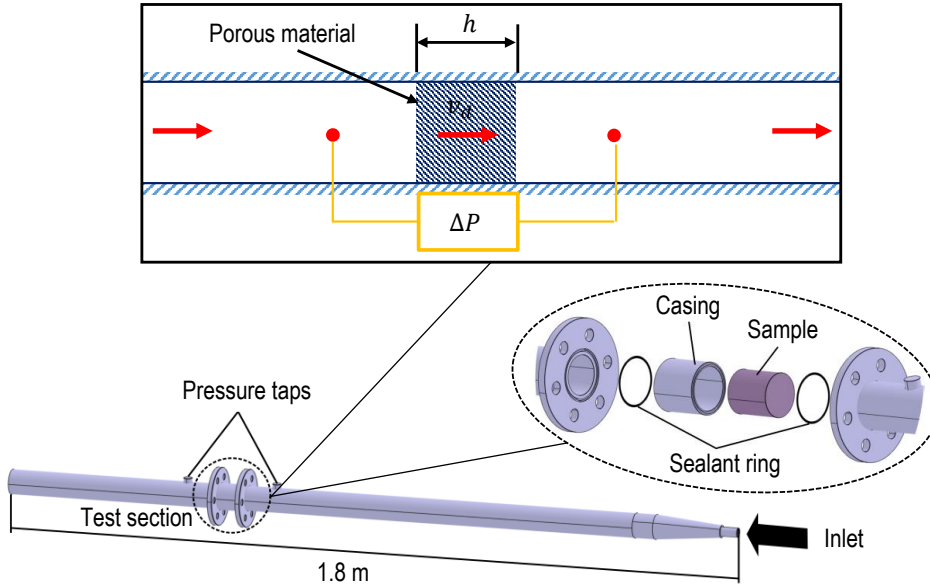
Figure 2.7: Porous material characterisation test rig at the Delft University of Technology. A simplified sketch is shown at the top.
