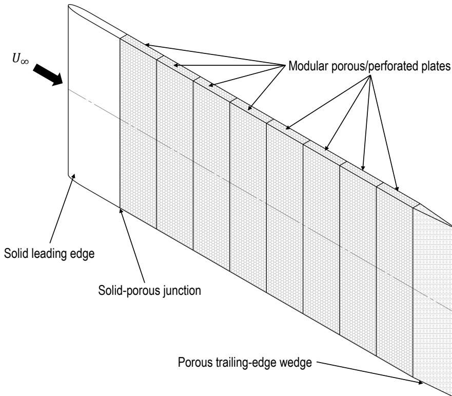
Figure 6.1: A flat-plate model consisting of a solid leading-edge and modular porous plates to investigation sound generation of a porous body.
