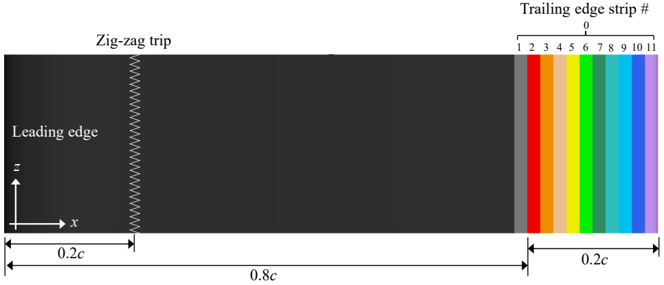
Figure 3.19: Top view of the airfoil planform, revealing the arrangement of the trailing edge strips for noise contribution analysis.
