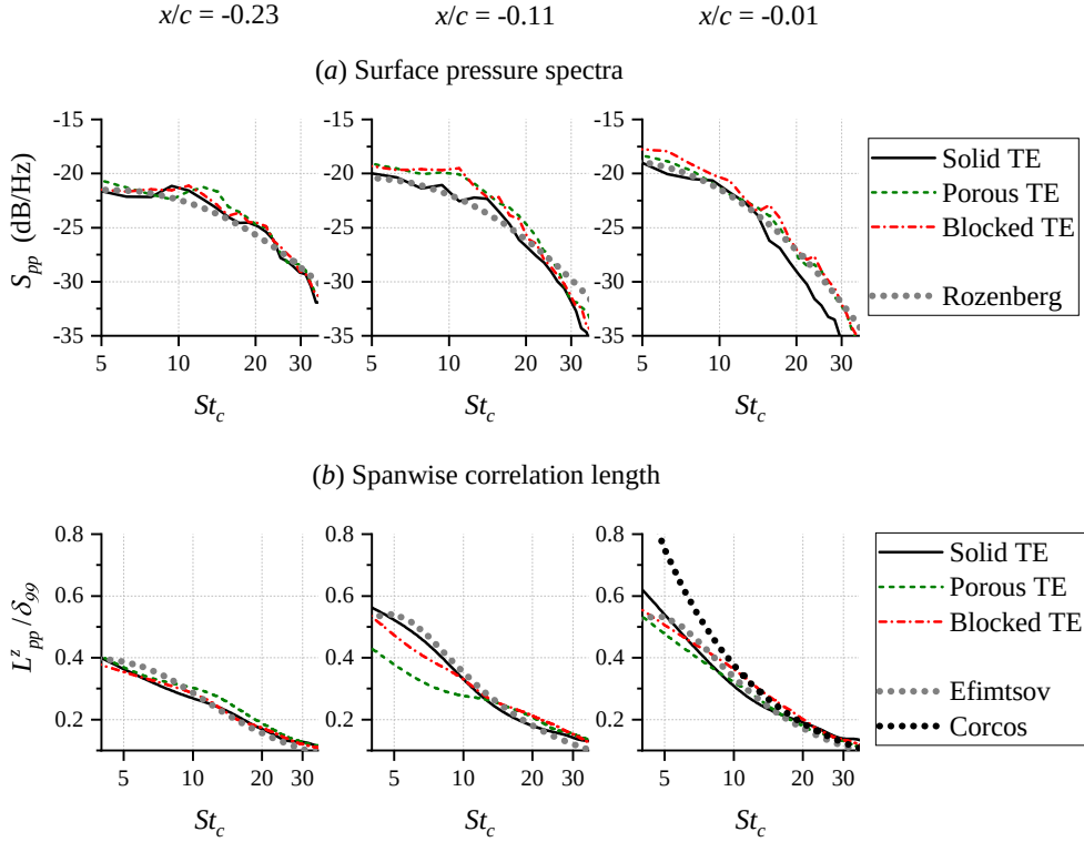
Figure 3.32: (Metal foam/modelled) The comparison of power spectral density of surface pressure fluctuations ( S_{pp} ) and spanwise coherence length ( L_{pp}^z ) between the three trailing edge treatments. The S_{pp} has been normalised with a reference pressure of 1 Pa, while L_{pp}^z with the \delta_{99} for the solid TE. For comparison, the prediction of Rozenberg's model [89] is included in plot (a), and Corcos' [19] and Efimtsov's [90, 91] in (b).
