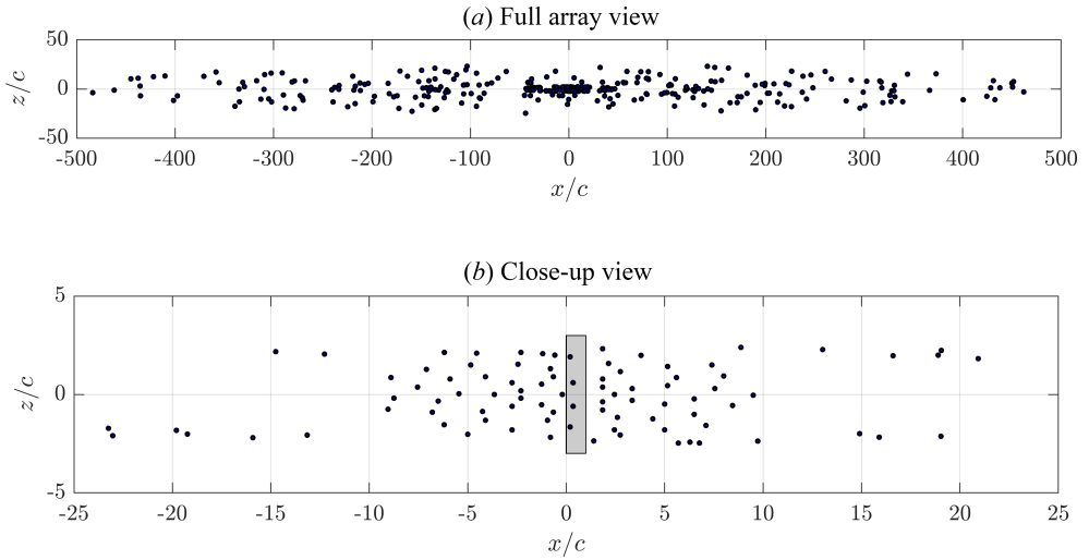
Figure 4.15: Microphone array used to obtain the acoustic source map. Overall dimension is 98\text{ m} \times 24\text{ m} with the Rayleigh limit of 0.008\text{ m} ( 0.08c ) at St_D = 0.2 . The airfoil planform is shown as grey rectangle in (b).
