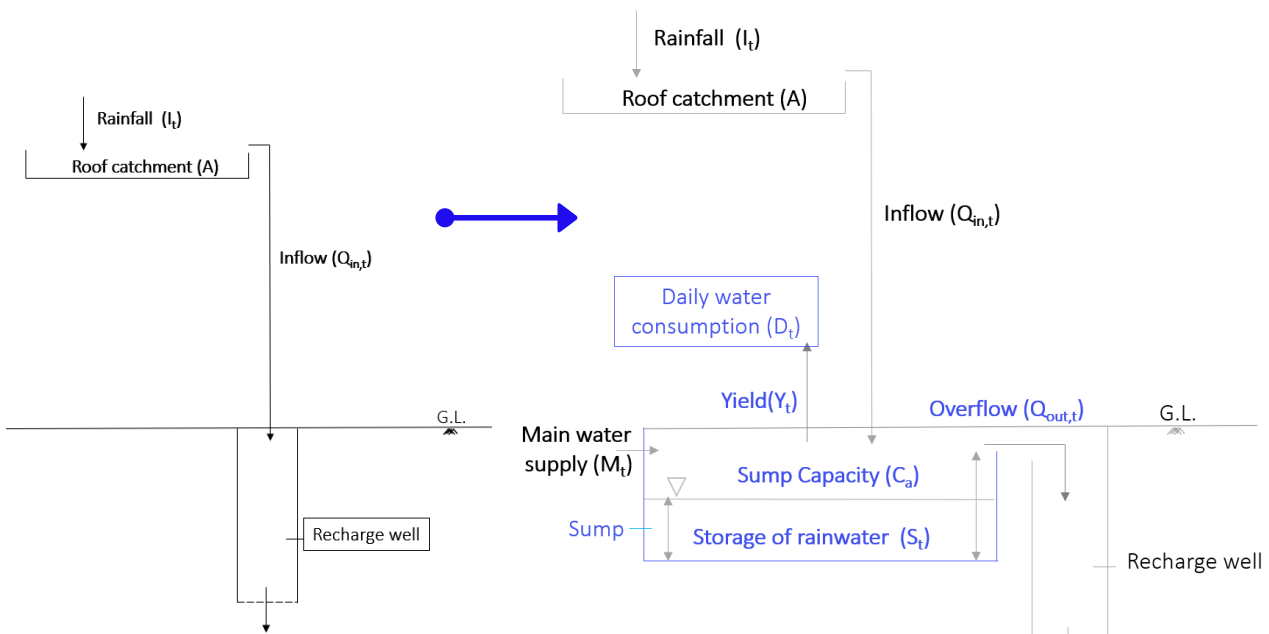
Figure 9. Scheme of RRWH in Chennai for groundwater recharge (open system)
