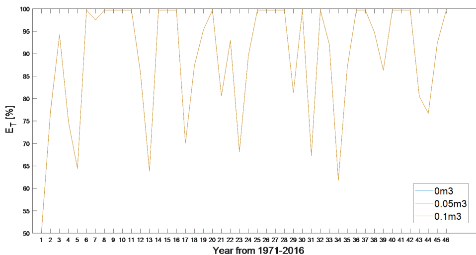
Figure 19. Effect of initial storage of year 1 on reliance for P=1 and A=33m^2
