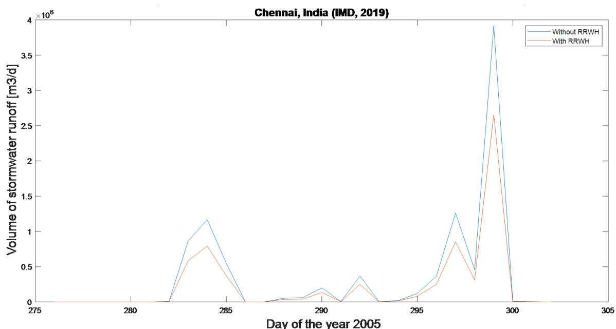
Figure 40. The effect of RRWH on stormwater peak runoff for the entire Mambalam sub-catchment for the year 2005, Chennai, India (IMD, 2019)
