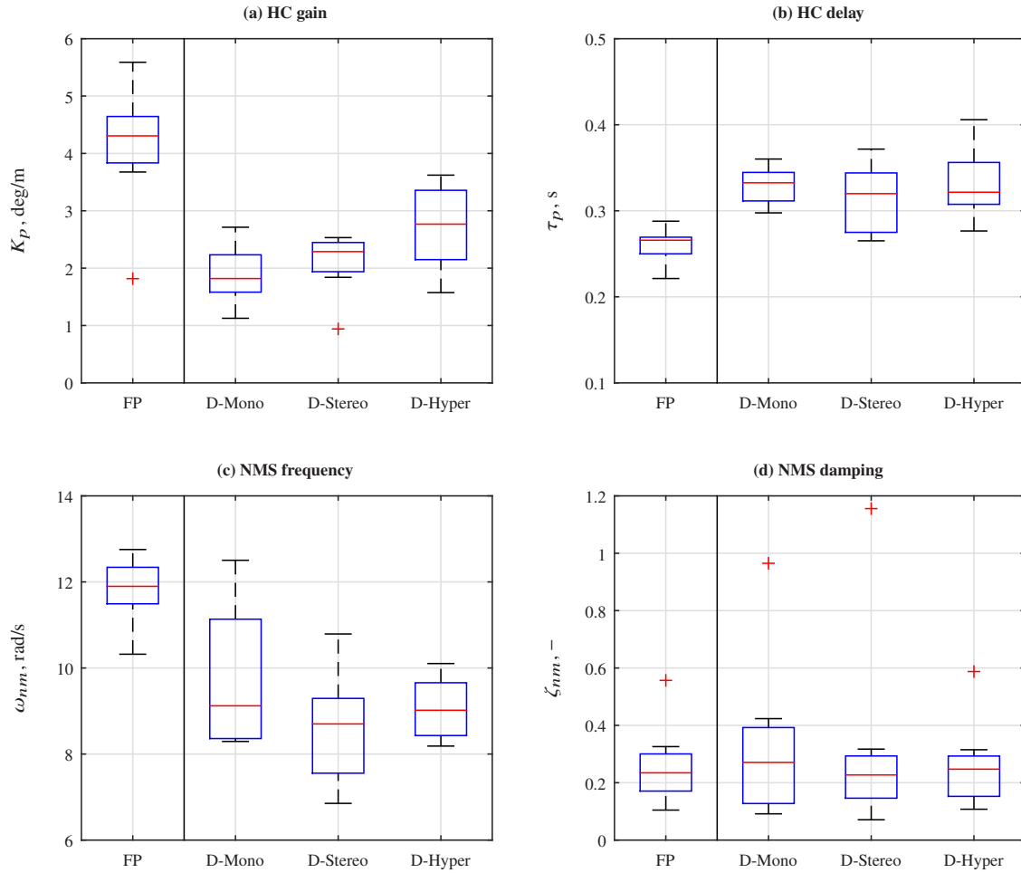
Fig. 12. Measured HC model parameters for all experiment conditions.
