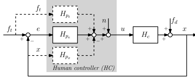
Fig. 1. A schematic representation of a pursuit tracking task.
