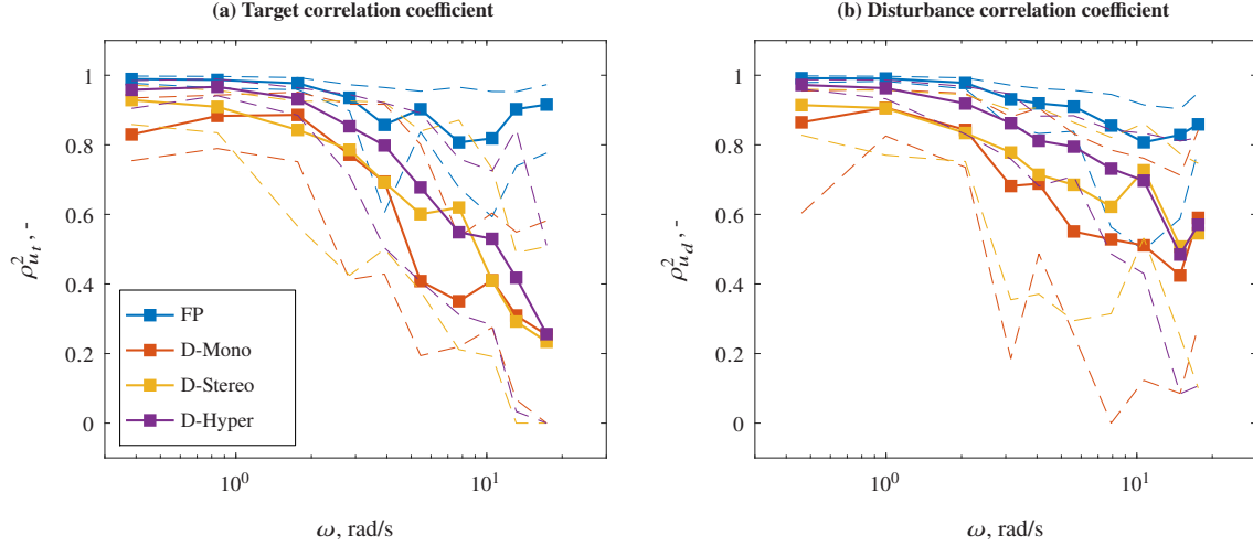
Fig. 6. Control correlation coefficient data at both the target and disturbance signal frequencies compared for all experiment conditions. Dashed lines of color that matches the mean condition data indicate the minimum and maximum \rho_{u_{t,d}}^2 measured at each frequency.
