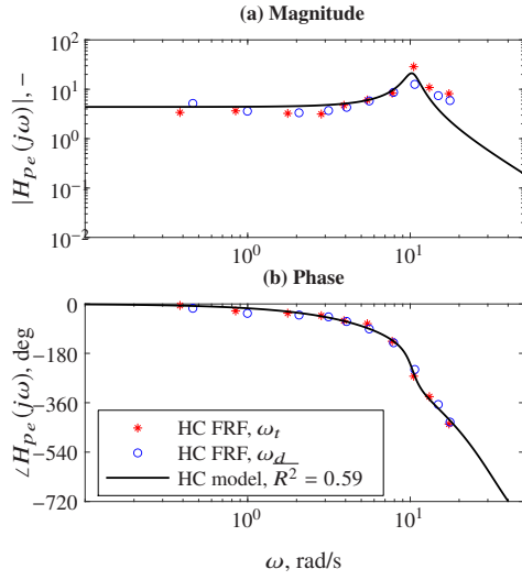
Fig. 7. HC FRFs and fitted model (Subject 1, condition FP).
