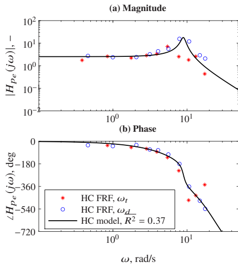
Fig. 9. HC FRFs and fitted model (Subject 1, condition D-Stereo).
