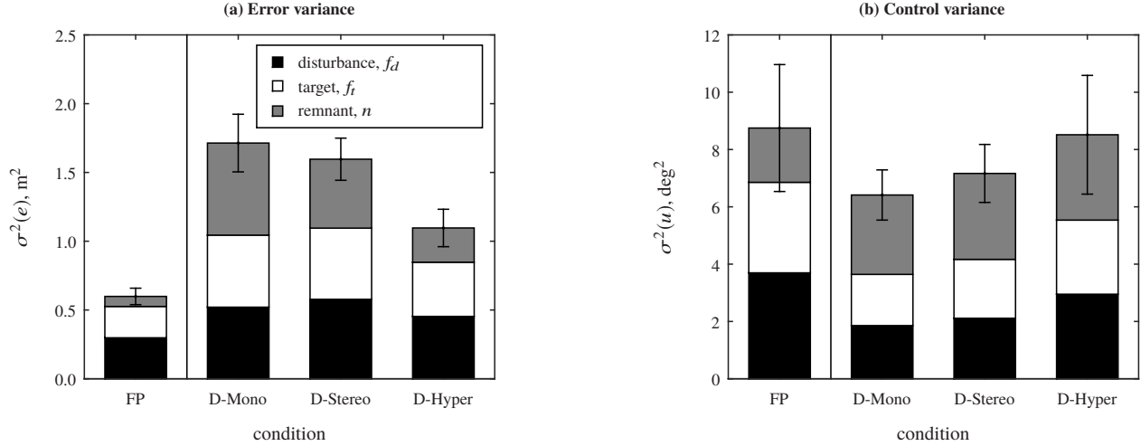
Fig. 5. Measured task performance (error signal variance) and control effort (control signal variance) for all conditions.
