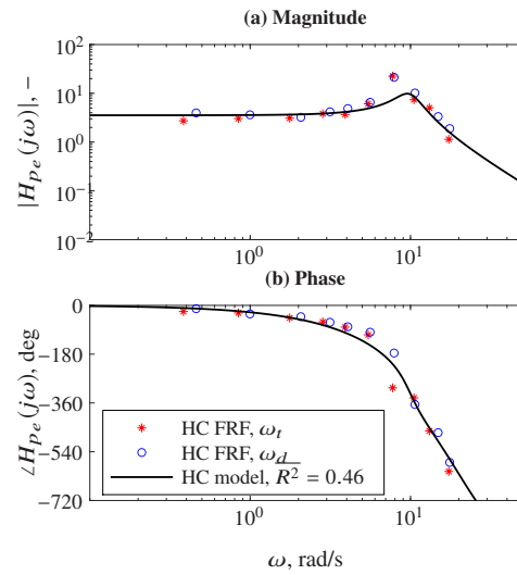
Fig. 10. HC FRFs and fitted model (Subject 1, condition D-Hyper).
