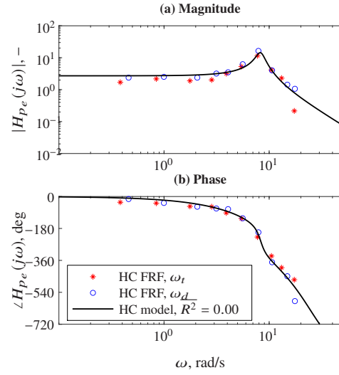
Fig. 8. HC FRFs and fitted model (Subject 1, condition D-Mono).
