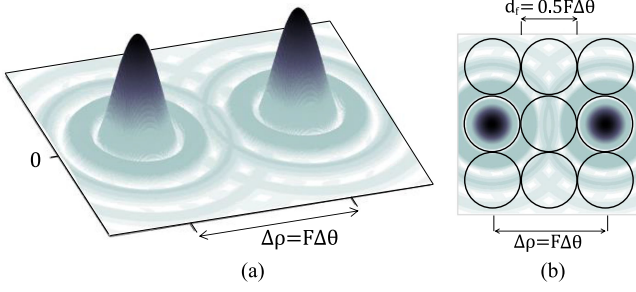
Fig. 4. (a) Diffracted field in the focal plane due to two point-sources separated by \Delta\theta . The focal plane image is a summation of two Airy discs which are separated by \Delta\rho = F\Delta\theta . (b) In order to resolve the sources in the focal plane, the feeds should be sampled with d_f = 0.5F\Delta\theta .
