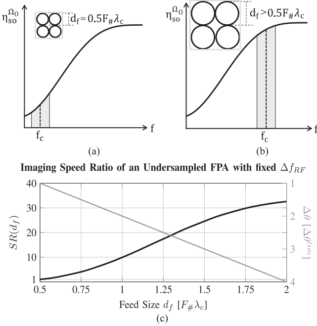
Fig. 8. The effect on imaging speed when using an undersampled array is studied w.r.t. a fully sampled array. The reference case, with imaging speed s^\beta(d_f = 0.5F_{\#}\lambda_c) , is shown in (a) and is a fully sampled FPA with \Delta\theta^{\text{lim}} = \lambda_c/D resolution. The reference case is compared to s^\alpha(d_f) as shown in (b), where the feed size is increased, leading to an undersampled array. In (c) the imaging speed ratio SR(d_f) = \frac{s^\alpha(d_f)}{s^\beta(d_f = 0.5F_{\#}\lambda_c)} and resolution are shown as a function of the feed size d_f .
