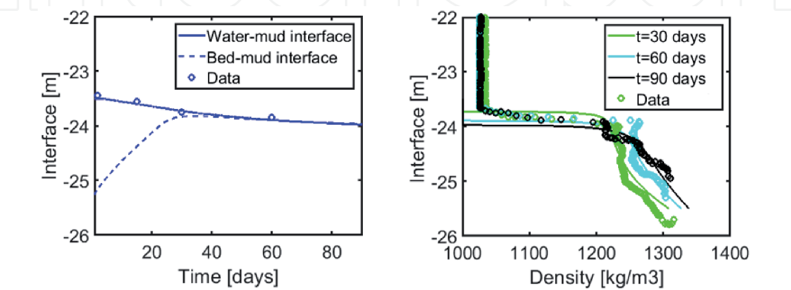
Figure 16. Estimating consolidation of fluidized mud layer after WID. Left panel shows development of water – fluidized mud interface as well as fluidized mud – Consolidated bed interface. Right panel show model predictions (solid lines) and in-situ measurements (symbols) of densities in water-mud vertical column.
