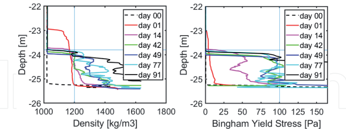
Figure 14. Density and yield stress profiles measured by Rheotune.
