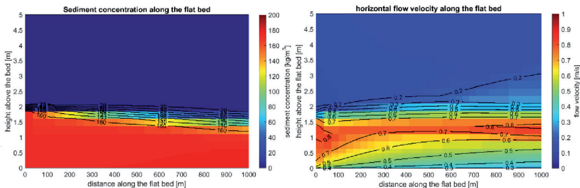
Figure 4. 1DV results for initial WID plume height of 2 m.
