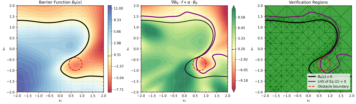
Figure 10: Barrier 2: Illustration of the barrier function B_\theta(x) , the CBF invariance condition, and the resulting verification regions after adaptive mesh refinement.
