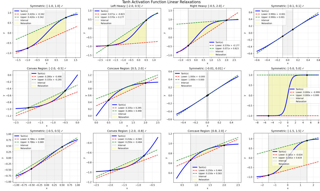
Figure 6: Tanh Relaxation.
