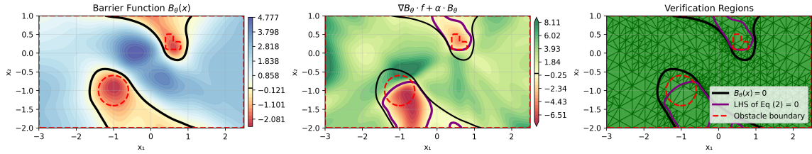
Figure 11: Barrier 3: Illustration of the barrier function B_\theta(x) , the CBF invariance condition, and the resulting verification regions after adaptive mesh refinement.
