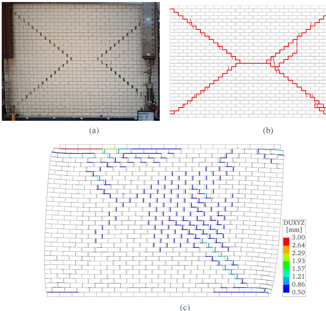
Fig. 13. (a) Wall TUD-COMP-4 at the end of the test, (b) crack pattern observed at the end of test TUD-COMP-4, and (c) deformed shape and absolute values of the relative displacements of the interfaces of TUD-COMP-4 for the maximum top displacement of 5.5 mm (scaling factor = 40).
