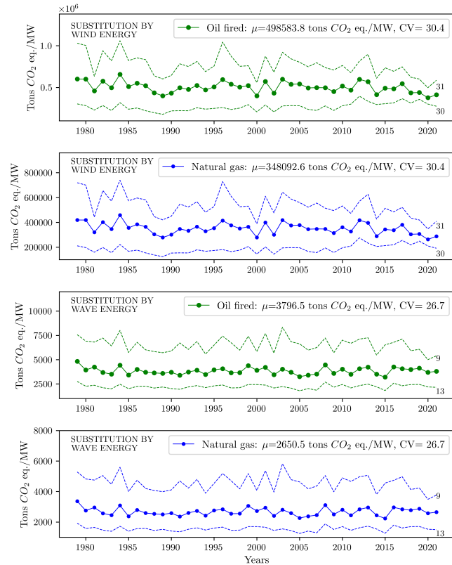
Fig. 9. Avoided CO_2 emissions by equivalent wind offshore and wave energy. Dashed lines correspond to the locations (written at the end of the trend) representing the maximum and minimum yearly values, whereas the solid line corresponds to the yearly mean value of the 36 locations.
