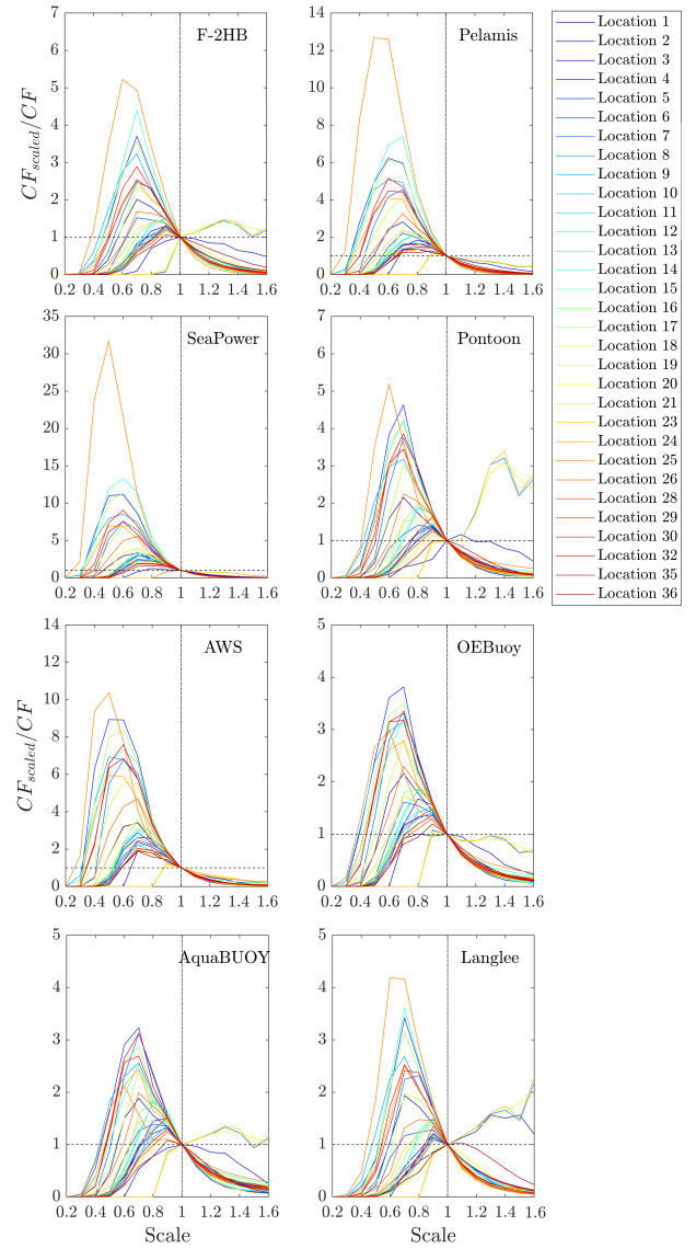
Fig. 5. CF scaled device over the CF of prototype device.
