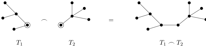
Figure 3. An example of the operation T_1 \frown T_2 .
