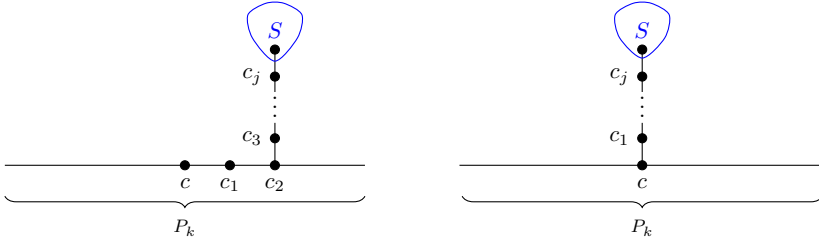
Figure 6. Potential elements of \mathcal{F} along with their ‘moving centres’.
