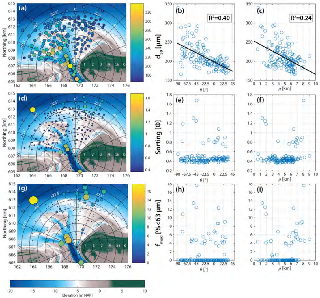
Figure 2.7: (a-c) Overview of the median grain size ( d_{50} ), (d-f) sediment sorting and (g-i) fraction of mud in the bed ( f_{mud} , defined as sediment with d_{50} < 63\mu m ). The right two columns indicate relation of the sediment parameter with clockwise direction relative to north ( \theta ) and distance from inlet ( \rho ). Modified from Elias et al. (2022) .
