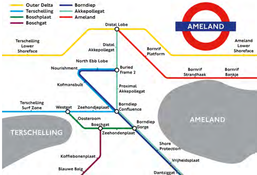
Figure 9.2: Subway map of Ameland ebb-tidal delta circa 2017. Subway lines correspond to major transport pathways as identified in this dissertation (Figure 9.1). In this way, we can depict complex information in a form more familiar to the general public.
