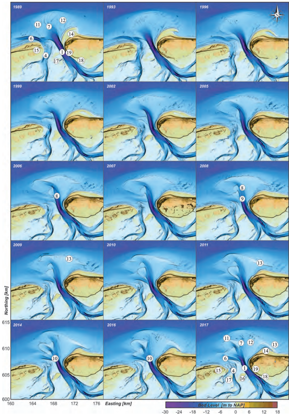
Figure 2.5: Complete digital elevation models of the ebb-tidal delta based on measurements from 1989-2017. Numbers corresponding to major channels and shoals are indicated in Figure 2.4. Source: Elias et al. (2019) .
