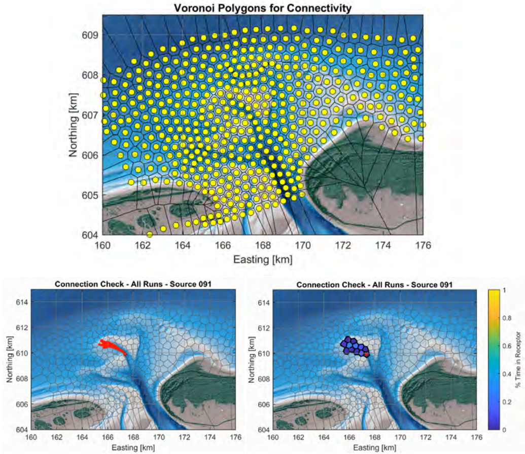
Figure 8.2: (a) Source locations for all particles, as determined via k -means cluster analysis of the bathymetry. Voronoi polygons are then drawn around each source to derive the receptor polygons. (b) Example of particle positions computed by SedTRAILS for Source 091. Particles originate at the large red and black circle, then travel in a northwesterly direction to the outer lobe of the ebb-tidal delta, passing through several geomorphic cells on its way. (c) Example of tabulated connectivity between Source 091 and its receptors. The number of particles t_{r,j} in each receptor cell j is counted and divided by the total number of particles t_{total} under consideration. Since a single particle is released at the start of the simulation and its position stored at each timestep, the colour of each receptor cell thus corresponds to the percentage of a given particle's total lifespan spent in each cell. For example, if a particle spends 25 out of 500 timesteps in a cell, that receptor cell will have a connectivity C_{ij} of 0.05.
