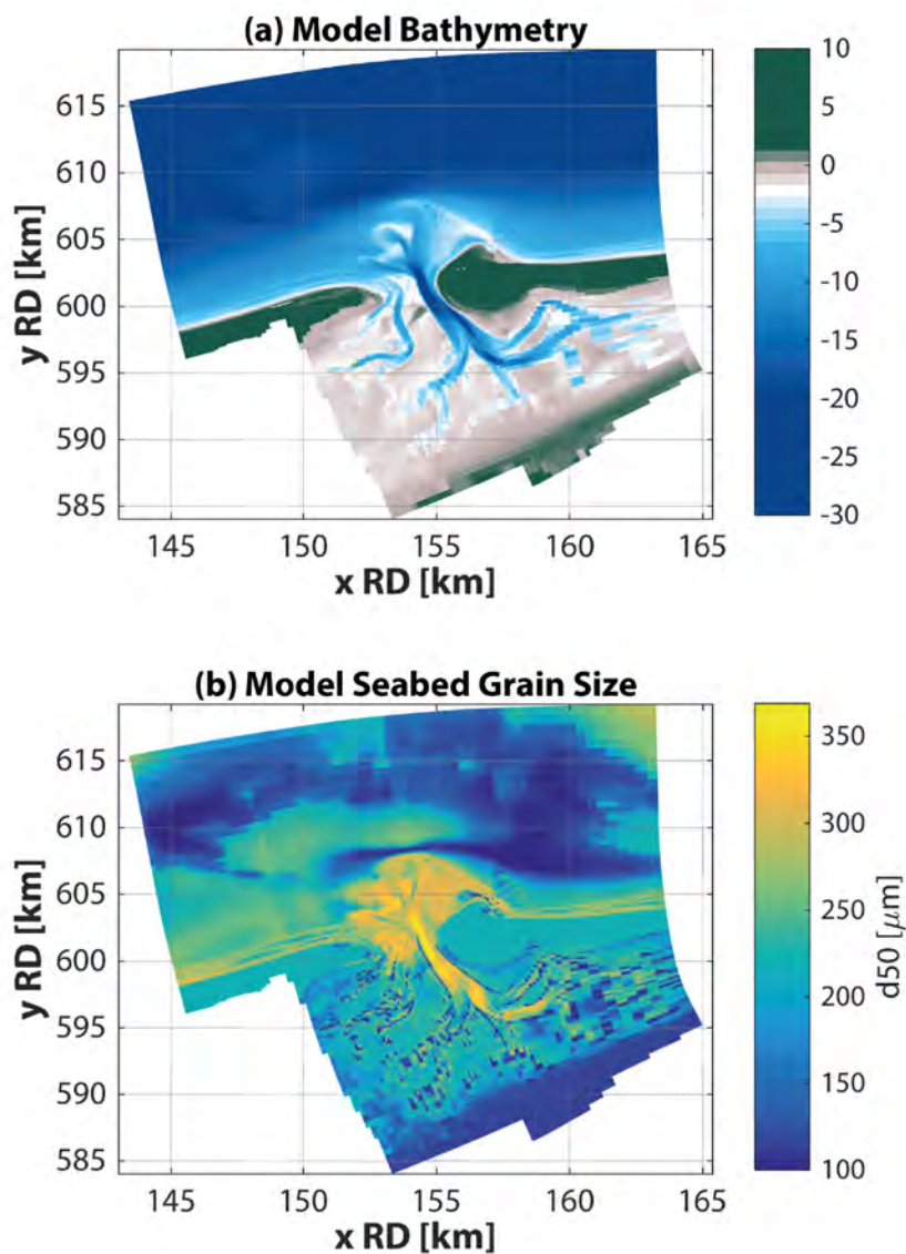
Figure 7.4: (a) Initial bathymetry of Delft3D numerical model used to calculate connectivity, based on Rijkswaterstaat (2016) . The maximum resolution of the grid is approximately 80 m at the inlet. (b) Initial sediment distribution in Delft3D model. Median grain size ( d_{50} [ \mu\text{m} ]). The coarsest sediment can be found in the deepest parts of the channel where tidal currents are strongest, whereas the finest sediment is located offshore, on intertidal flats inside the basin, and seaward of the ebb-tidal shoals. Coordinates are given in Amersfoort/RD New system.
