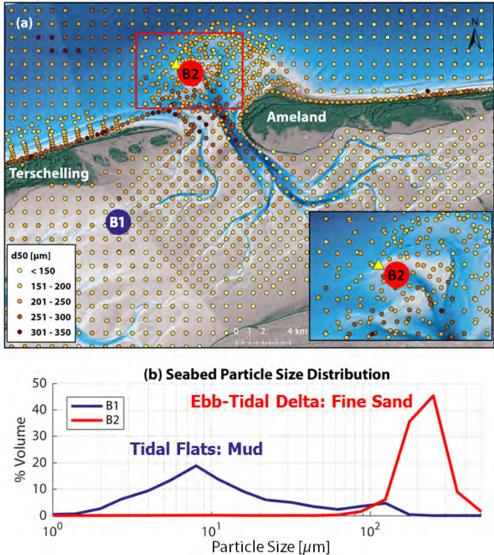
Figure 4.3: (a) Median bed sediment grain size ( d_{50} ). Ebb-tidal delta sediment was obtained from box cores for this study, and basin/offshore areas were obtained from the Wadden Sea Sediment Atlas ( Rijkswaterstaat, 1999 ). The yellow triangle indicates the measurement frame. (b) Particle size distribution in the bed at key locations.
