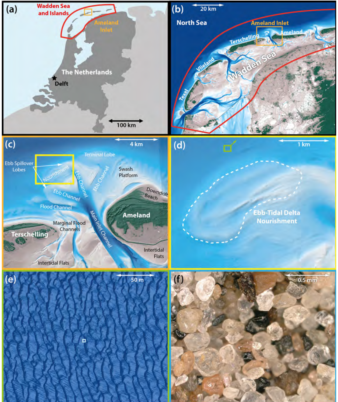
Figure 1.2: Overview of the study site at different spatial scales. (a) Overview map of the Netherlands indicating the location of the Wadden Sea and main study site at Ameland Inlet ( \mathcal{O}(100 - 1000\text{km}) ). (b) The Dutch Wadden Sea ( \mathcal{O}(10 - 100\text{km}) ). (c) Ameland inlet and ebb-tidal delta circa 2021 ( \mathcal{O}(1 - 10\text{km}) ). (d) Nourishment on Ameland ebb-tidal delta ( \mathcal{O}(100 - 1000\text{m}) ). (e) Bedforms on the seabed located just offshore of the ebb-tidal delta ( \mathcal{O}(0.01 - 100\text{m}) ). (f) Individual grains of sand on the ebb-tidal delta ( \mathcal{O}(0.01 - 1\text{mm}) ).
