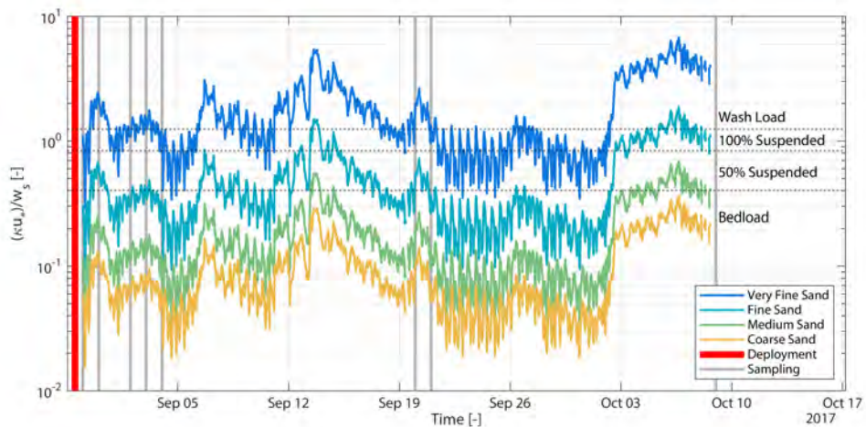
Figure 6.10: Inverse Rouse number ( \kappa u_* / w_s ) and transport mode for each sediment class. Calculated using the method of Soulsby (1997) from wave and near-bed velocity measurements taken by a downward-facing ADCP-HR near the tracer source (mounted 0.5m above the seabed). Tracer sampling dates are indicated by grey bars.
