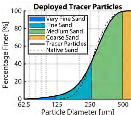
Figure 6.4: Particle size distribution of deployed tracer sediment and native seabed sediment (from available pre-study data (Rijkswaterstaat, 1999)). Deployed tracer and native sediment largely consist of fine (125-250 \mu\text{m} ) and medium (250-500 \mu\text{m} ) sand.
