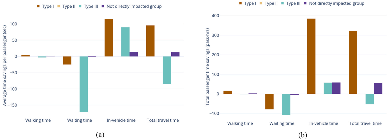
Fig. 6. Effect of skip-stop operation on (a) average time savings per passenger in seconds; (b) total passenger time savings in passenger-hours; for the southbound direction of metro line 19 under increased demand (180 %).
